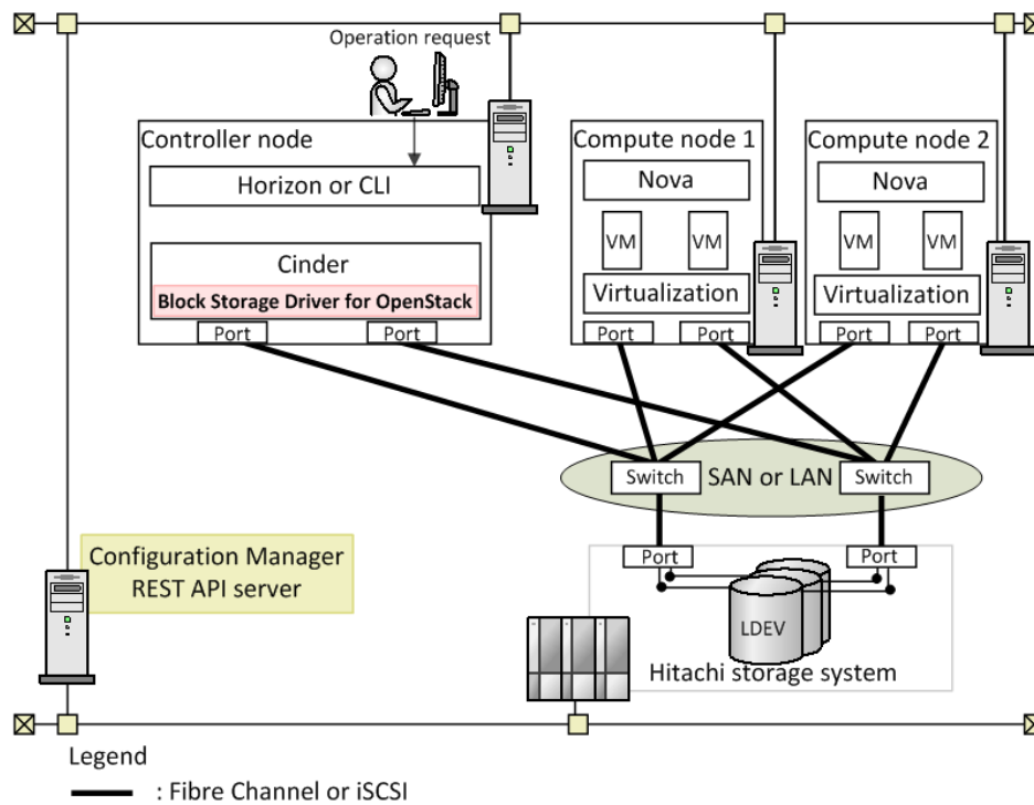
Figure 4 Connection example of node configuration
