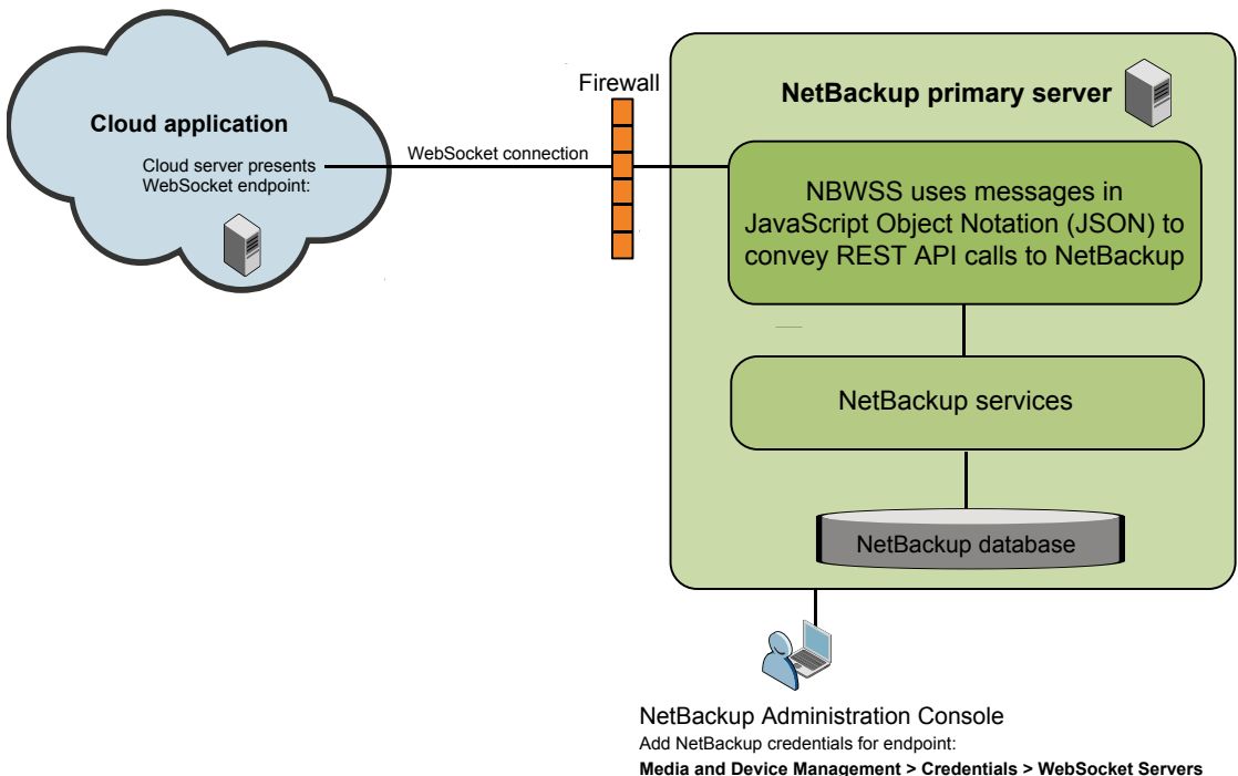
Figure 1-1 NBWSS overview
