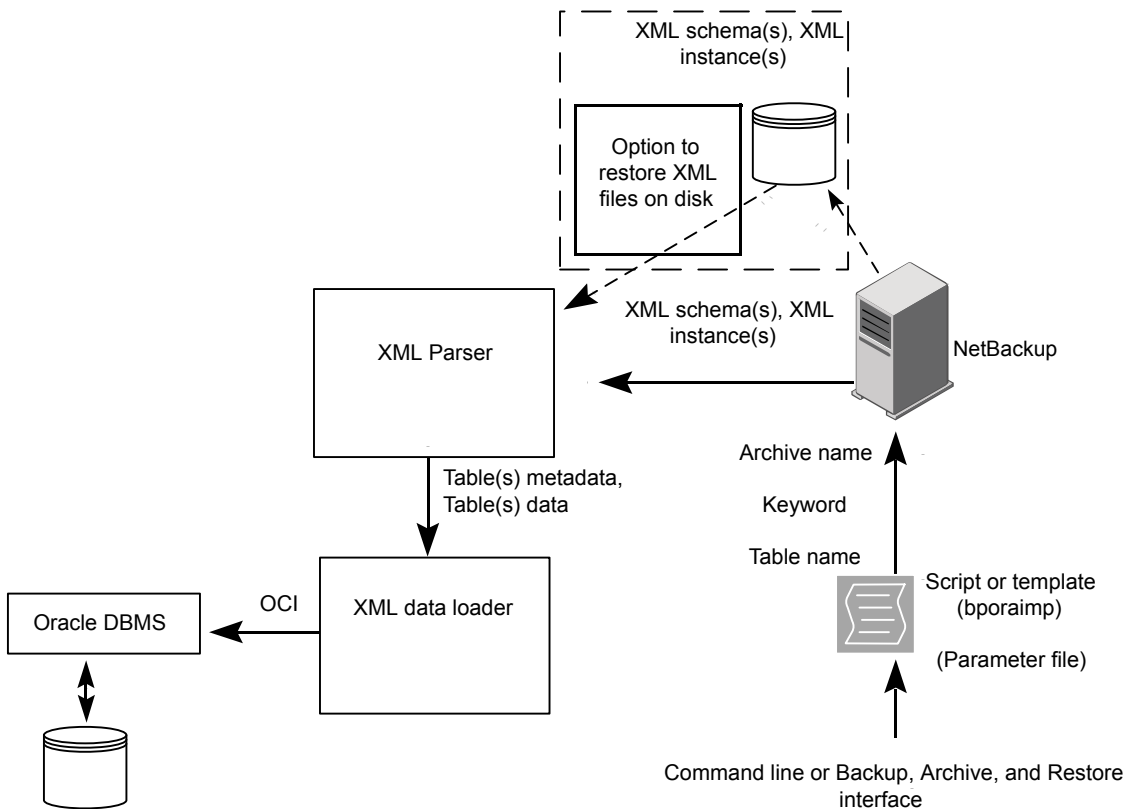
Figure D-4 XML import restore data flow
