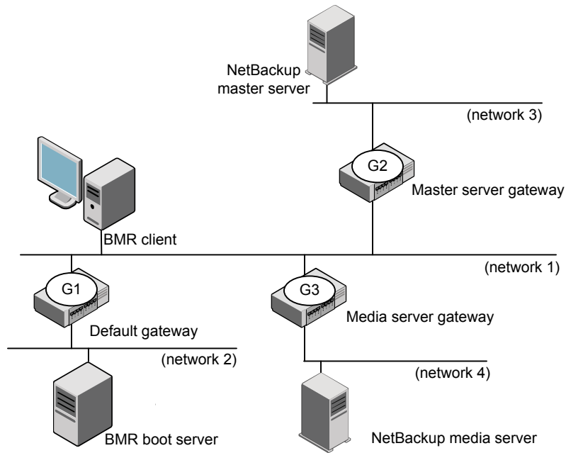
Figure 6-5 Gateway example
