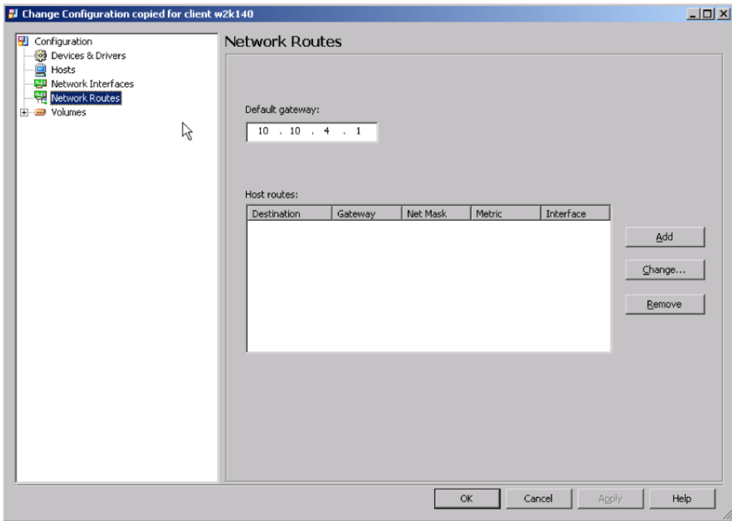
Figure 8-6 Network routes property sheet
