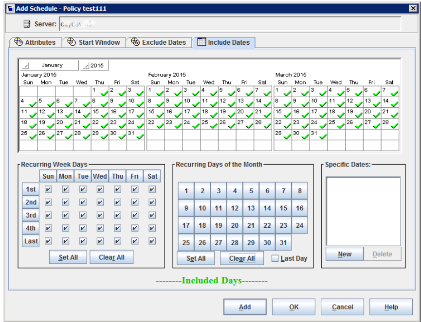
Figure 21-20 An open schedule that is calendar-based
