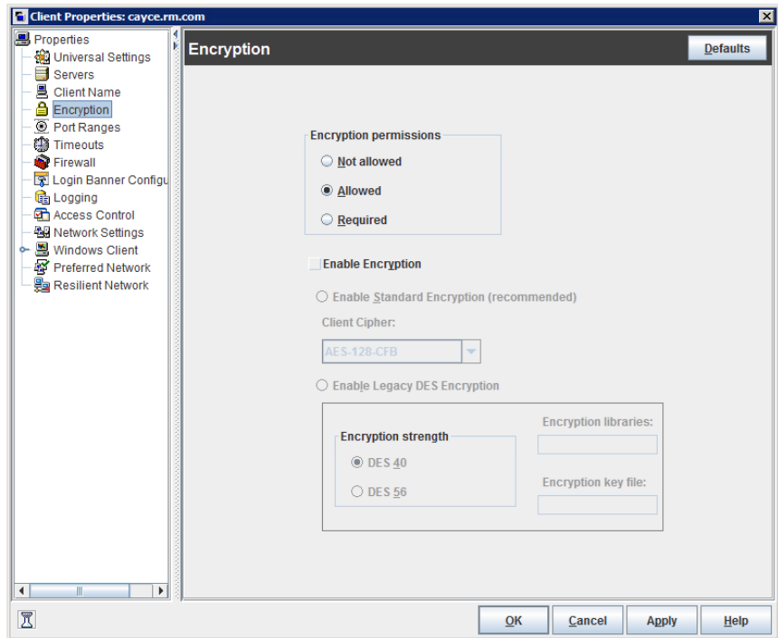
Figure 3-15 Encryption dialog box
