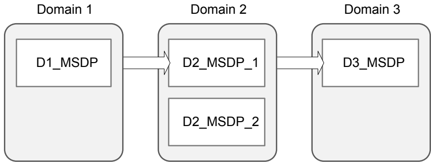
Figure 28-13 Example storage lifecycle policy topology
