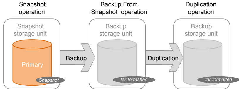
Figure 16-13 SLP that contains a Snapshot operation, a Backup From Snapshot operation, and a Duplication operation
