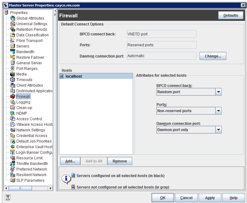
Figure 3-22 Firewall dialog box
