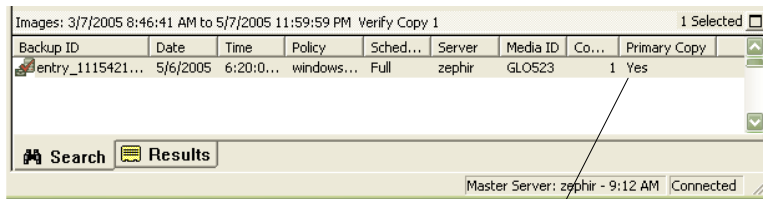
Figure 25-2 Primary copy status
