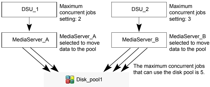
Figure 12-6 Impact when disk storage units use one disk pool but different media servers
