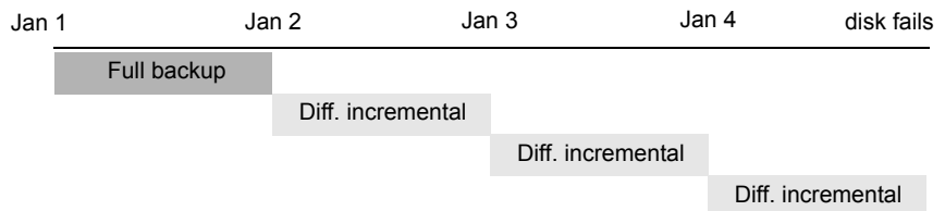
Figure 21-10 Full and differential incremental example
