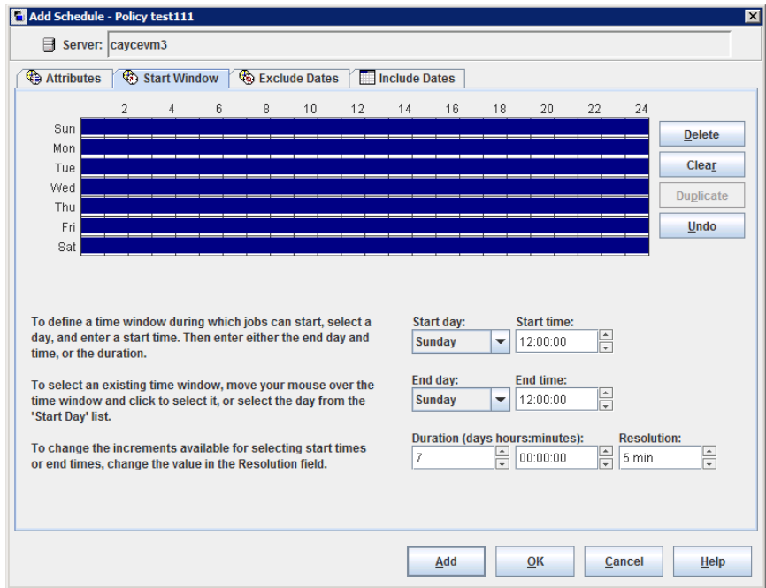
Figure 21-19 An open schedule
