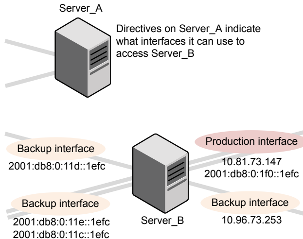
Figure 3-37 Multihomed servers example
