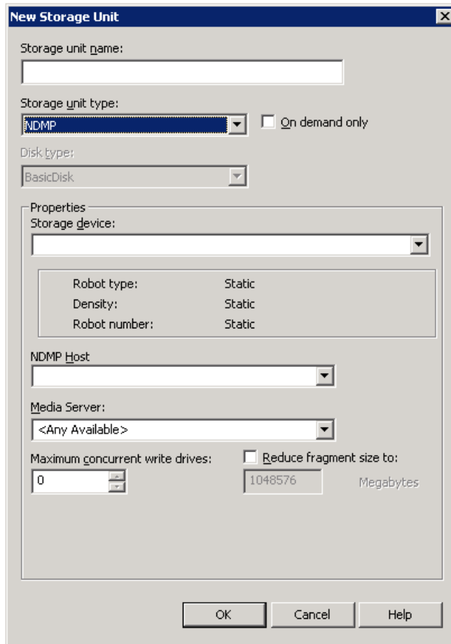
Figure 12-5 NDMP storage unit settings
