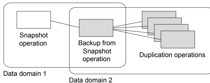
Figure 16-18 Hierarchical operations
