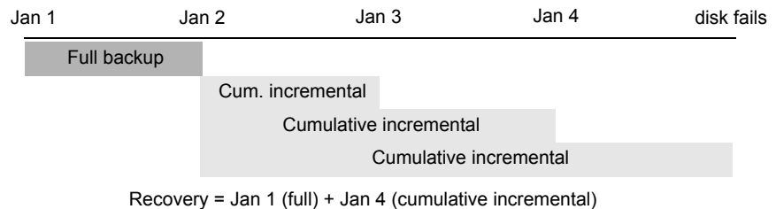
Figure 21-11 Full and cumulative incremental example
