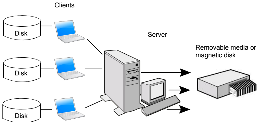
Figure 21-12 Multiplexed backups
