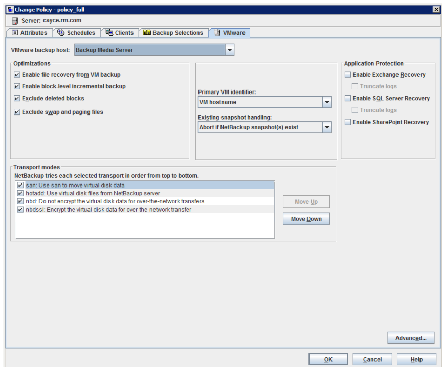
Figure 21-31 VMware tab
