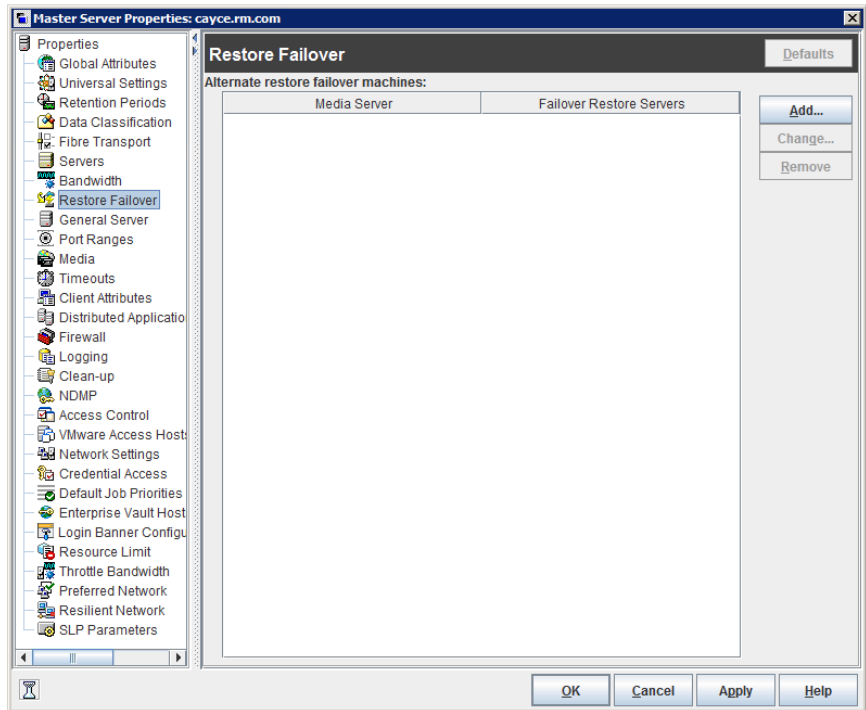
Figure 3-54 Restore Failover dialog box
