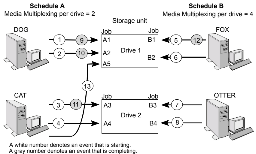
Figure 21-13 Multiplexing process scenario
