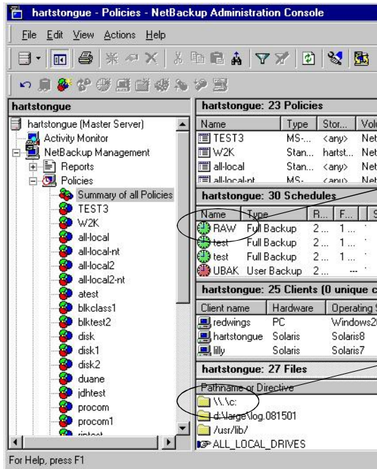
Figure 21-23 Disk image backups
