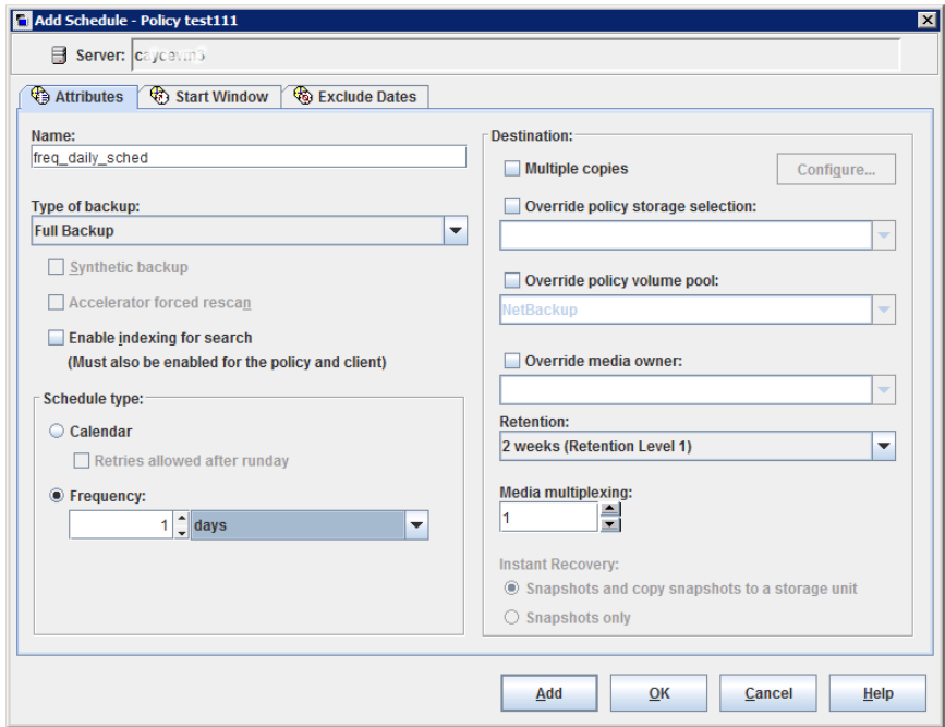
Figure 21-21 An open schedule that is frequency-based
