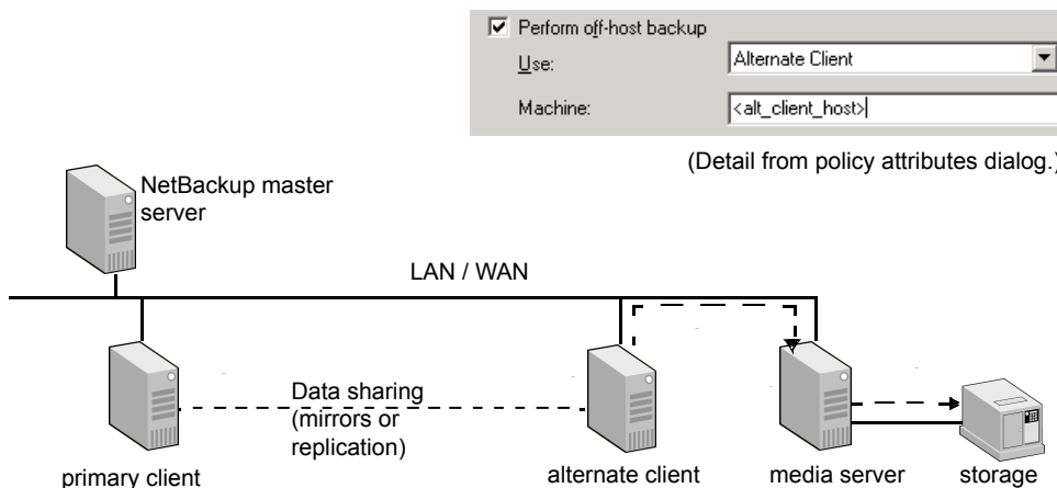
Figure 1-6 Alternate client backup: backup is performed on alternate client
