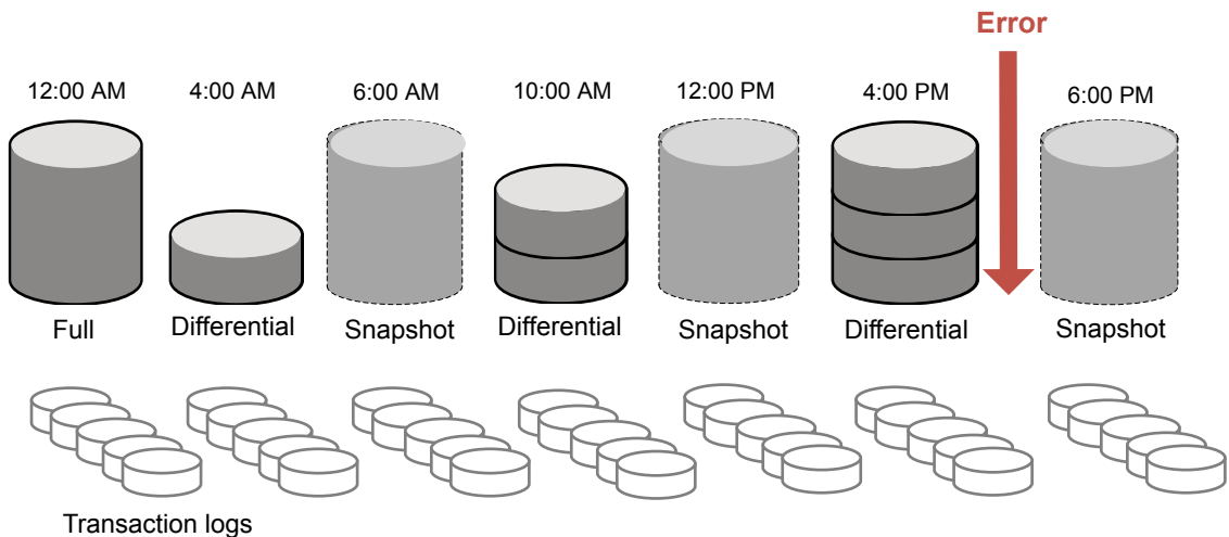
Figure 8-2 Recovering after an error when using full and copy-only backups
