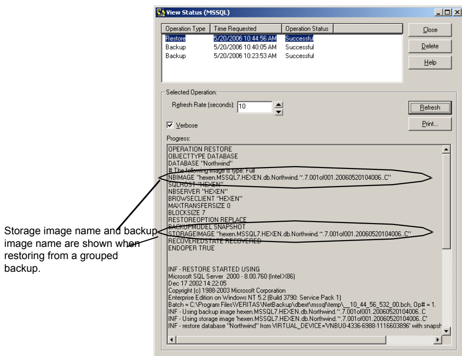
Figure 8-4 Batch file shown in the progress report for the restore operation
