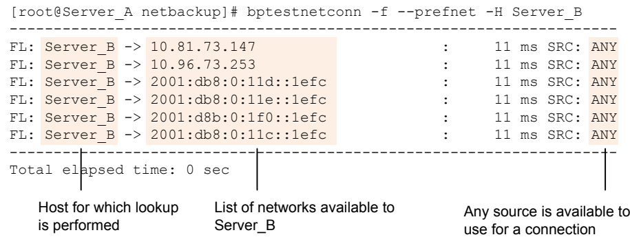
Figure 3-45 bptestnetconn for Server_B with no directives listed
