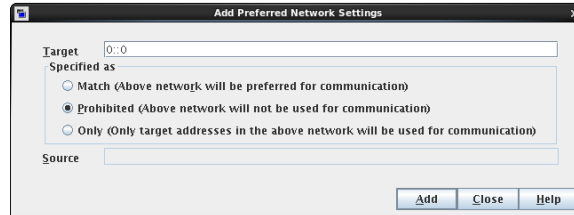
Figure 3-49 Prohibit IPv6 addresses as targets
