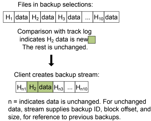
Figure 20-7 NetBackup client: Accelerator backup stream
