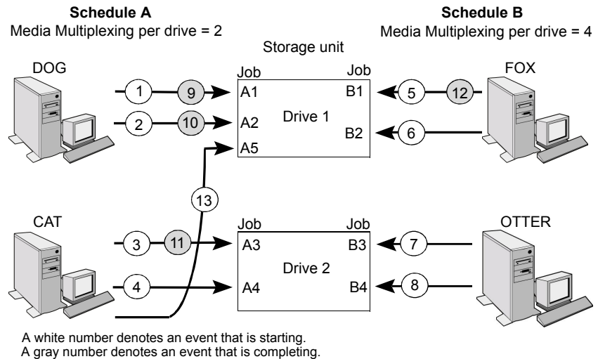
Figure 20-14 Multiplexing process scenario
