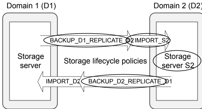
Figure 25-9 Topology after changes
