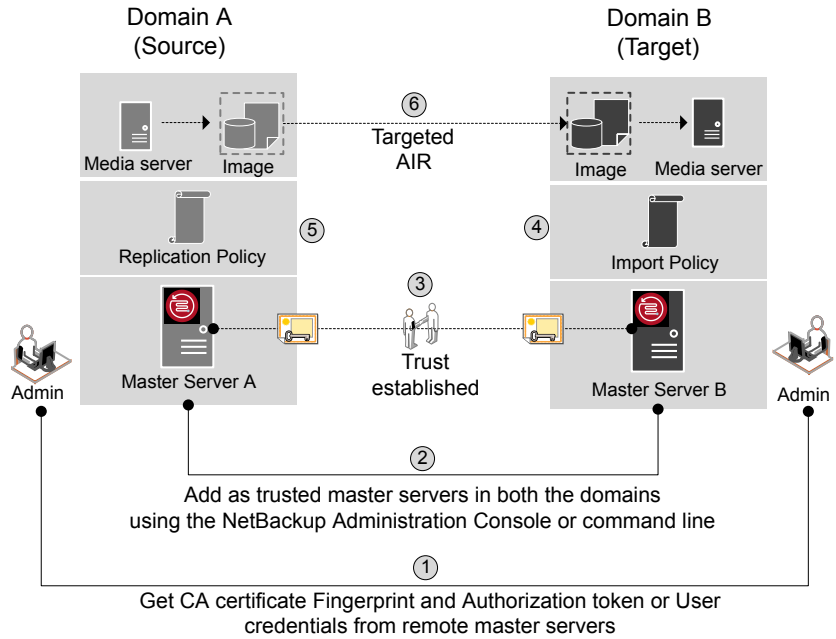
Figure 25-3 Tasks to establish a trust relationship between master servers for Targeted A.I.R.
