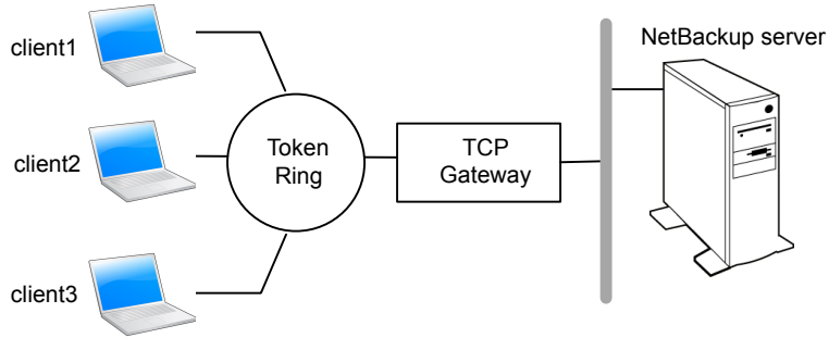
Figure 33-1 Example restore from a token ring client
