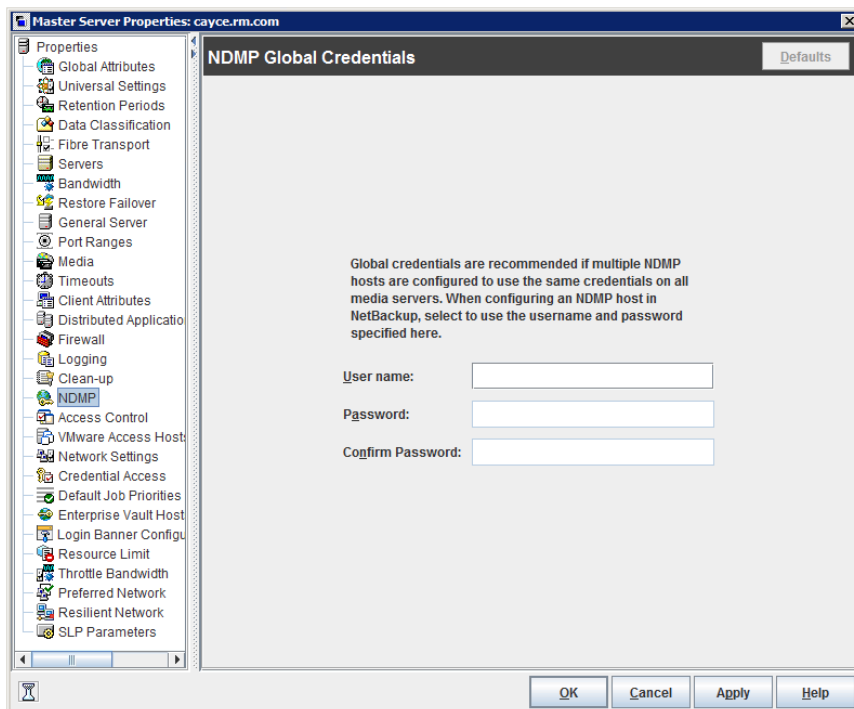
Figure 3-37 NDMP Global Credentials dialog box
