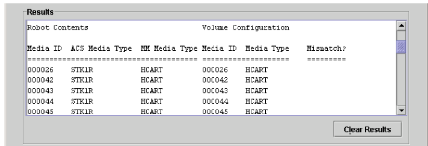
Figure 10-3 Compare contents report (API robot)
