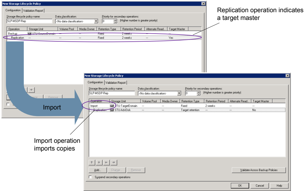
Figure 25-4 Storage lifecycle policy pair required for Auto Image Replication
