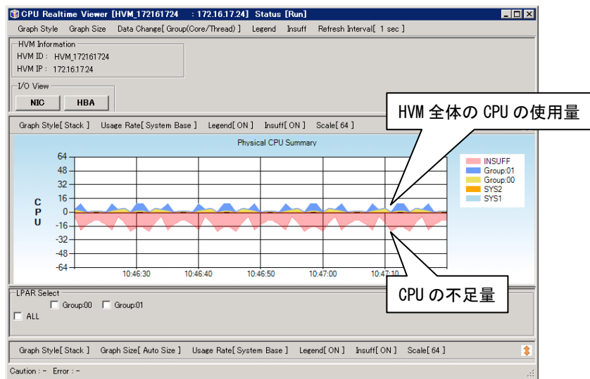
図 2-10 CPU Realtime Viewer[HVM ID : HVM IP]ウインドウ (Physical CPU Summary [Case 5])
