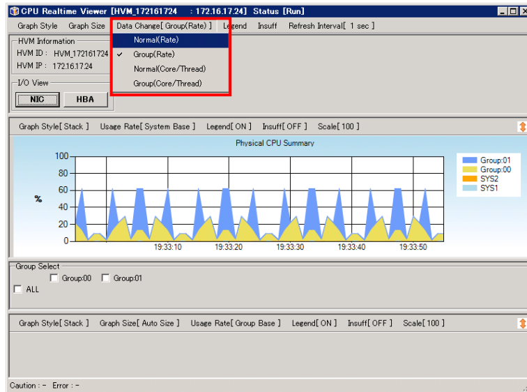
図 4-27 CPU Realtime Viewer[HVM_ID : HVM_IP]ウインドウ ([Data Change]-[Normal (Rate)])選択
