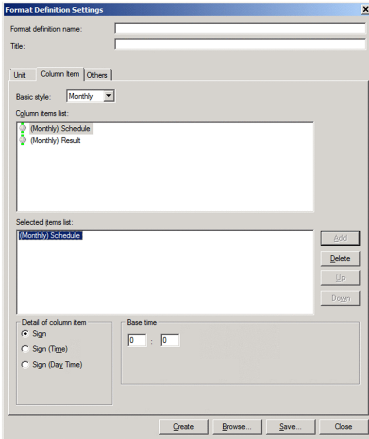
Figure 7–33: Column Item tab of Format Definition Settings window (with Monthly Schedule selected)
