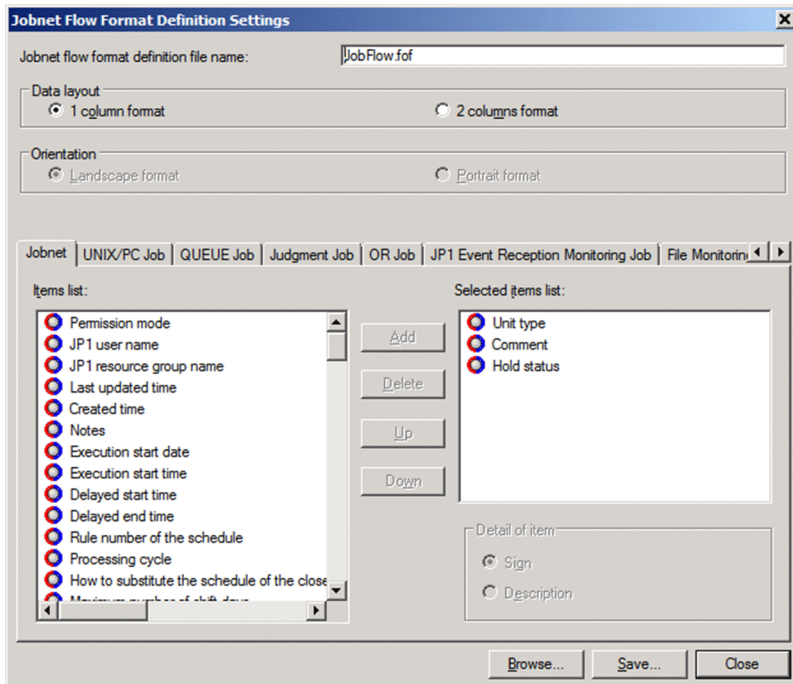
Figure 7–64: Jobnet Flow Format Definition Settings window
