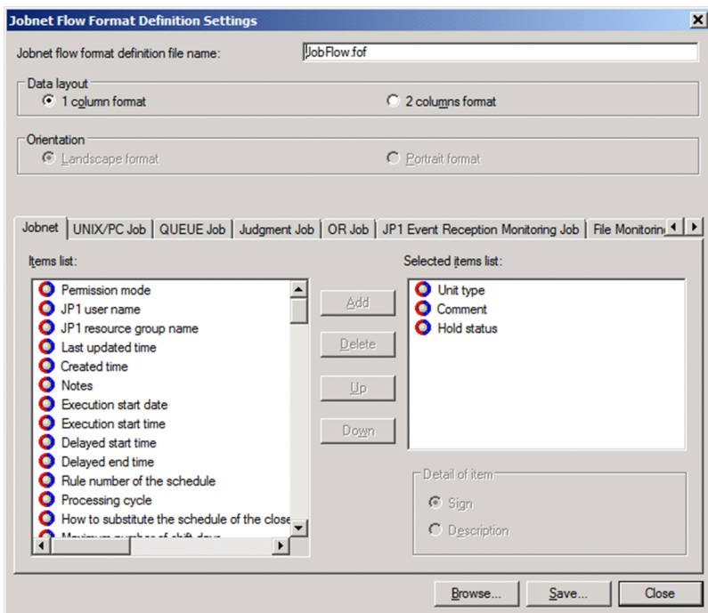
Figure 6–41: Jobnet Flow Format Definition Settings window
