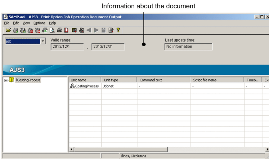
Figure 6–3: Job Operation Document Output window with file open
