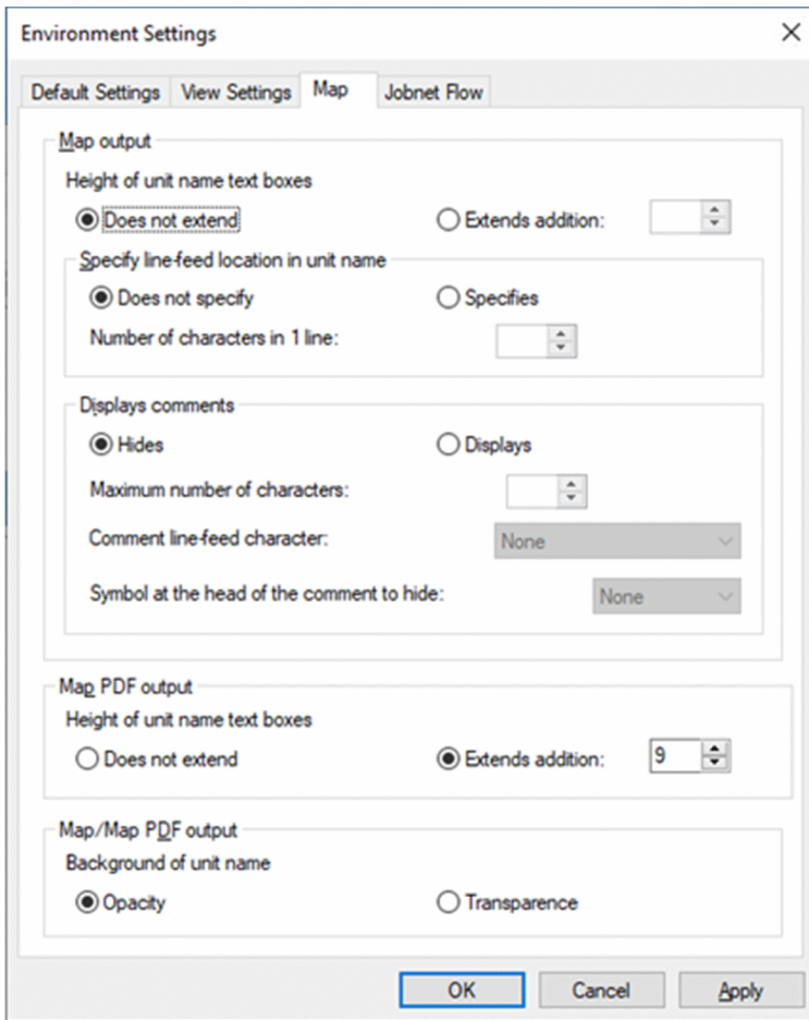
Figure 7–67: Map tab of Environment Settings window
