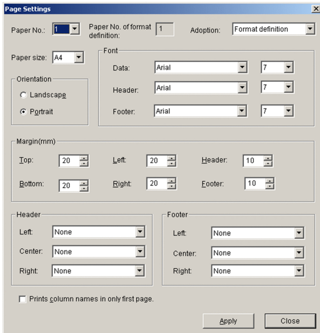
Figure 7–61: Page Settings window
