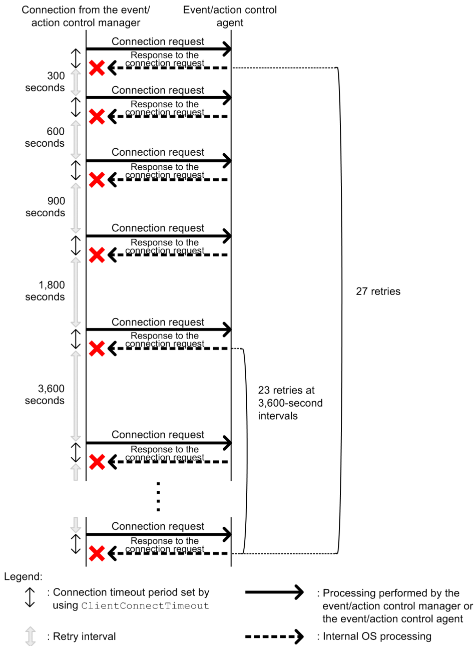
Figure 15–4: Communication from the event/action control manager to the event/action control agent when a connection timeout occurs
