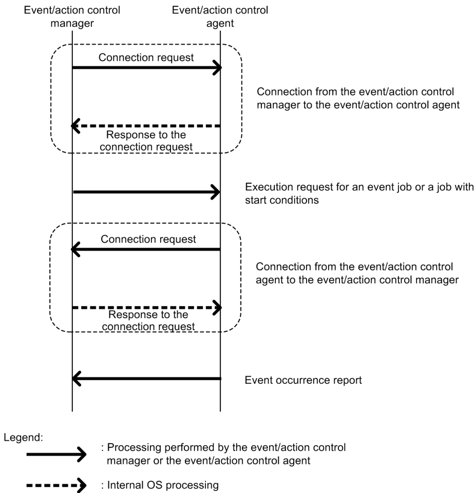
Figure 15–2: Communication when an event job, a custom event job or a jobnet with start conditions is executed
