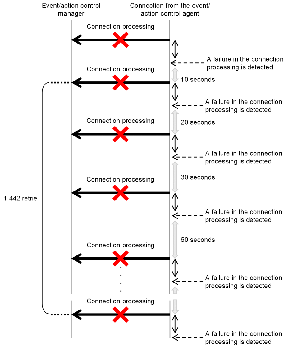
Figure 15–5: Communication from the event/action control agent to the event/action control manager when a connection error occurs
