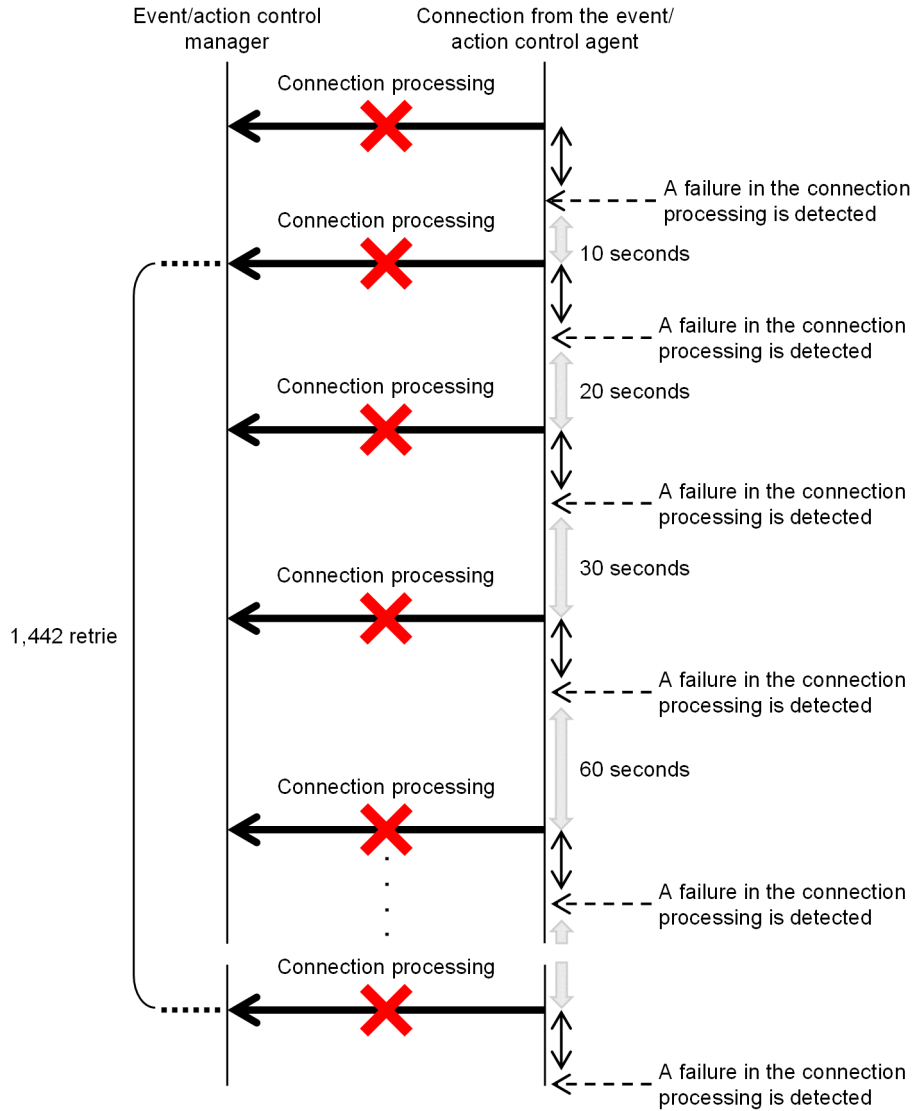
Figure 6–5: Communication from the event/action control agent to the event/action control manager when a connection error occurs
