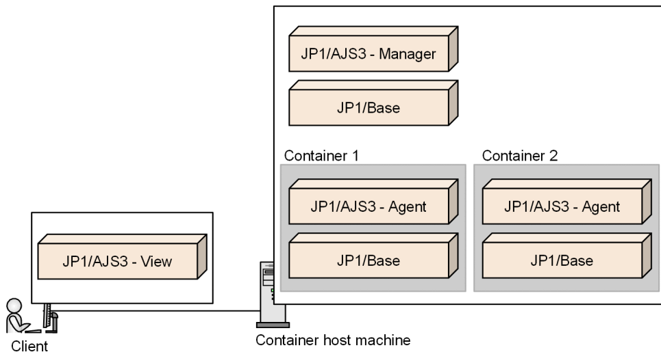
Figure 2–79: JP1/AJS3 system configuration in a container environment (1): JP1/AJS3 - Manager is installed on a container host machine and JP1/AJS3 - Agent is installed in each container
