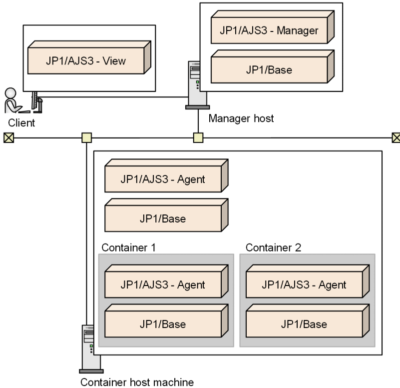
Figure 2–80: JP1/AJS3 system configuration in a container environment (2): JP1/AJS3 - Agent is installed both on a container host machine and in each container, with a manager host prepared
