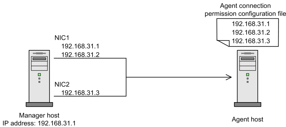
Figure 2–44: Example of restricting access in a multiple-NIC environment
