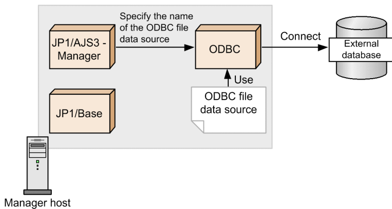
Figure 2–69: ODBC-based connection to the external database
