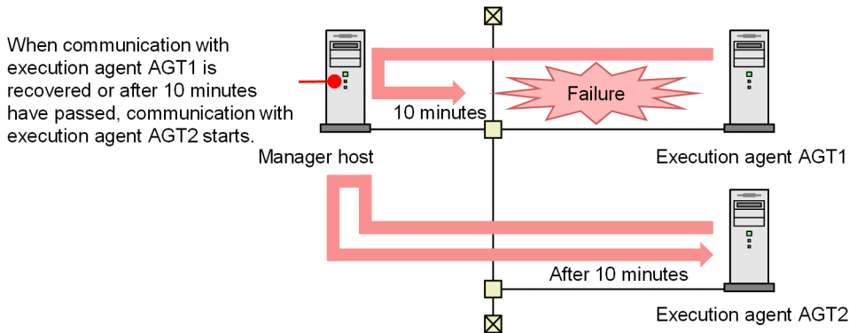
Figure 2–54: Job status transition when a communication failure occurs on an execution agent
