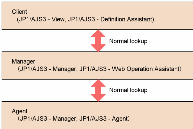
Figure 2–38: Settings required for name resolution by using normal lookup for JP1/AJS3 products
