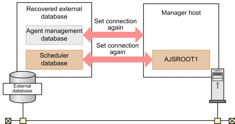
Figure 2–78: Example of setting connections again when the external database is recovered
