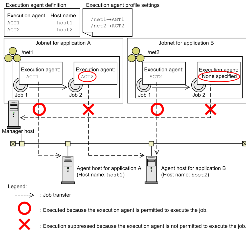
Figure 2–49: Example of using the execution agent restriction functionality
