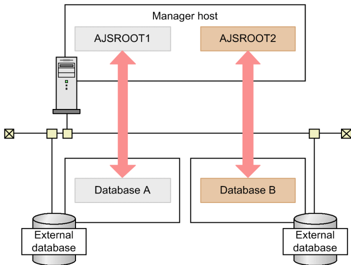
Figure 2–73: Configuration in which one manager host uses different instances of the external database
