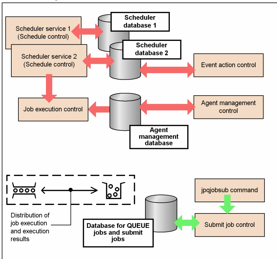
Figure 2–57: JP1/AJS3 database configuration
