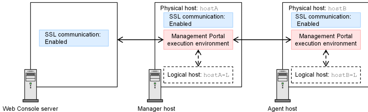
Figure 2–37: Example of communications when using the Web GUI (Management Portal)
