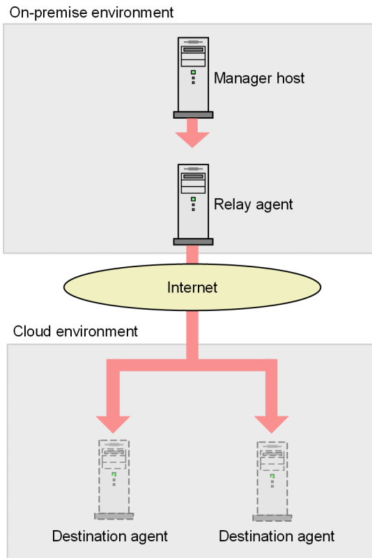
Figure 2–62: Example of combining an on-premise environment and a cloud environment 1
