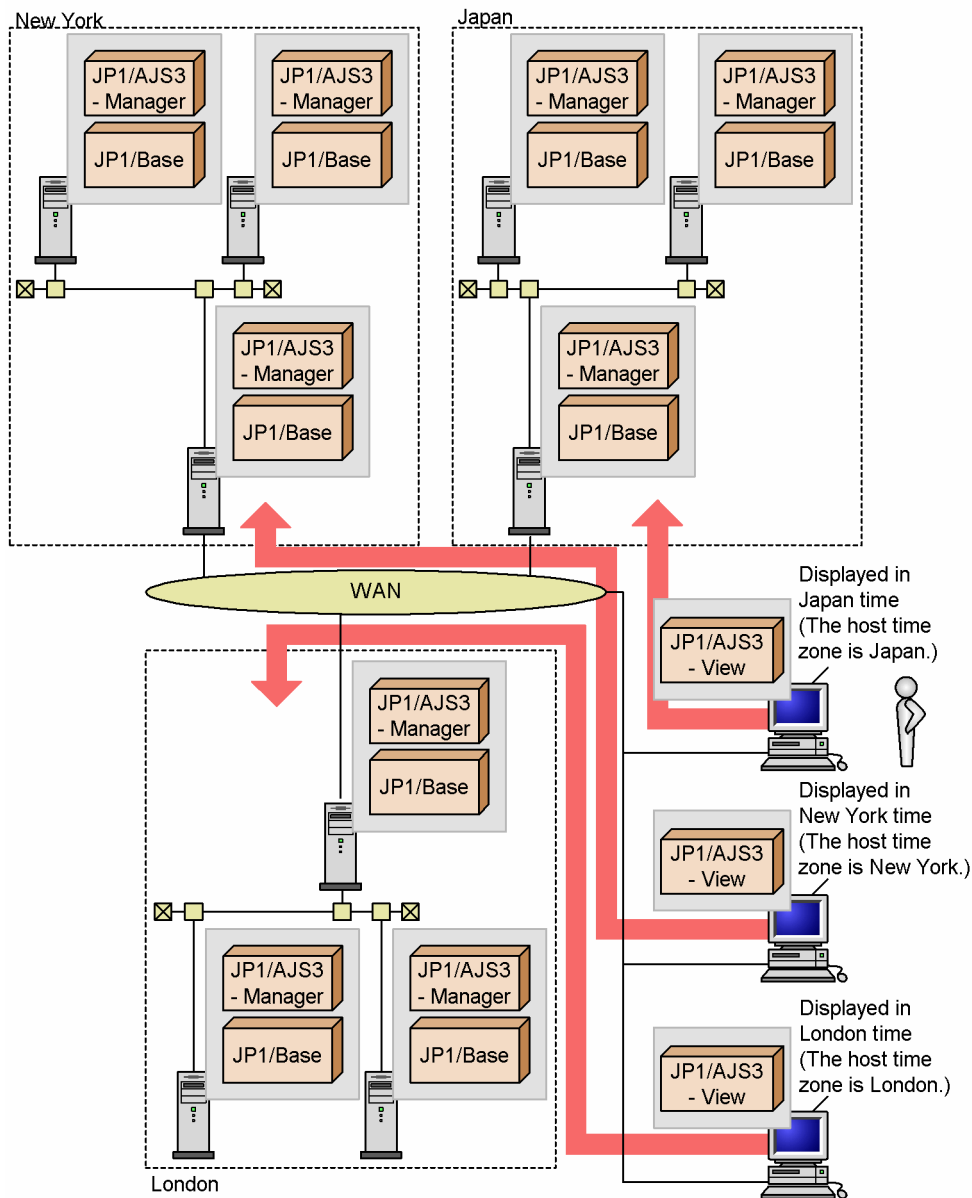
Figure 2–45: Example of a system configuration for checking jobnet execution status on manager hosts in different time zones
