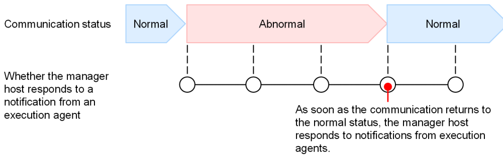
Figure 2–56: Time when the recovery of an execution agent from communication failure can be detected
