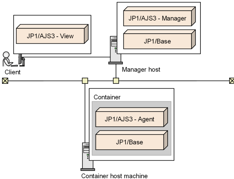
Figure 2–81: JP1/AJS3 system configuration in a container environment (3): JP1/AJS3 - Agent is installed in only each container on a container host machine, with a manager host prepared
