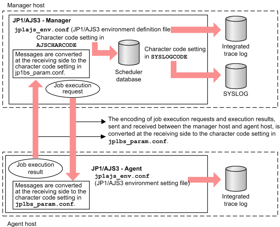
Figure 2–48: Sections affected when the character encoding is changed
