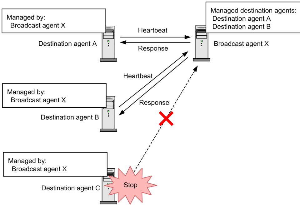
Figure 2–66: Example in which a broadcast agent manages destination agents
