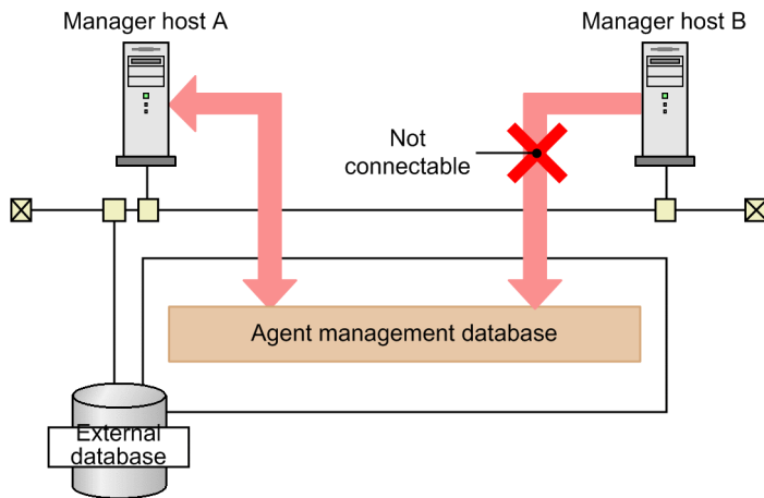
Figure 2–76: Connection relationship between the agent management database and the manager host
