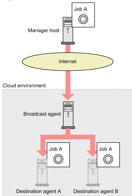
Figure 2–65: Example in which a broadcast agent distributes a job to multiple destination agents
