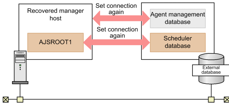
Figure 2–78: Example of setting connections again when the external database is recovered
