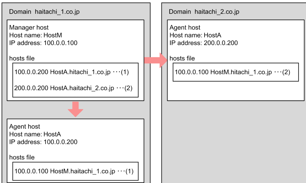
Figure 2–40: Example of operation with FQDN host names
