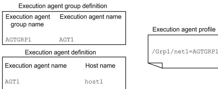
Figure 2–51: Setting an execution agent group in the execution agent profile
