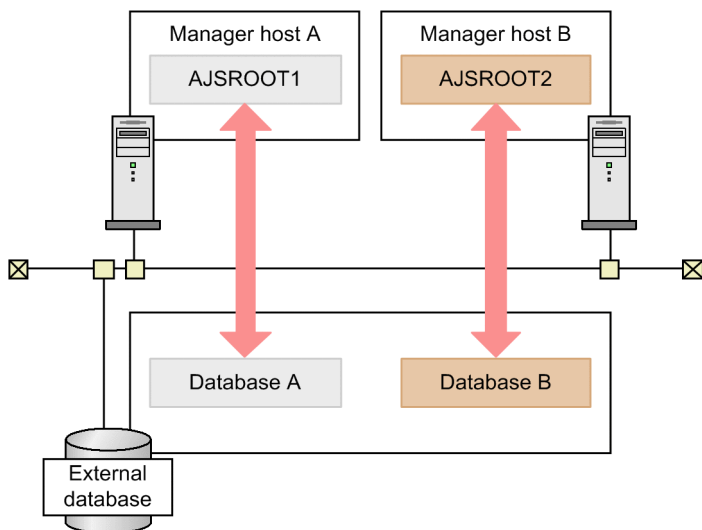
Figure 2–74: Configuration in which different manager hosts use one instance of the external database
