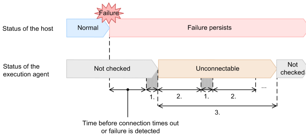
Figure 2–53: Time periods that can be set by using environment setting parameters
