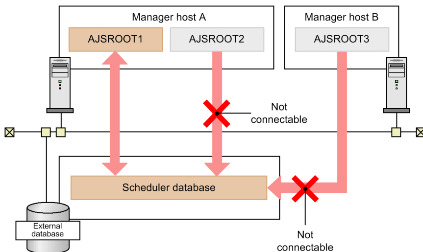
Figure 2–75: Connection relationship between the scheduler database configured with the external database and scheduler services
