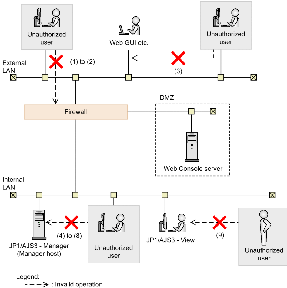
Figure 2–58: Measures preventing access by unauthorized users
