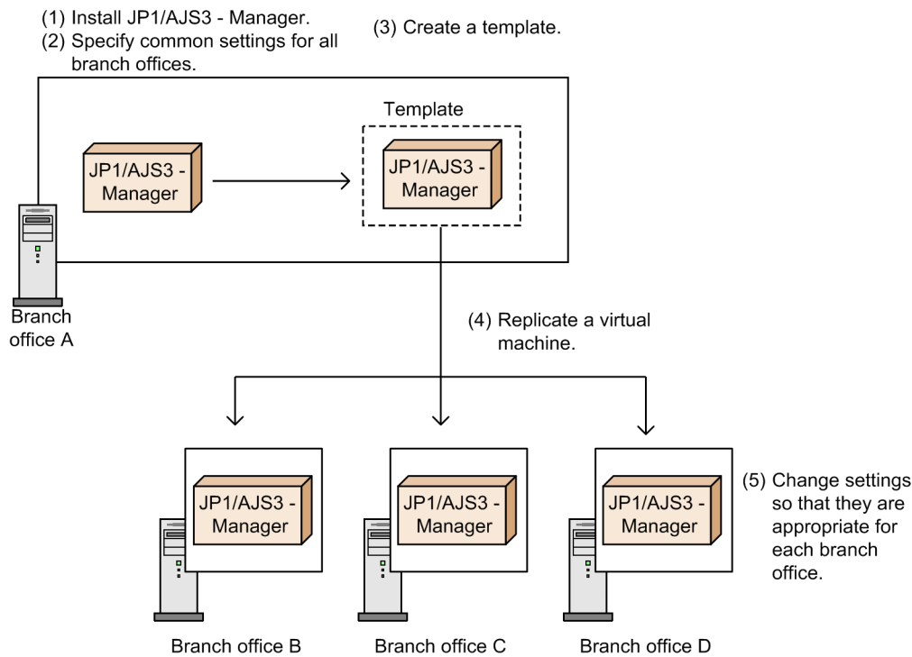
Figure 2–60: Operation example for replicating a virtual machine on which JP1/AJS3 - Manager has been set up
