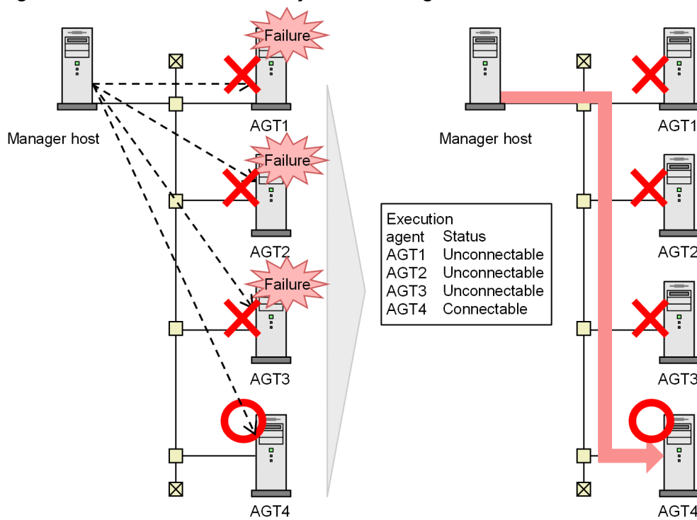
Figure 2–52: Distribution of a job according to the status of execution agents
