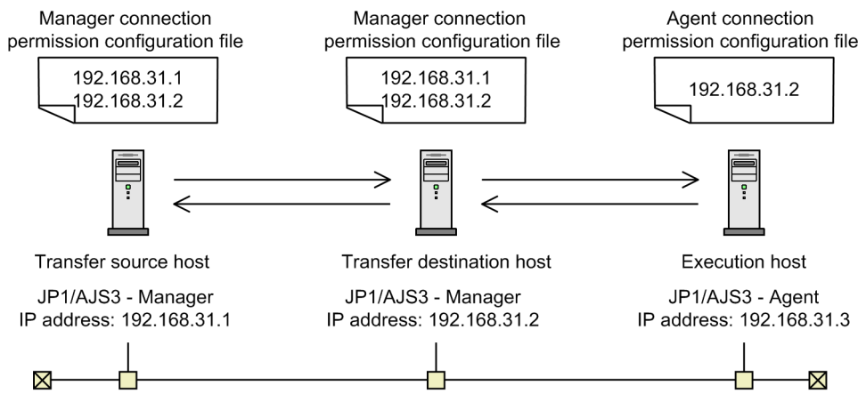
Figure 2–41: Example configuration when a remote jobnet is executed
