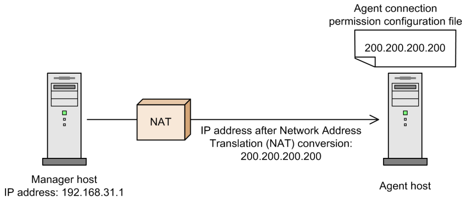
Figure 2–43: Example of restricting accesses in a NAT environment
