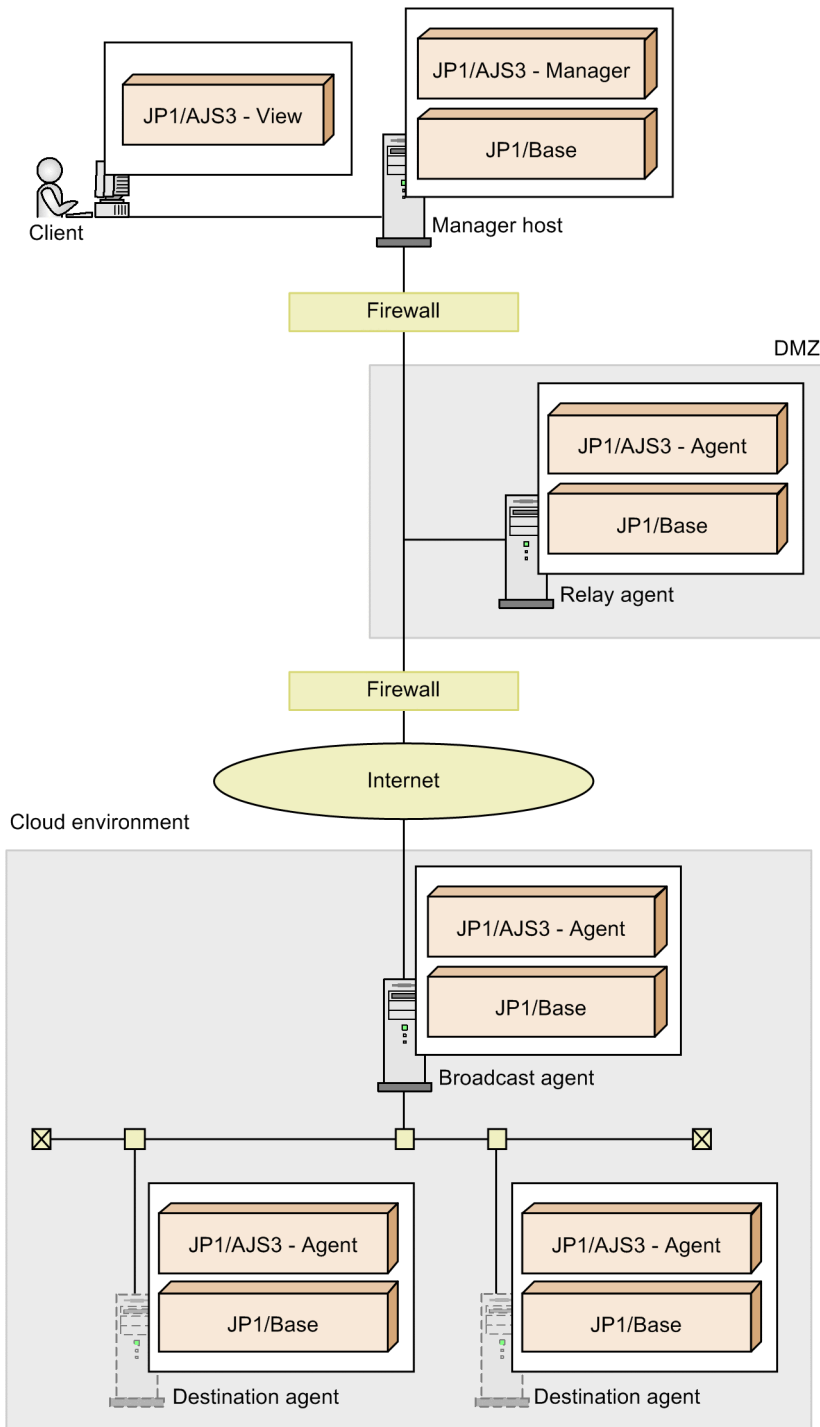
Figure 2–67: Example of a system configuration that uses a broadcast agent
