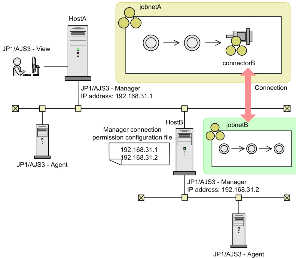
Figure 2–42: Example jobnet connector
