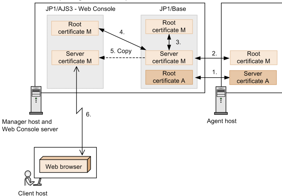
Figure 2–31: When the Web Console server and the manager host are installed on the same host (using JP1/Base)
