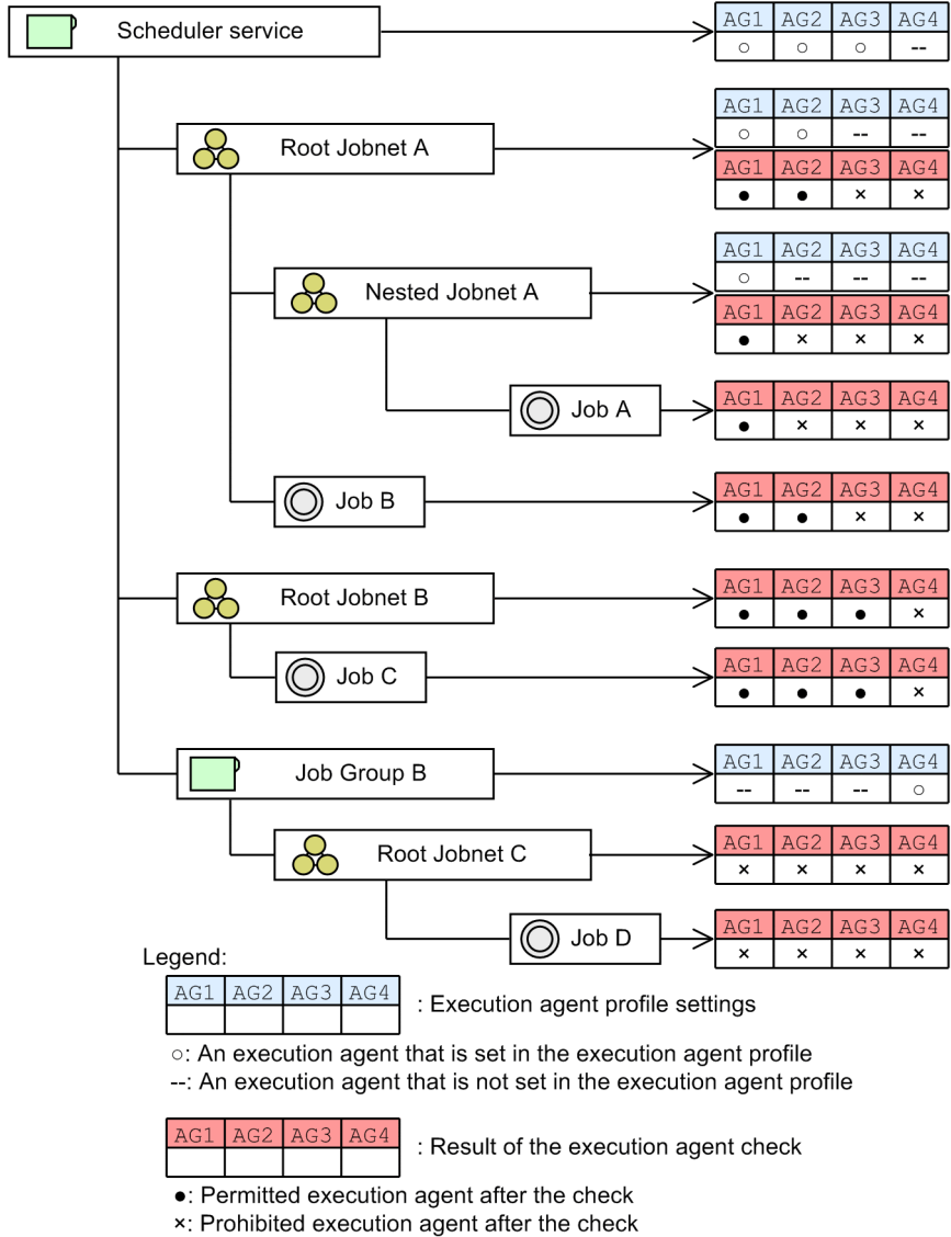
Figure 2–50: Execution agent profile settings and permitted execution agents
