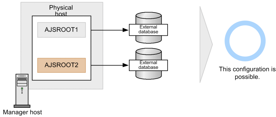
Figure 2–71: Example of configurations of a manager host connected with external databases
