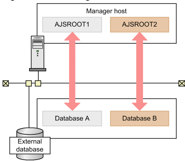
Figure 2–72: Configuration in which one manager host uses one instance of the external database
