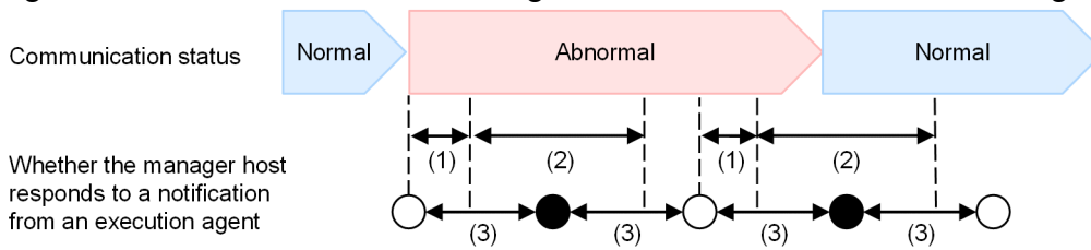
Figure 2–55: Interval for monitoring communication with execution agents
