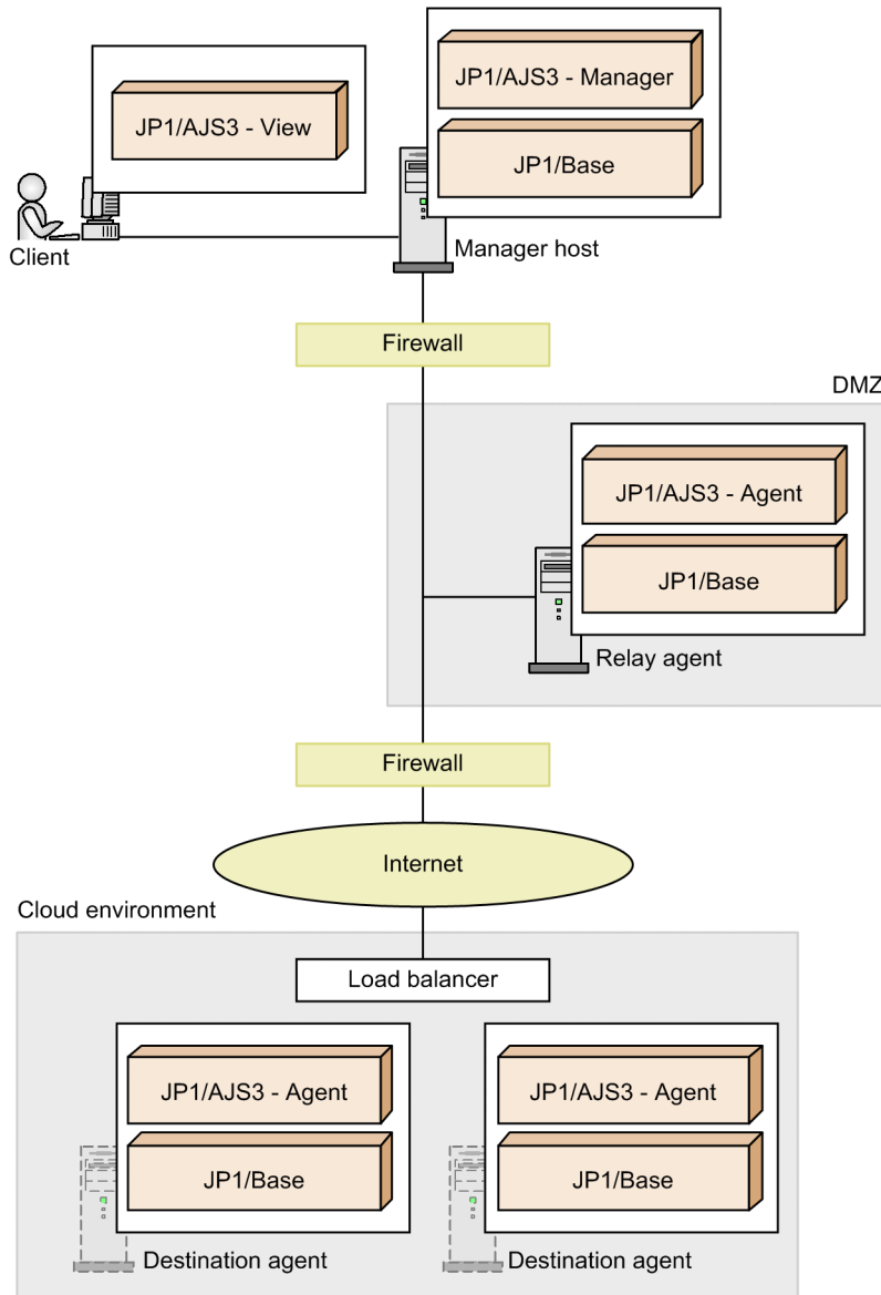
Figure 2–64: Example system configuration that includes a load balancer and a relay agent
