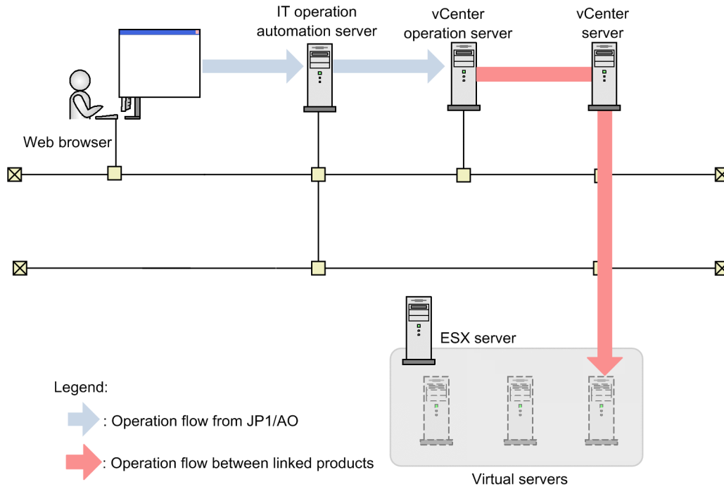
Figure 3–10: System configuration of Restart Virtual Machine
