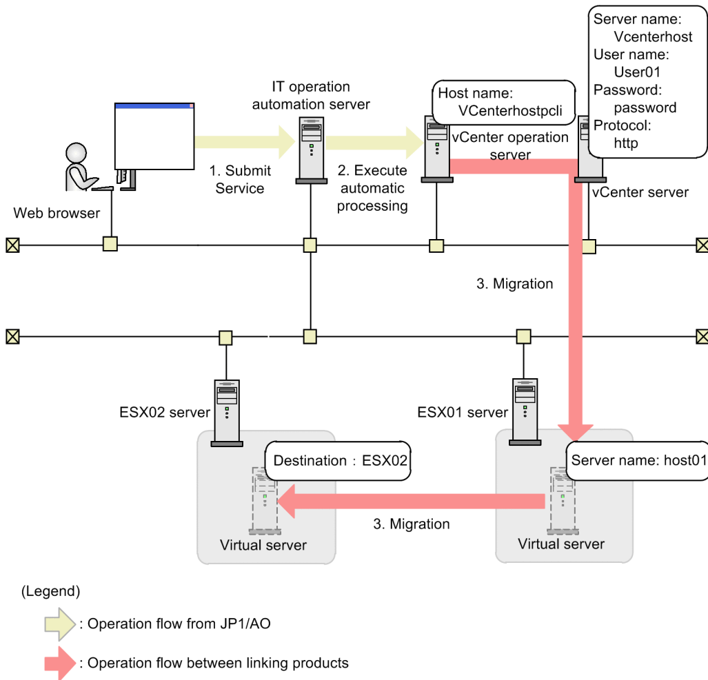
Figure 3–1: System configuration assumed for the Migrate Virtual Machine service template
