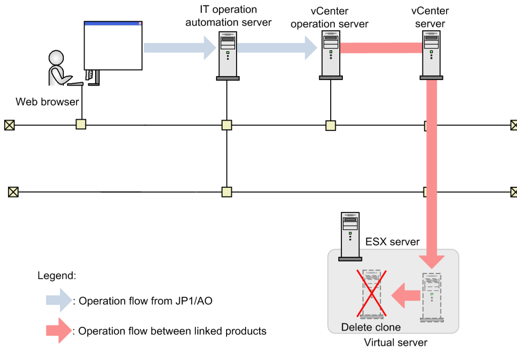
Figure 3–15: System configuration of Delete Cloned Virtual Machine
