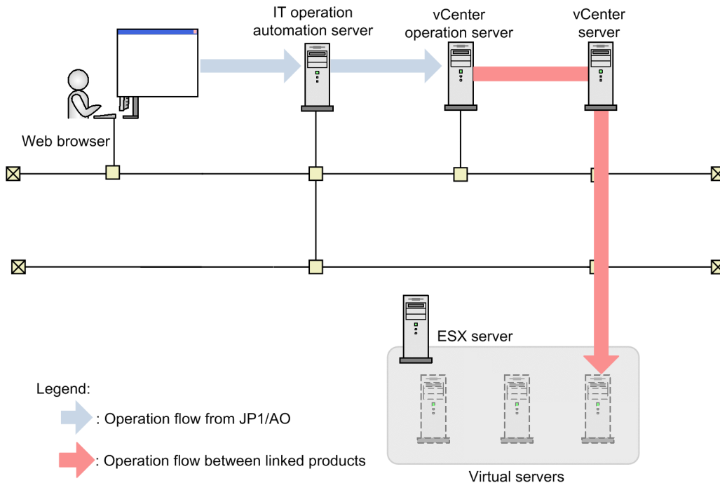
Figure 3–3: System configuration of Add Virtual Disk to Virtual Machine
