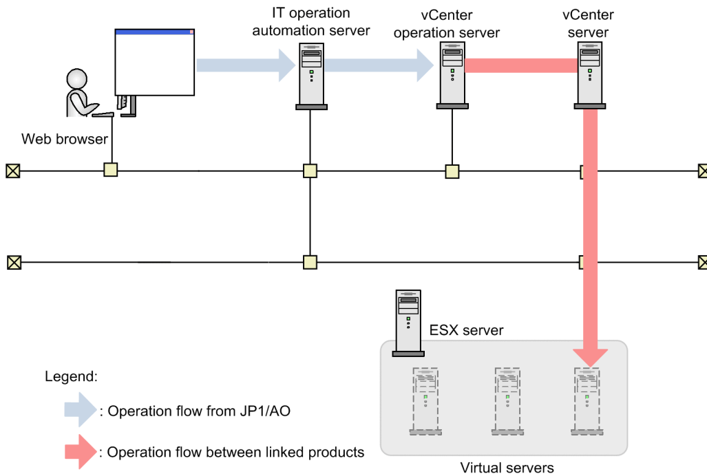
Figure 3–7: System configuration of Create Snapshot of Virtual Machine
