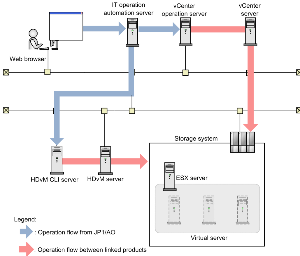
Figure 3–11: System configuration of Migrate Virtual Machine
