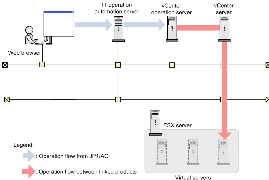
Figure 3–5: System configuration of Remove Virtual Disk from Virtual Machine
