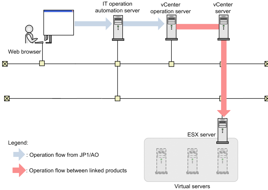
Figure 3–2: System configuration of Deploy and Setup OS on Virtual Machine
