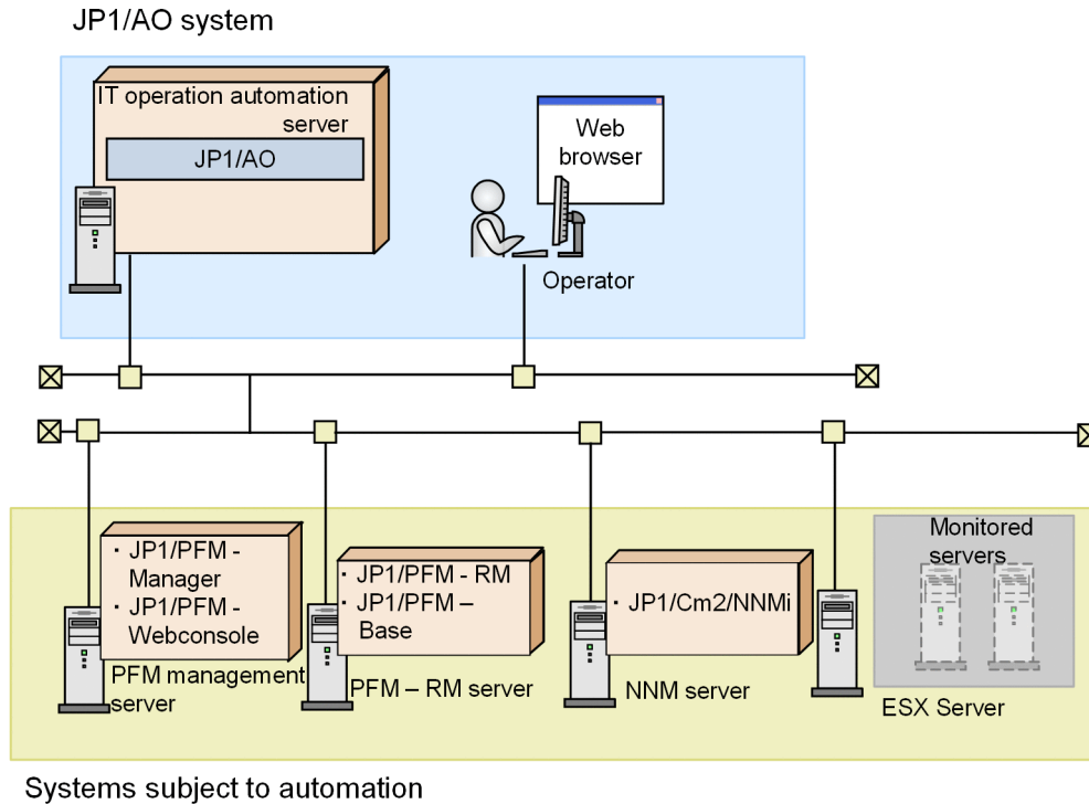
Figure 1-3: System configuration for an example application
