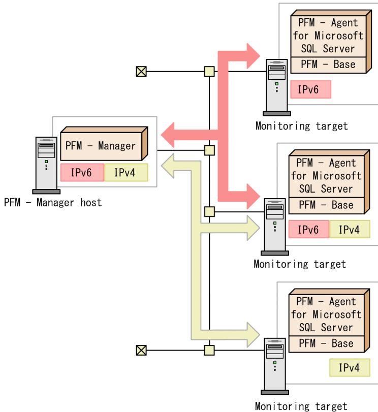
Figure L-1: Scope of communication when an IPv4 environment and an IPv6 environment are used
