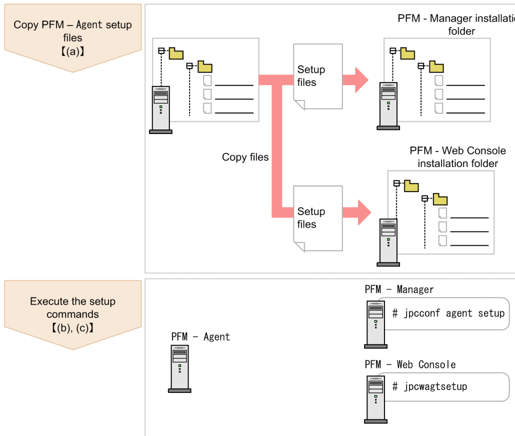
Figure 2–4: Procedure for registering PFM - Agent for Microsoft SQL Server
