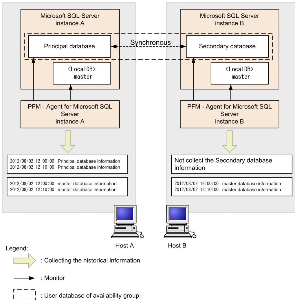
Figure 2–8: Example of monitoring in the SQL Server AlwaysOn Availability Group configuration
