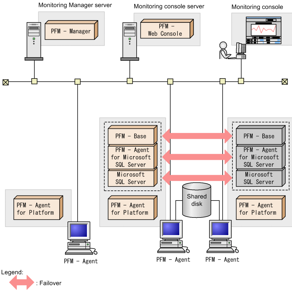
Figure 3–1: Example of an PFM - Agent for Microsoft SQL Server configuration in an HA cluster system
