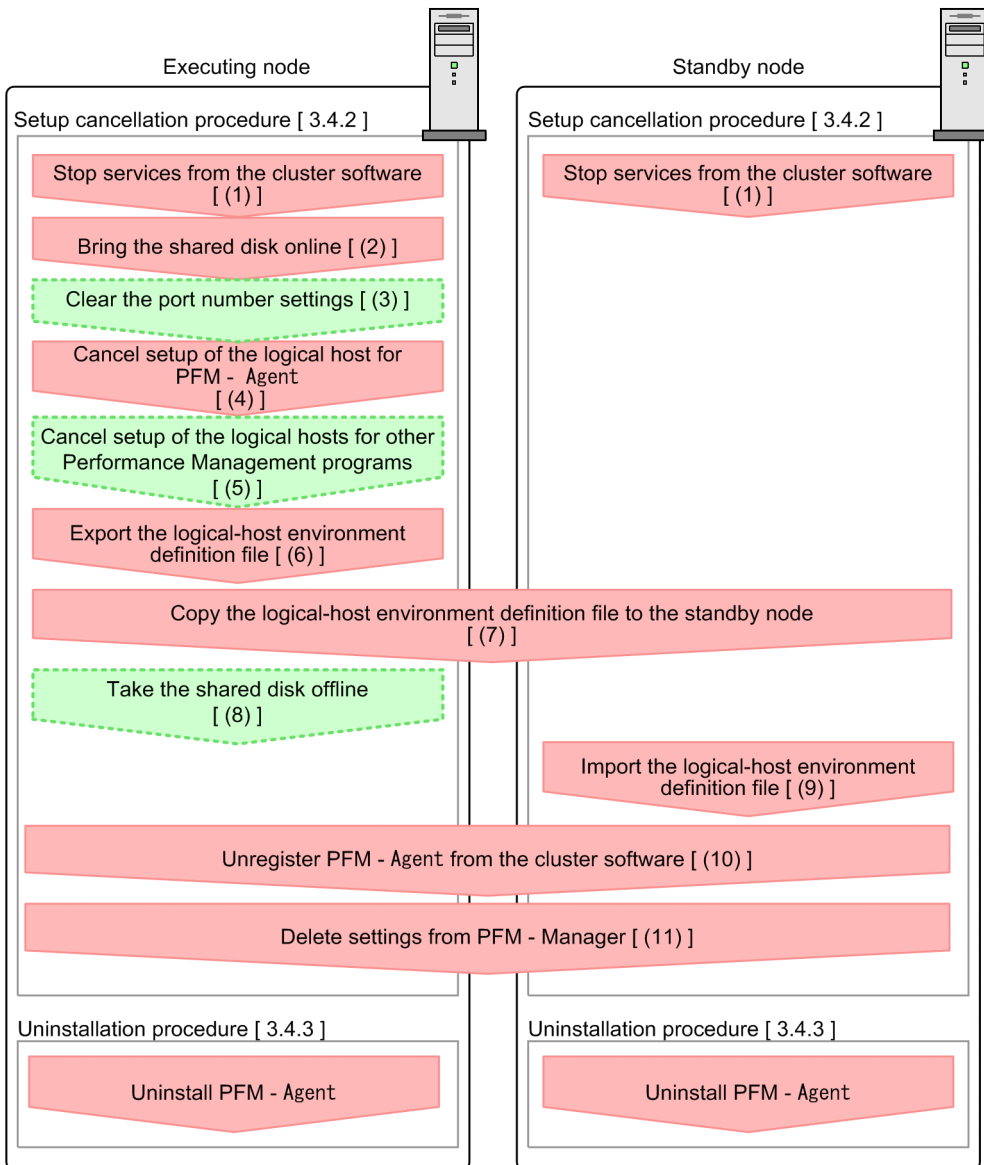
Figure 3–6: Setup cancellation and uninstallation workflow of PFM - Agent for Microsoft SQL Server running on a logical host in a cluster system (Windows)
