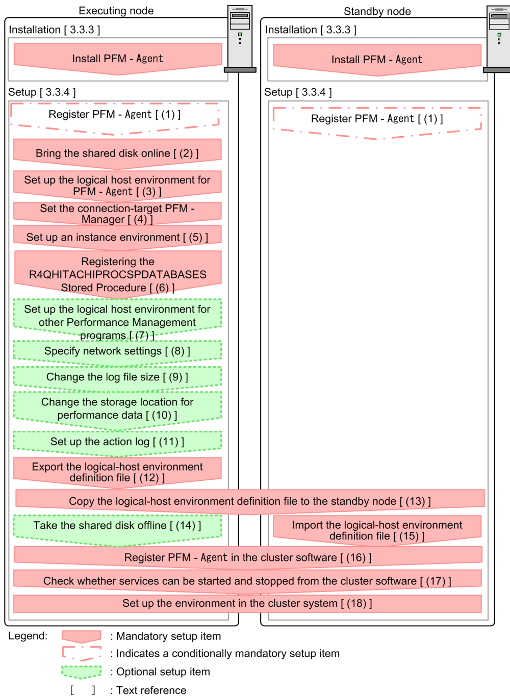
Figure 3–5: Flow of installing and setting up PFM - Agent for Microsoft SQL Server in a cluster system
