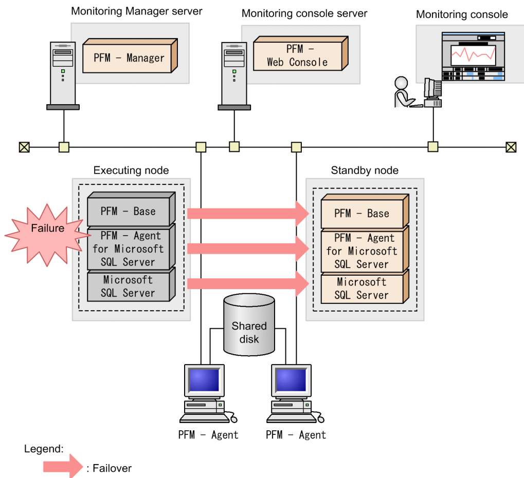
Figure 3–3: Processing when failover occurs on the PFM - Agent host
