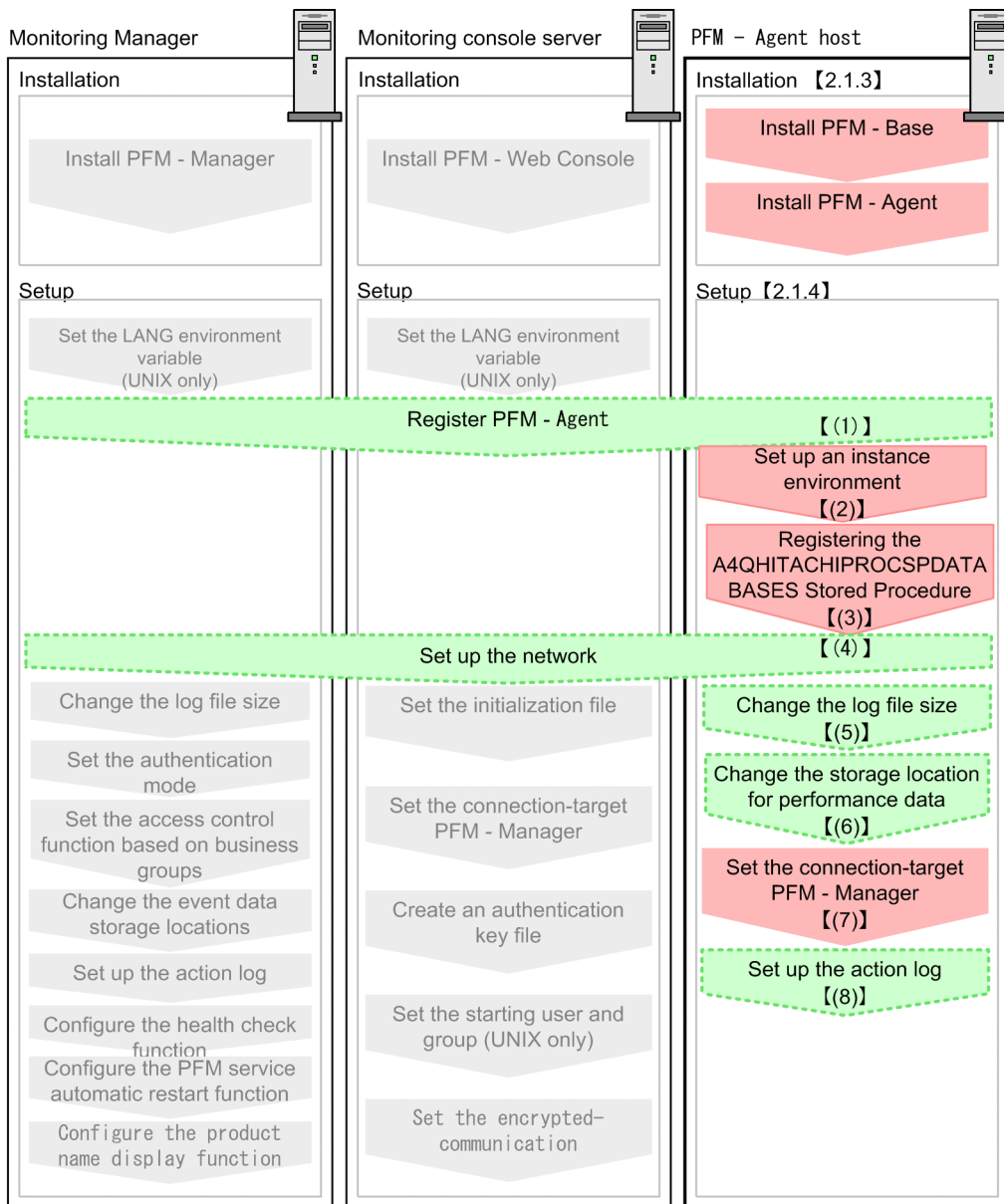
Figure 2–2: Installation and setup flow
