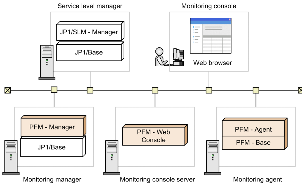
Figure 13–2: Program configuration for linking with JP1/SLM
