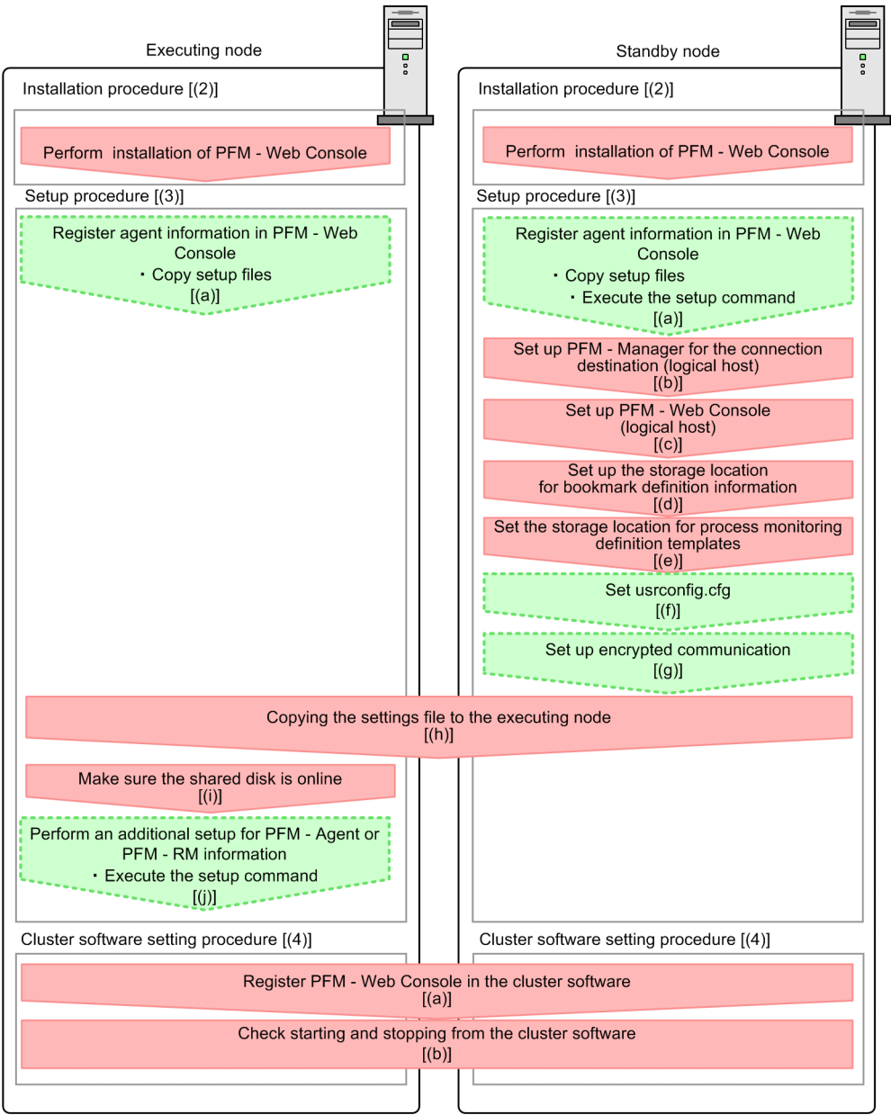
Figure 10–23: Process flow for installation and setup of PFM - Web Console used on a logical host
