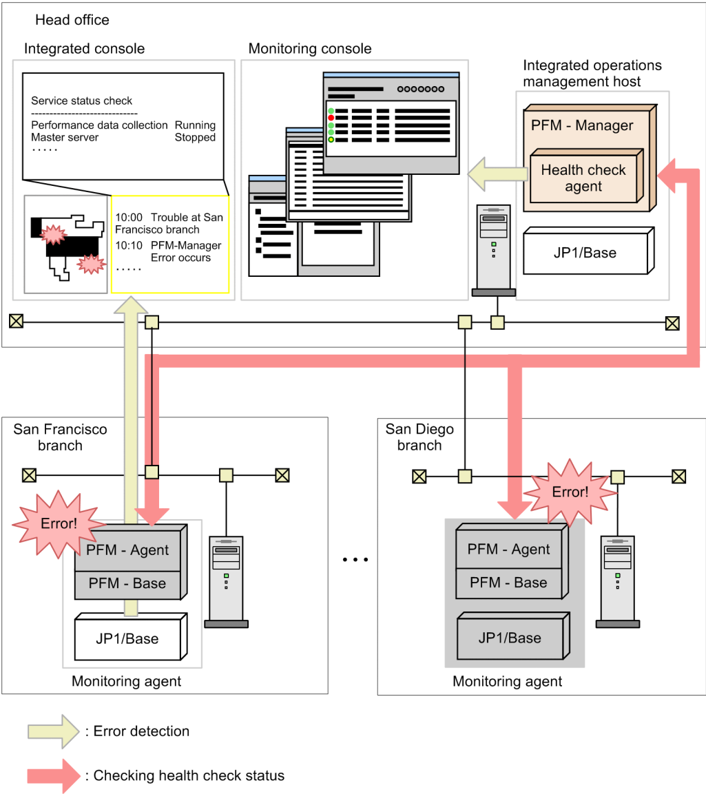
Figure 16–1: Example of detecting problems in Performance Management itself (PFM - Agent)
