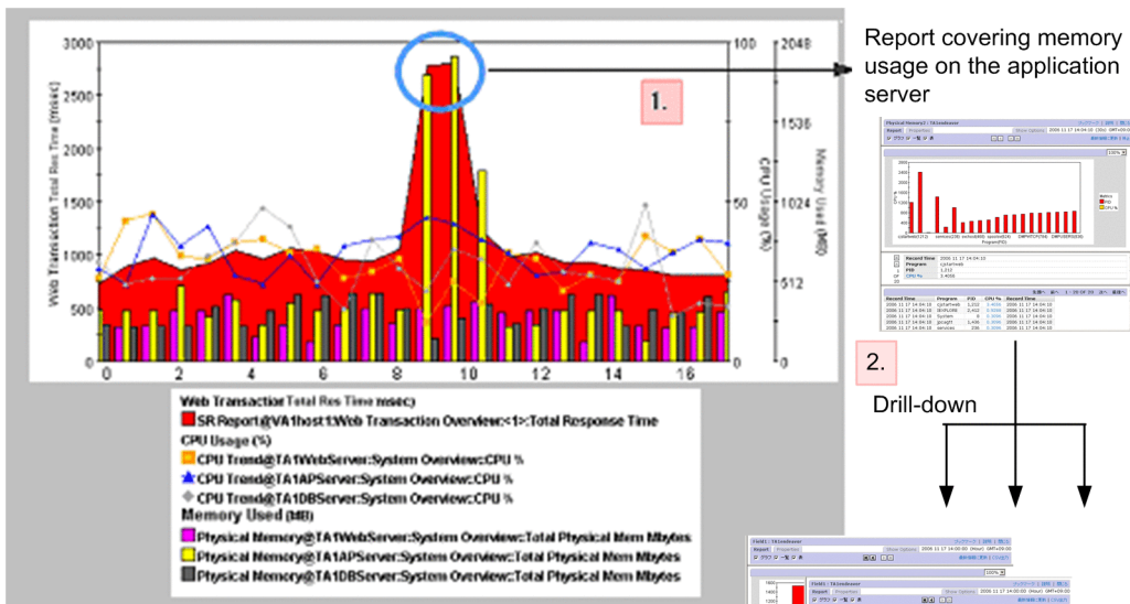
Figure 5–16: Example combining various types of report
