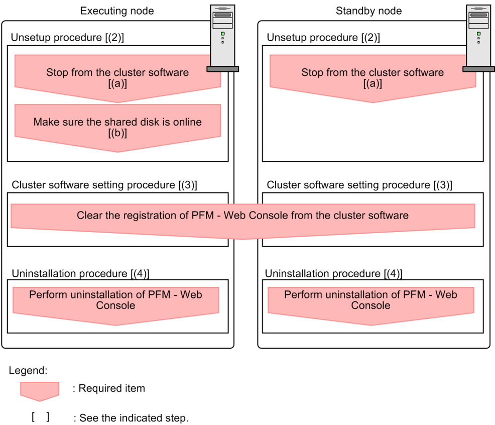
Figure 10–25: Process flow for unsetup and uninstallation of PFM - Web Console used on a logical host (in UNIX)
