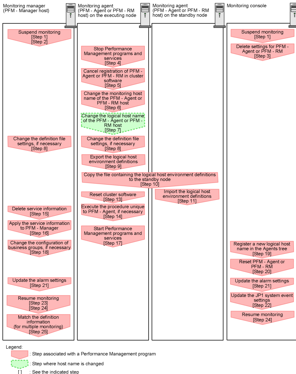
Figure 10–29: Changing the logical host name of PFM - Agent or PFM - RM
