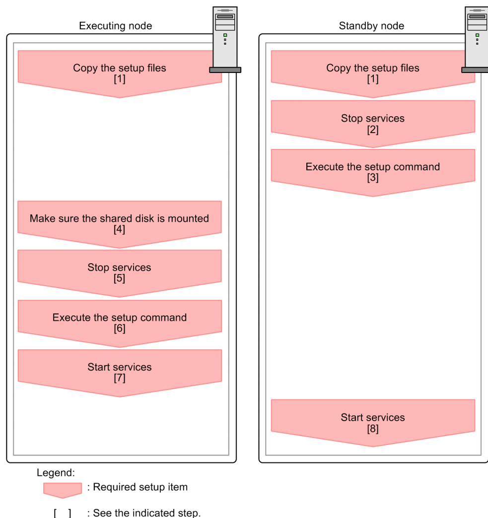
Figure 10–27: Additional PFM - Agent or PFM - RM information setup in PFM - Manager
