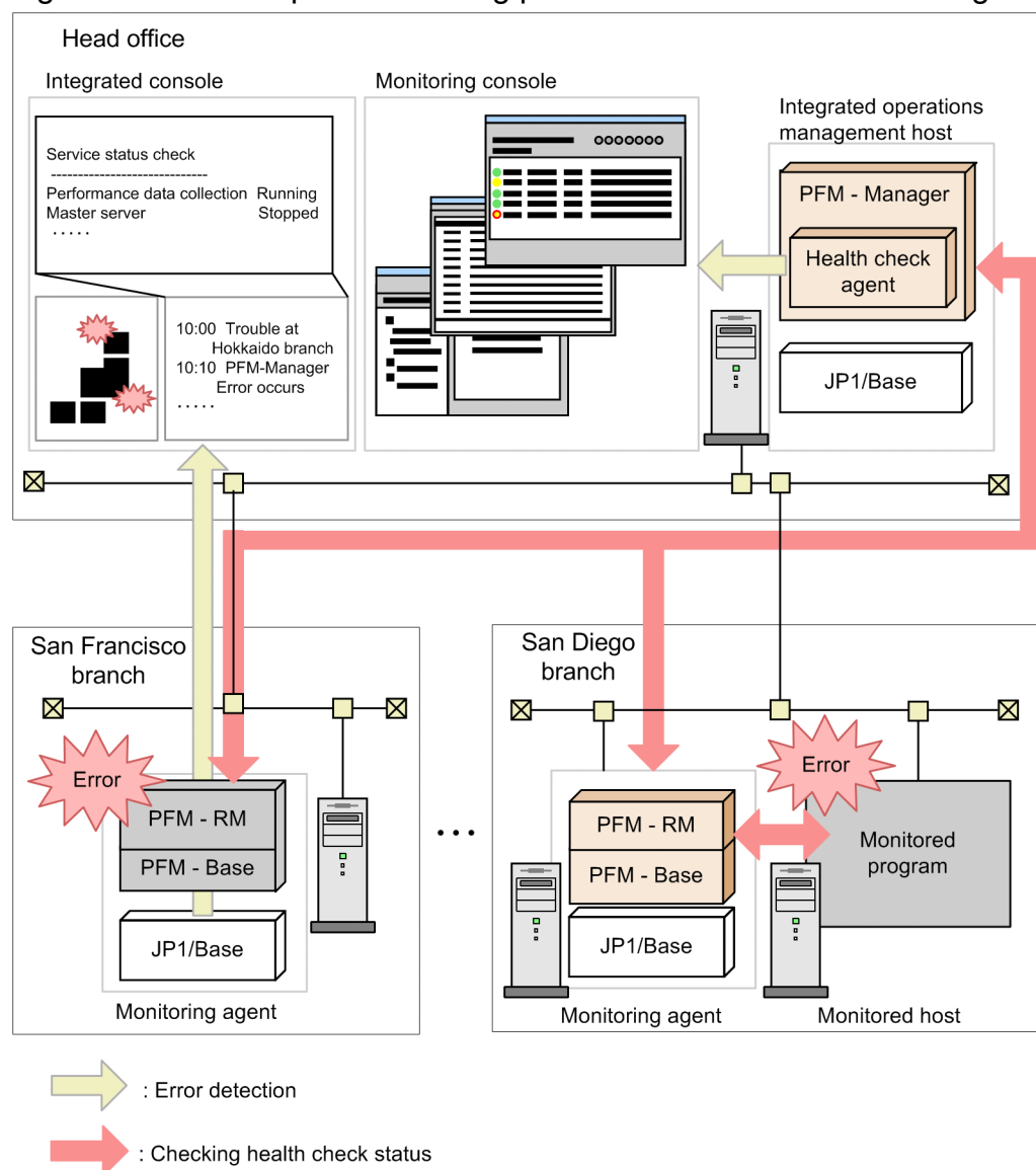
Figure 16–2: Example of detecting problems in Performance Management itself (PFM - RM)
