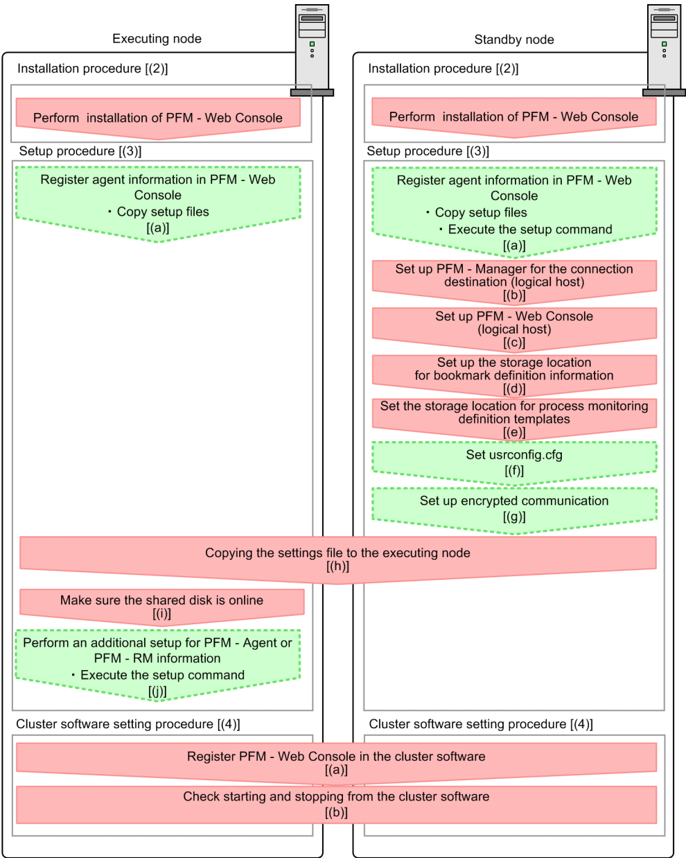
Figure 10–13: Process flow for installation and setup of PFM - Web Console used on a logical host
