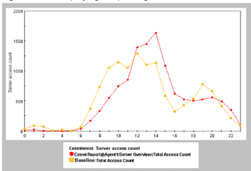
Figure 5–15: Displaying a report together with a baseline
