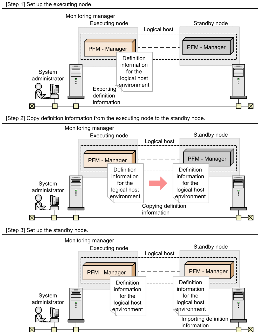
Figure 10–11: Method for applying the content set up on the executing node to the standby node
