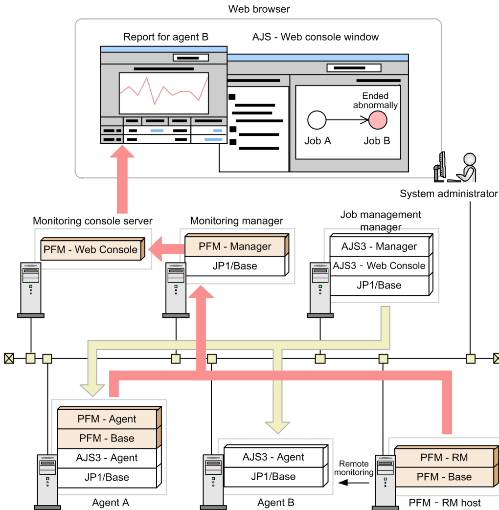
Figure 14–1: Example of monitoring with Performance Management linked with JP1/AJS3
