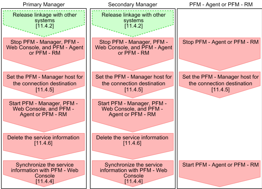
Figure 11–7: Procedure for terminating multiple monitoring when the primary Manager and the secondary Manager will be used separately
