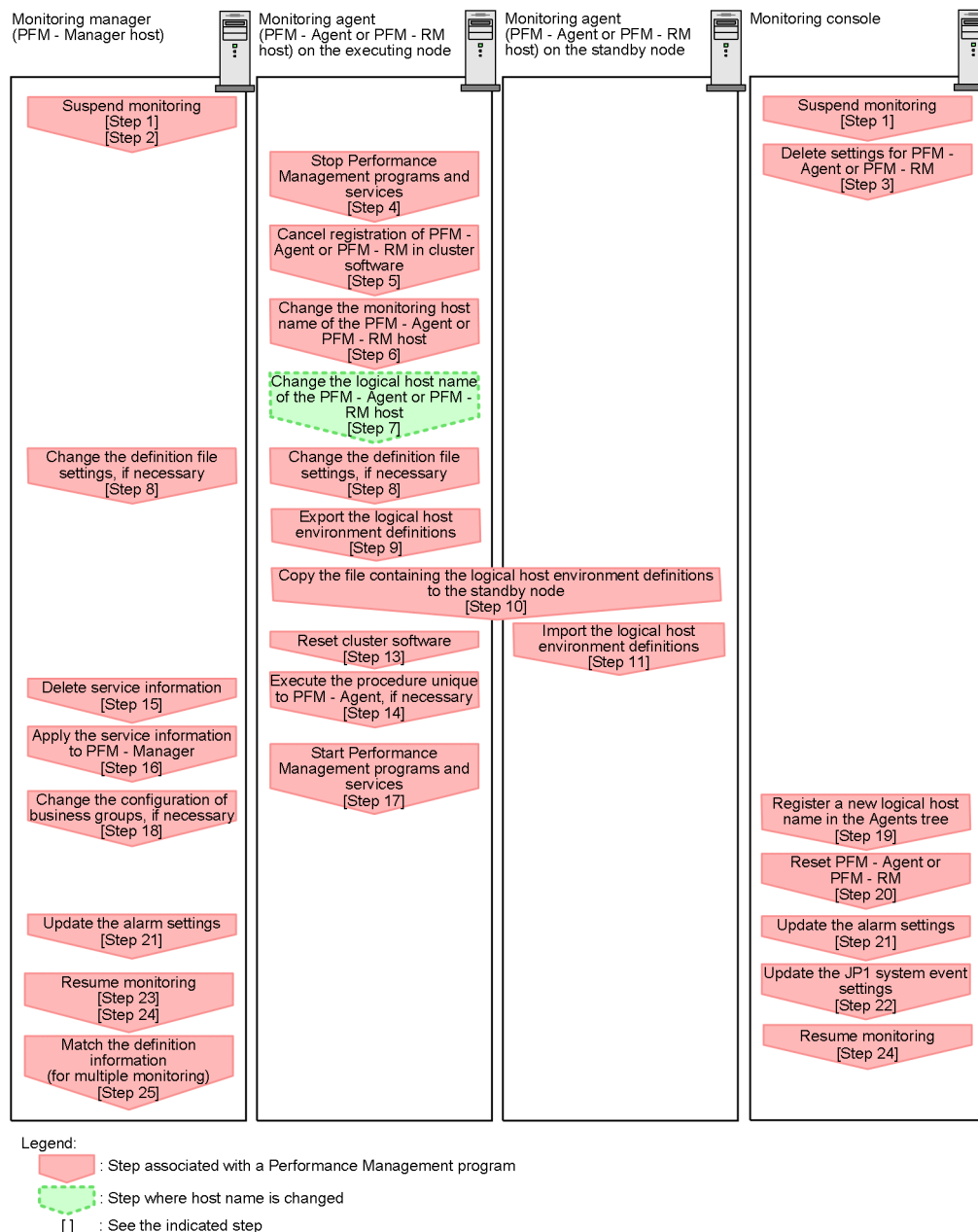
Figure 10–19: Changing the logical host name of PFM - Agent or PFM - RM
