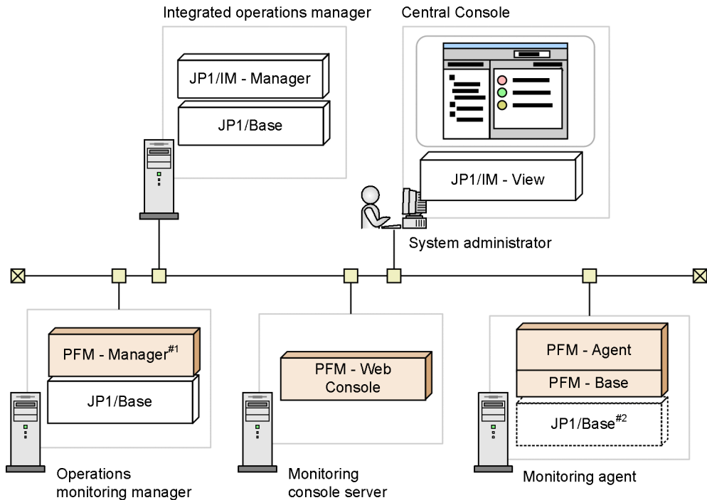
Figure 12–2: JP1/IM installation configuration for linkage with JP1/IM
