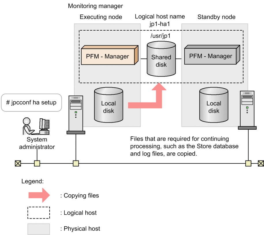
Figure 10–22: Execution example of the jpccnf ha setup command
