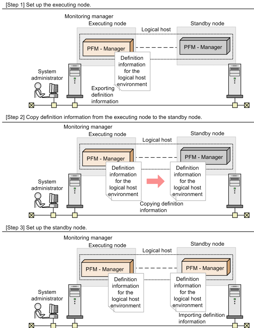
Figure 10–21: Method for applying the content set up on the executing node to the standby node
