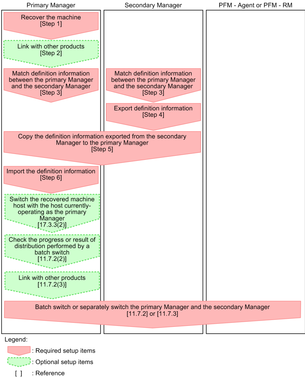
Figure 17–5: Procedure for recovering the machine that is down and reconfiguring it as the primary Manager
