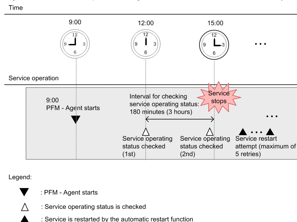
Figure 16–15: Example of using the automatic restart functionality
