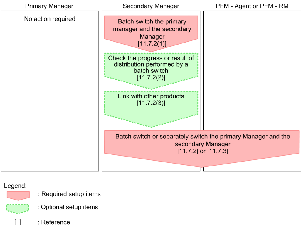
Figure 11–9: Procedure for switching the primary Manager and the secondary Manager
