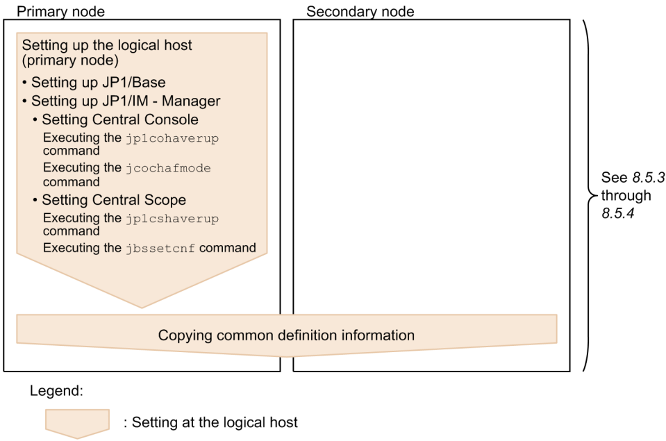
Figure 8–3: Setup procedure (when upgrading the existing logical host environment)
