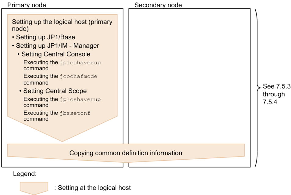
Figure 7–5: Setup procedure (when upgrading the existing logical host environment)
