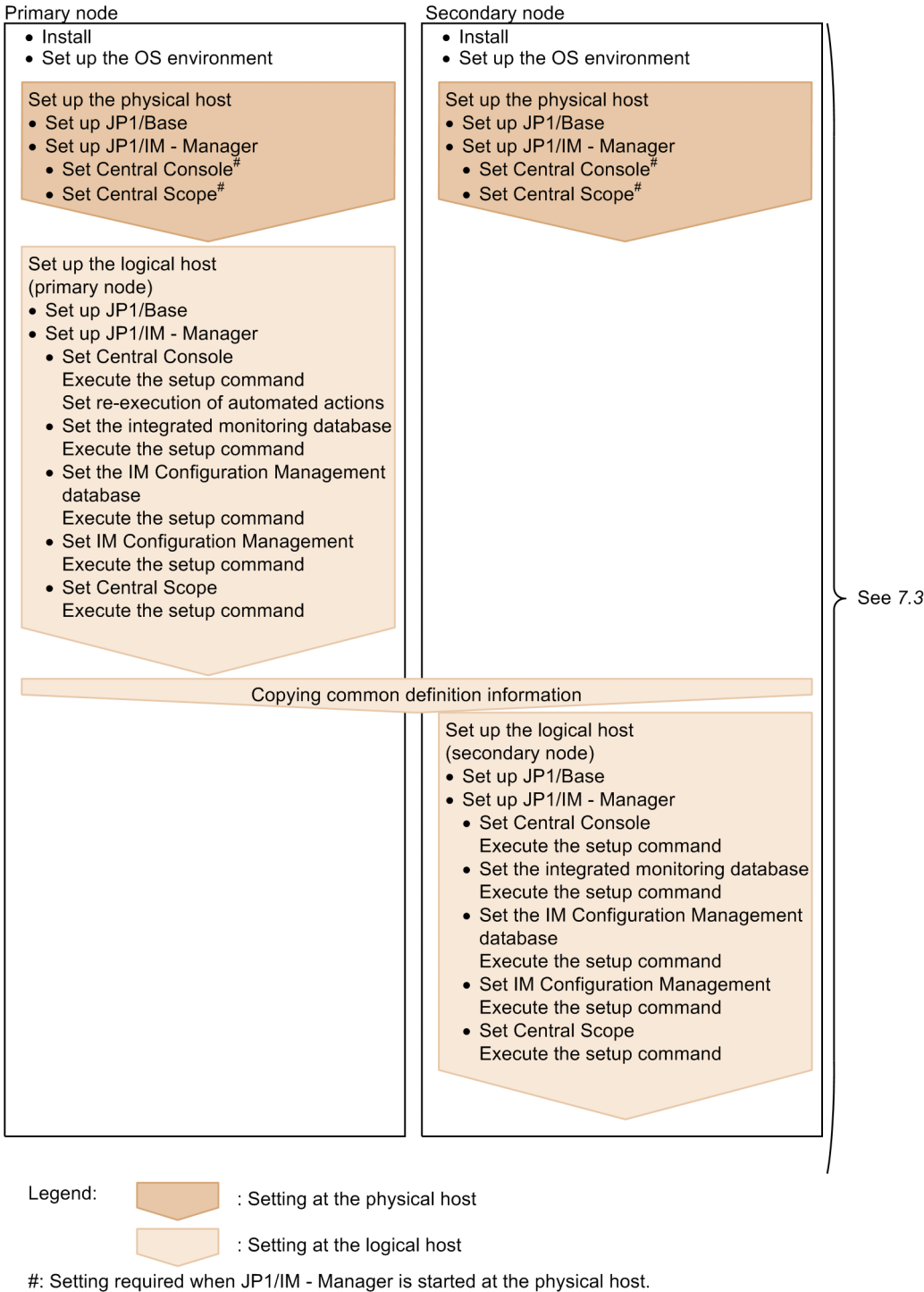
Figure 7–4: Setup procedure (when setting up a new environment)
