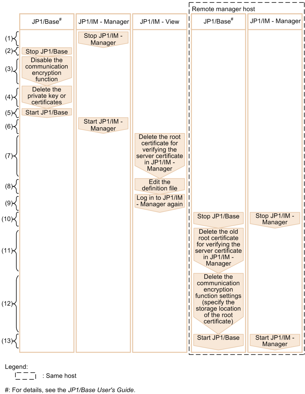
Figure 9–11: Procedure for stopping using the communication encryption function
