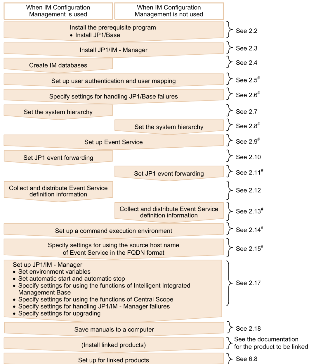
Figure 2–1: Installation and setup procedure (manager)
