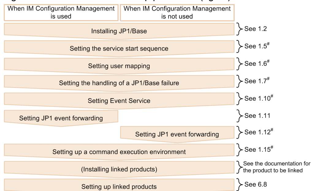
Figure 1–2: Installation and setup procedure (agent)
