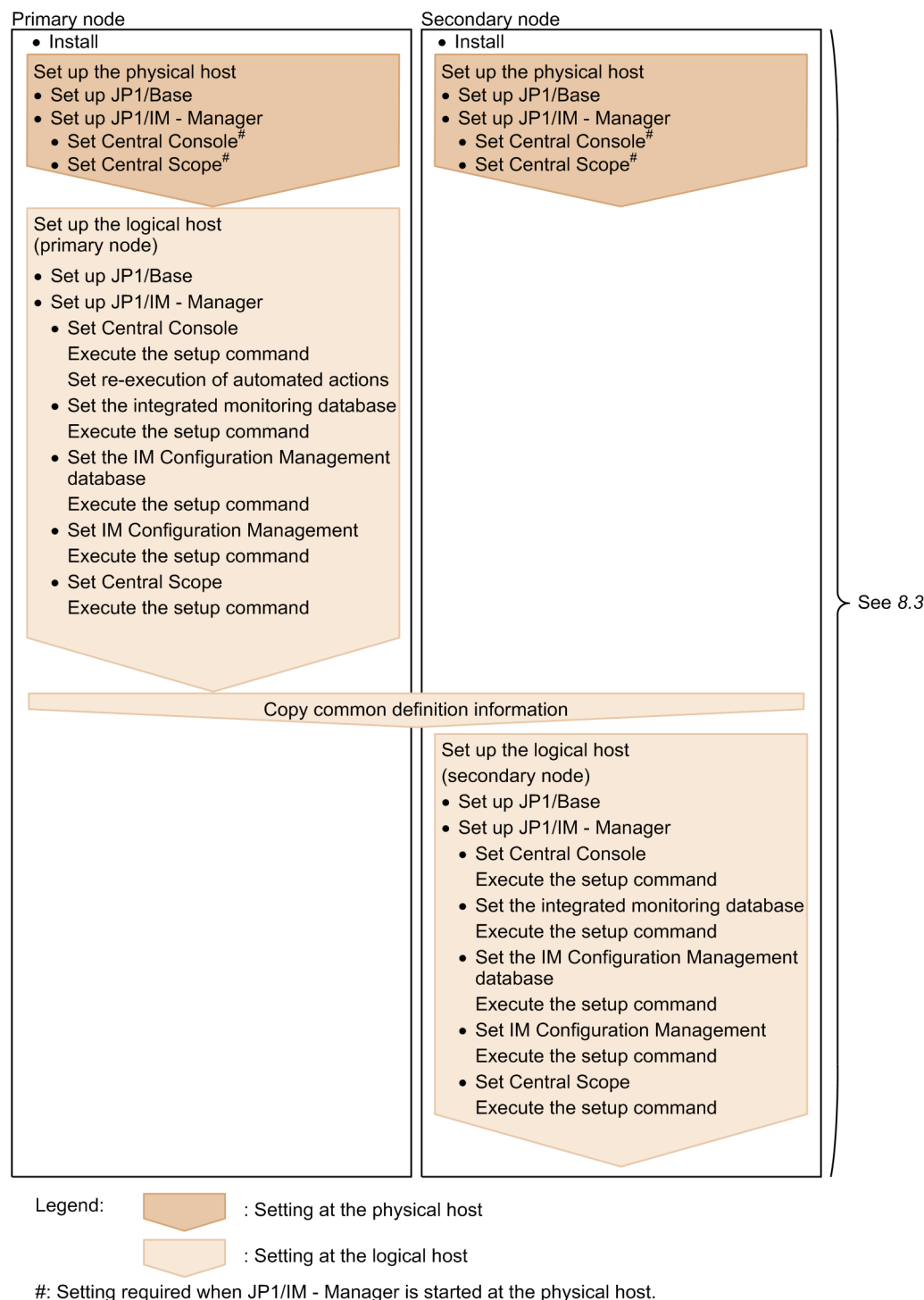
Figure 8–2: Setup procedure (when setting up a new environment)
