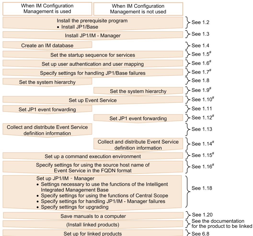
Figure 1–1: Installation and setup procedure (manager)
