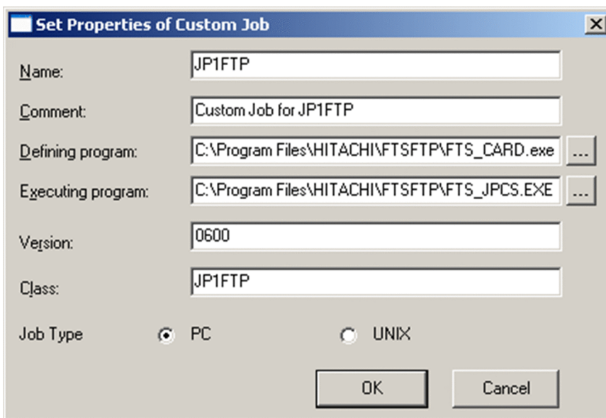
Figure 5–2: Set Properties of Custom Job dialog box
