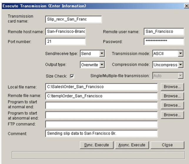
Figure 3–15: Execute Transmission (Enter Information) dialog box
