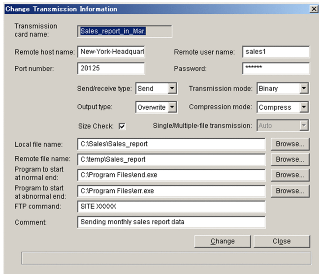
Figure 3–12: Change Transmission Information dialog box
