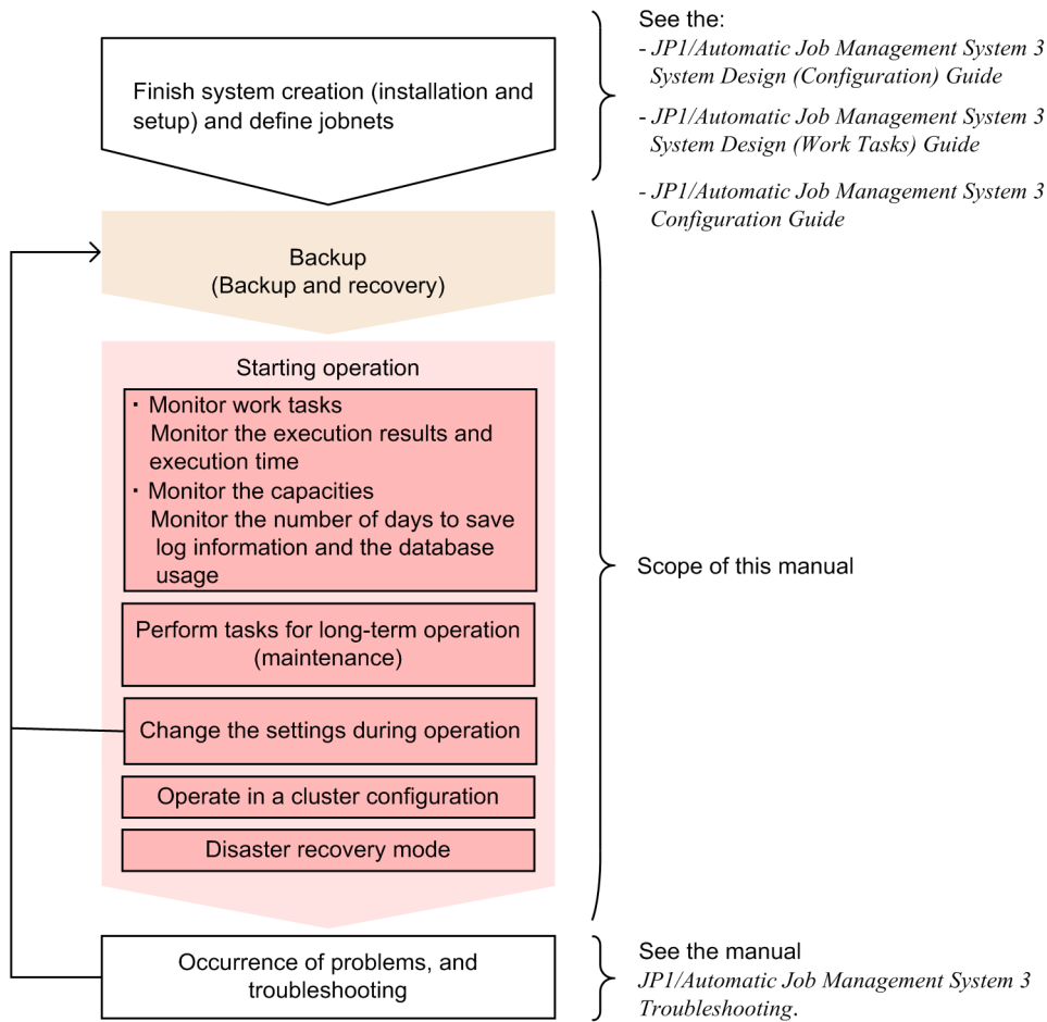
Figure 1-1: Example of operation using JP1/AJS3
