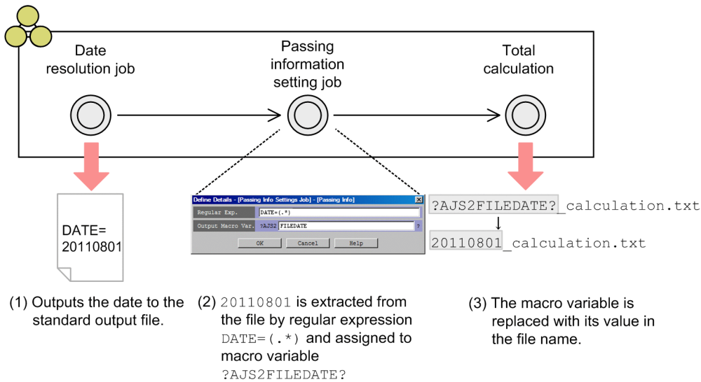
Figure 12–10: Assigning the date to the total calculation job standard output file name
