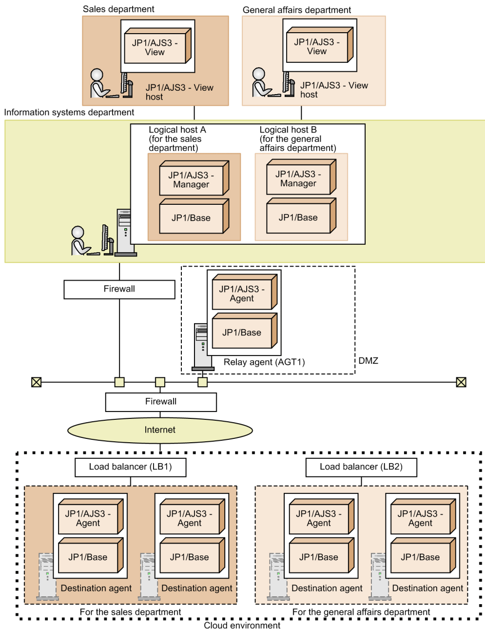
Figure 12–18: Example in which a cloud is used as the job execution environment
