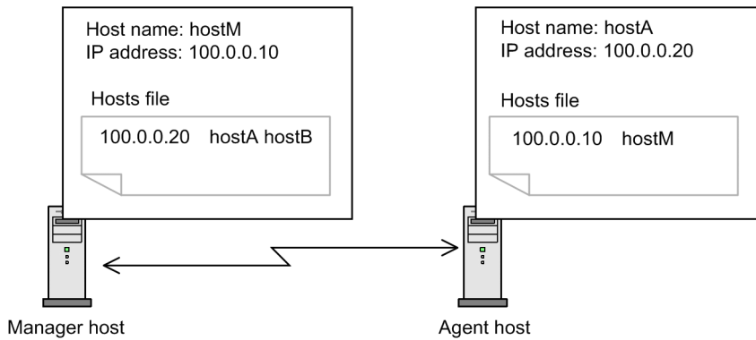
Figure 12–13: Example of hosts file defining an alias host name
