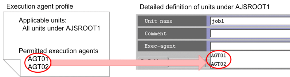
Figure 12–6: Execution agent restriction (at unit definition)
