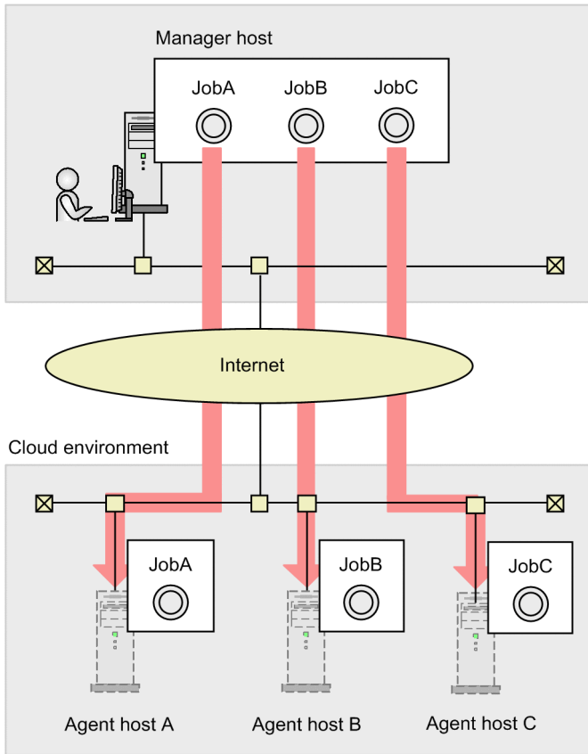
Figure 12–20: Example in which jobs are added or deleted
