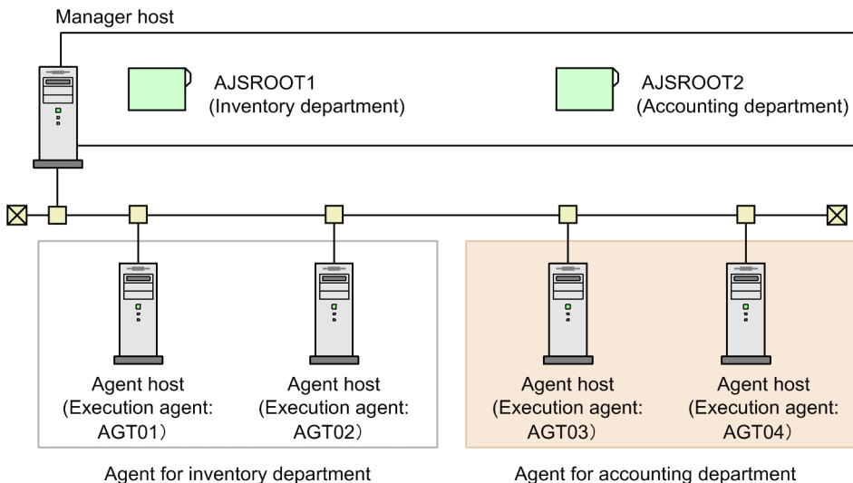
Figure 12–4: Example using different execution agents and scheduler services
