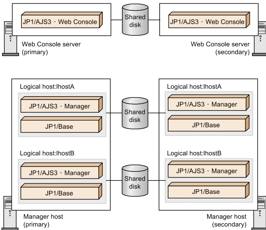
Figure 10–2: If you set up a cluster by installing JP1/AJS3 - Web Console and JP1/AJS3 - Manager on different hosts
