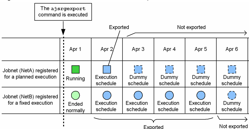
Figure 3–3: Execution schedules to be exported
