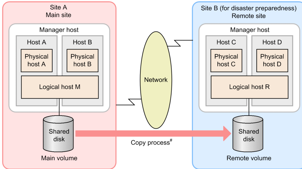
Figure 11–1: Overview of JP1/AJS3 disaster recovery operation
