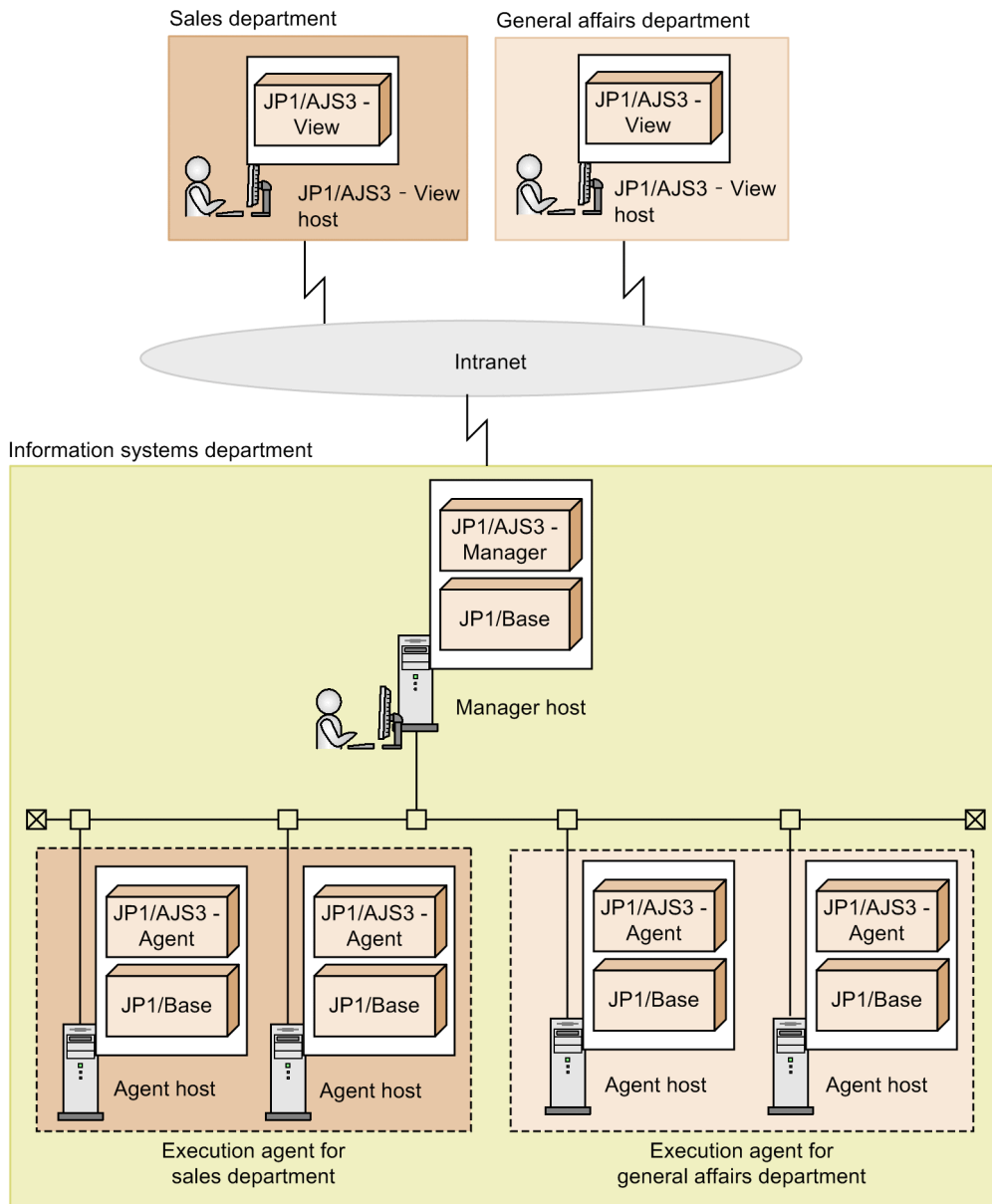
Figure 12–16: Configuration example of an integrated JP1/AJS3 system
