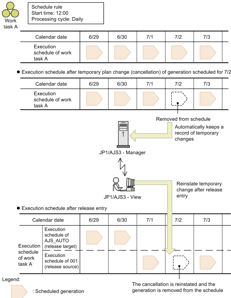
Figure 12–12: Example of reinstating temporary change made prior to release
