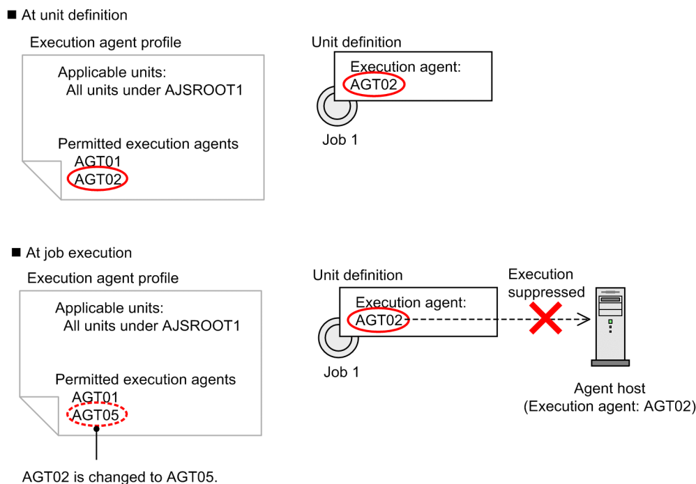
Figure 12–7: Execution agent restriction (at job execution)
