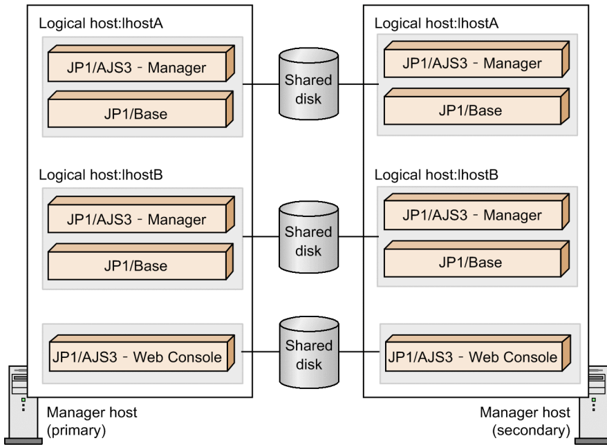
Figure 10–3: If you separately set up clusters by installing JP1/AJS3 - Web Console and JP1/AJS3 - Manager on the same host
