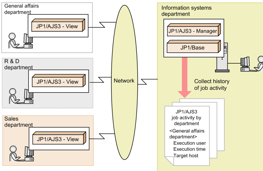
Figure 12–2: Example of collecting job histories
