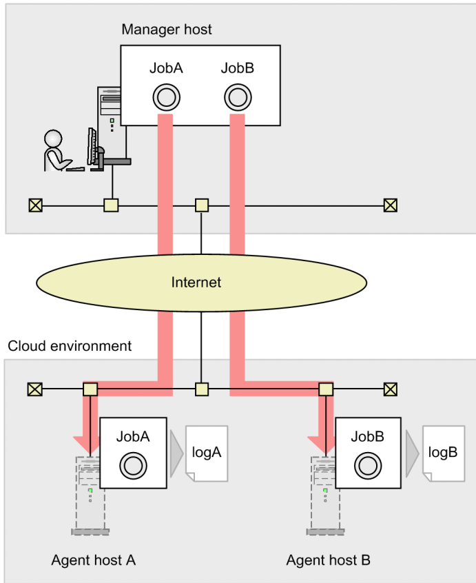
Figure 12–19: Example in which a job is defined for each agent host
