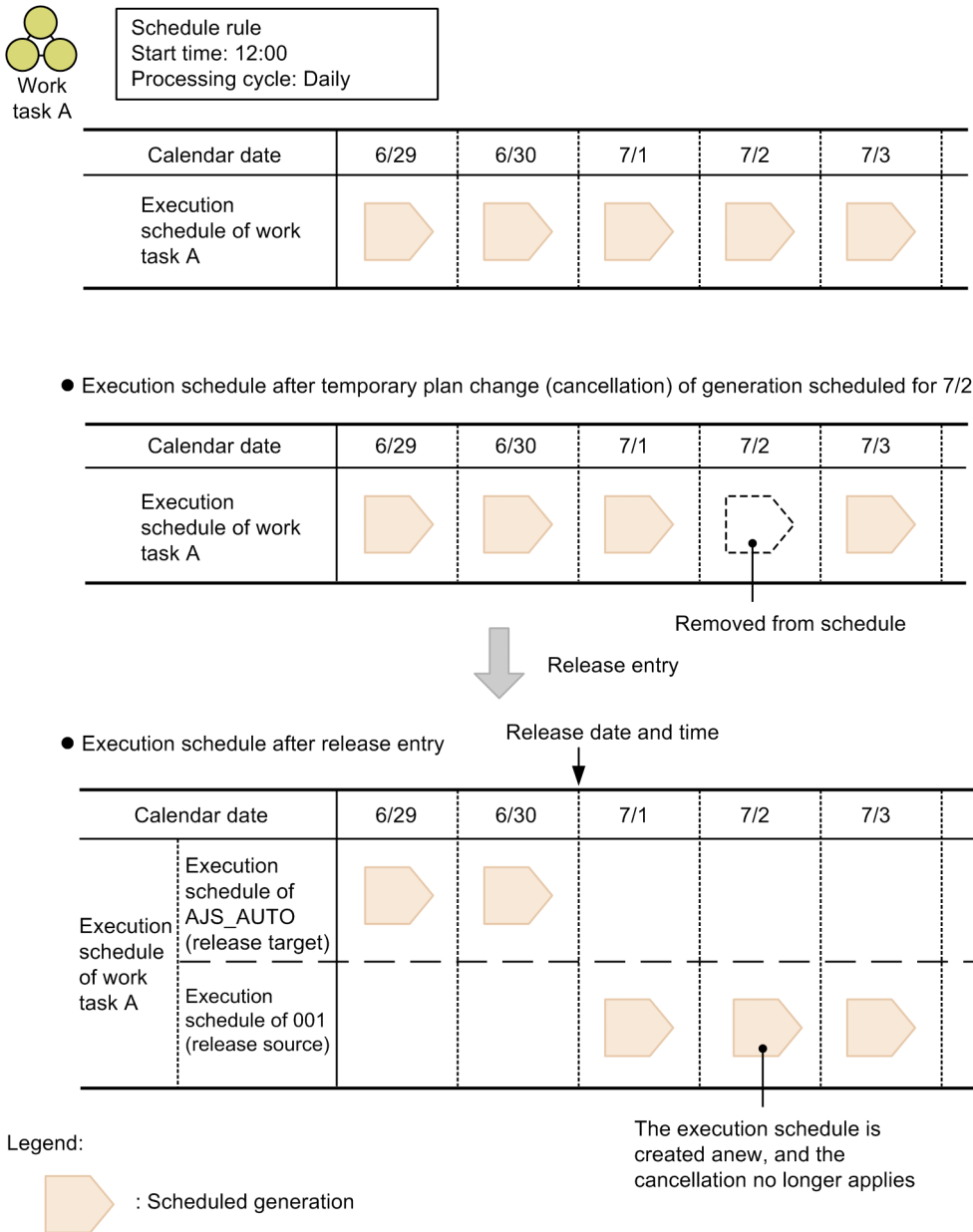
Figure 12–11: Example of release registration after temporary schedule change
