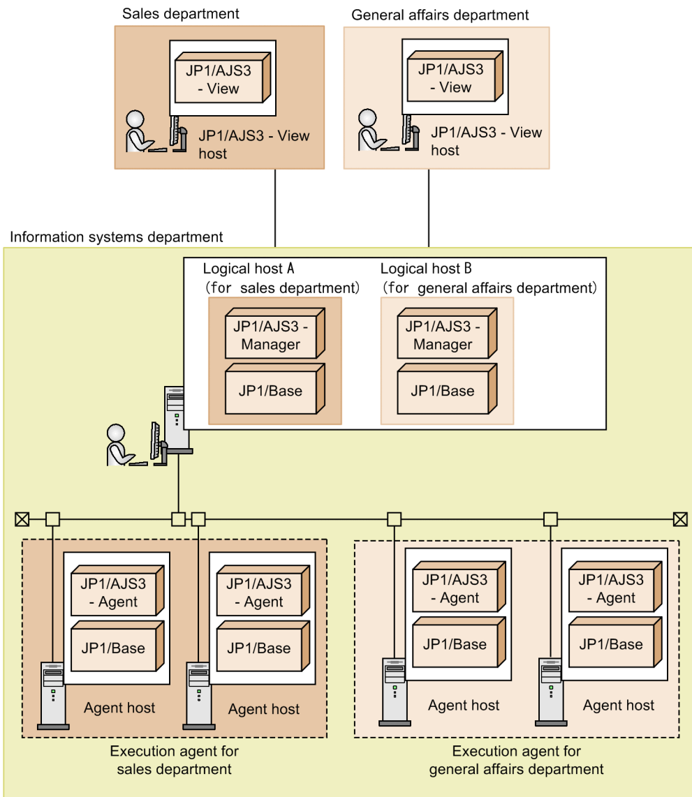
Figure 12–17: Example in which the manager host and agent hosts are operated in the premises environment of each department
