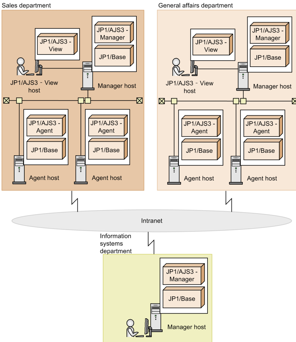
Figure 12–15: An example in which each department operates its own manager host and agent hosts
