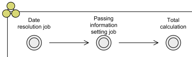
Figure 12–9: Flow of jobnet execution
