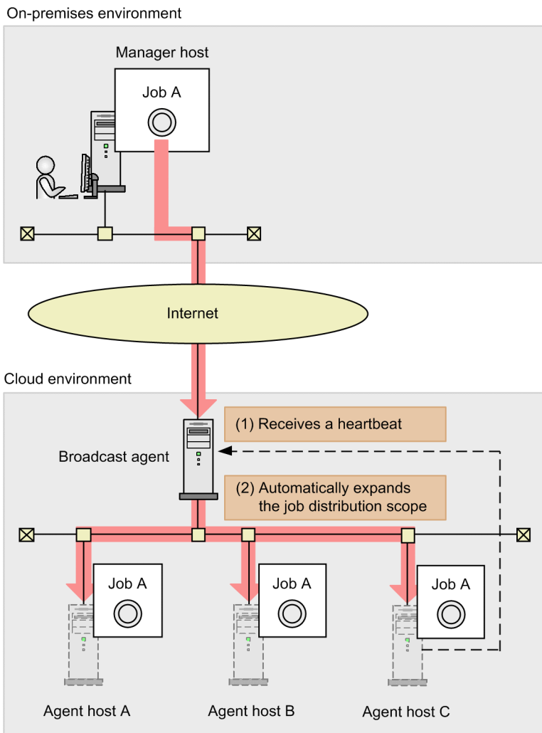
Figure 12–22: Example in which a broadcast agent automatically expands the distribution scope
