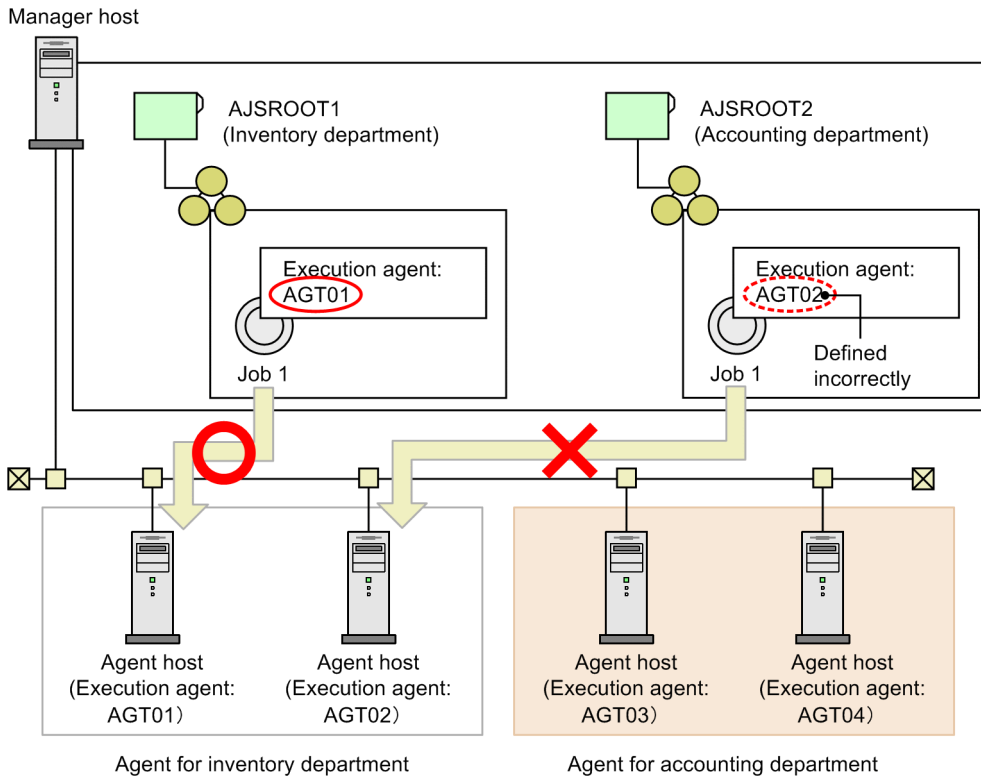
Figure 12–5: Example of job execution using an execution agent allocated to another department
