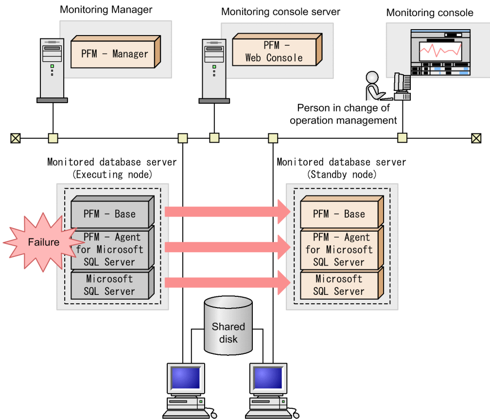
Figure 1–1: Example of an PFM - Agent for Microsoft SQL Server configuration in an HA cluster system
