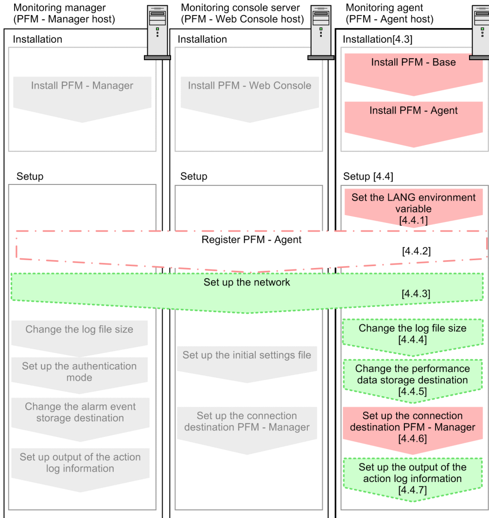
Figure 4–1: Installation and setup flow
