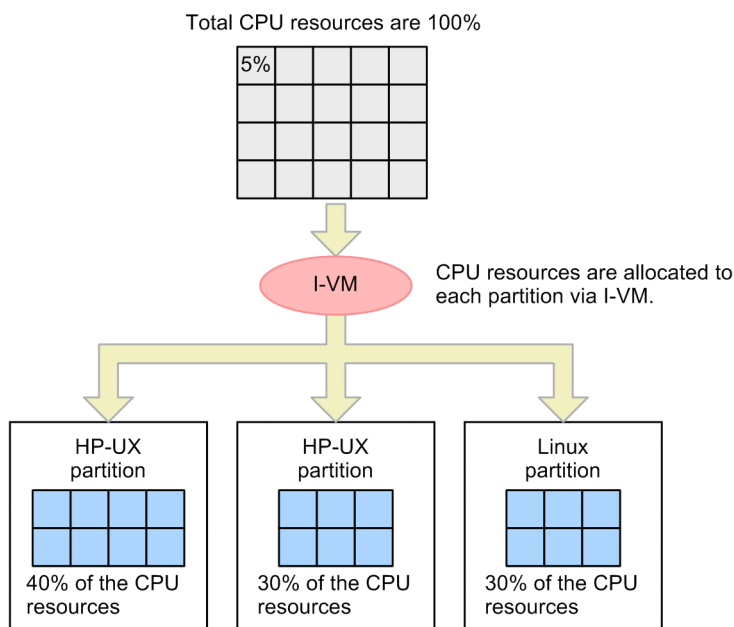
Figure 2–12: HP Integrity Virtual Machines structure
