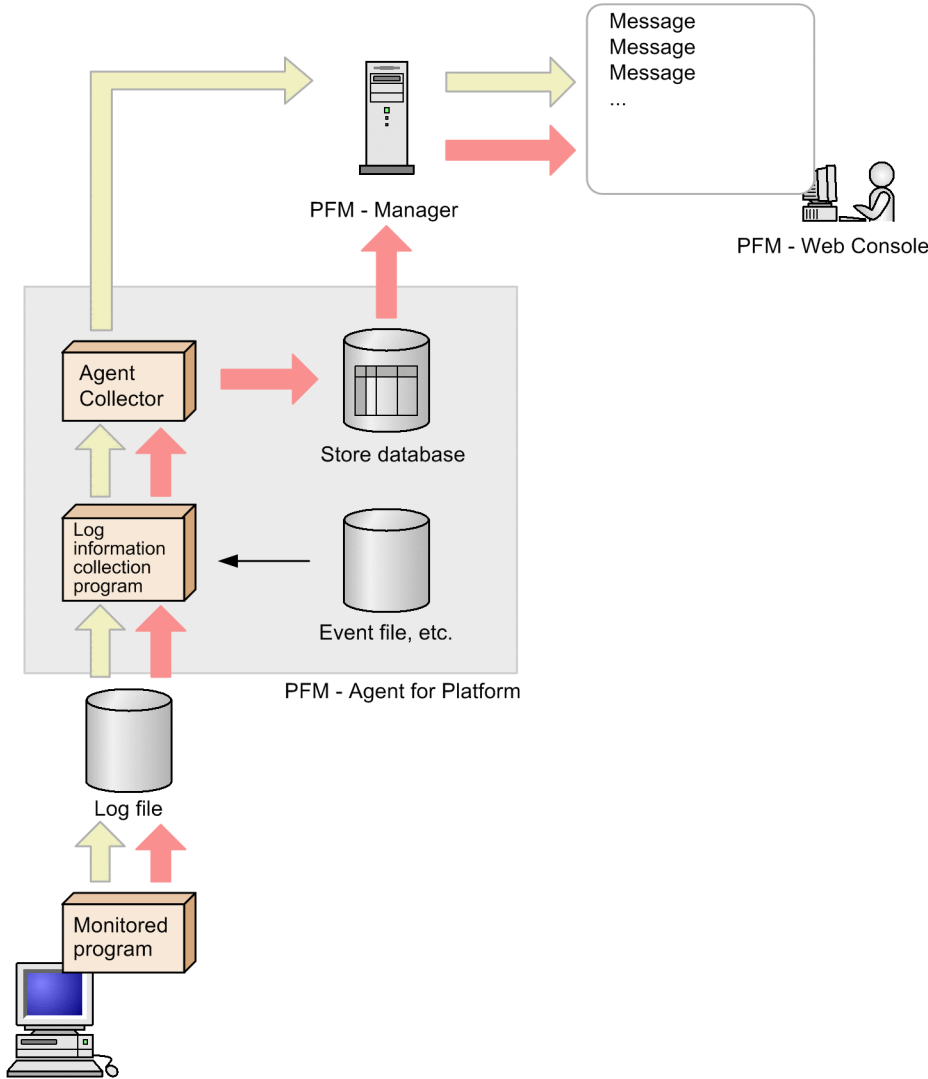
Figure 5-1: Log information monitoring flow
