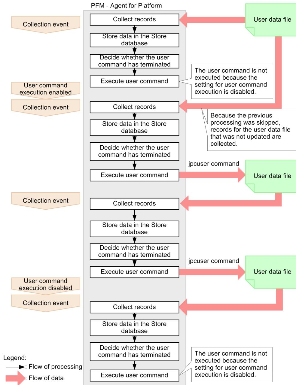
Figure 6–2: Flow of processing for functionality for periodically executing user commands
