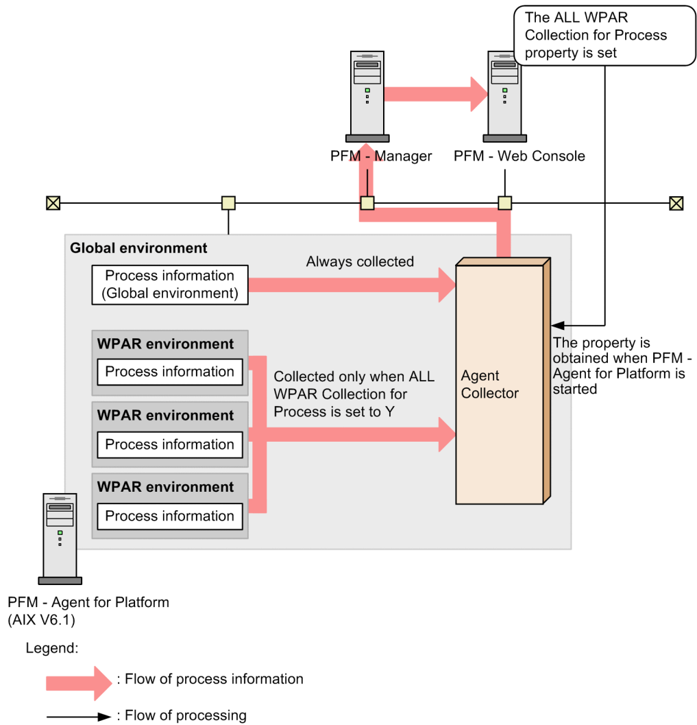
Figure 2-14: Process information collected for the global environment
