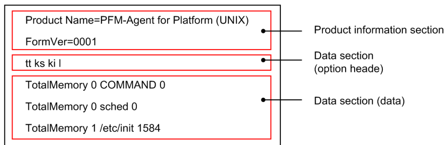
Figure 6–4: Example configuration of user-created data
