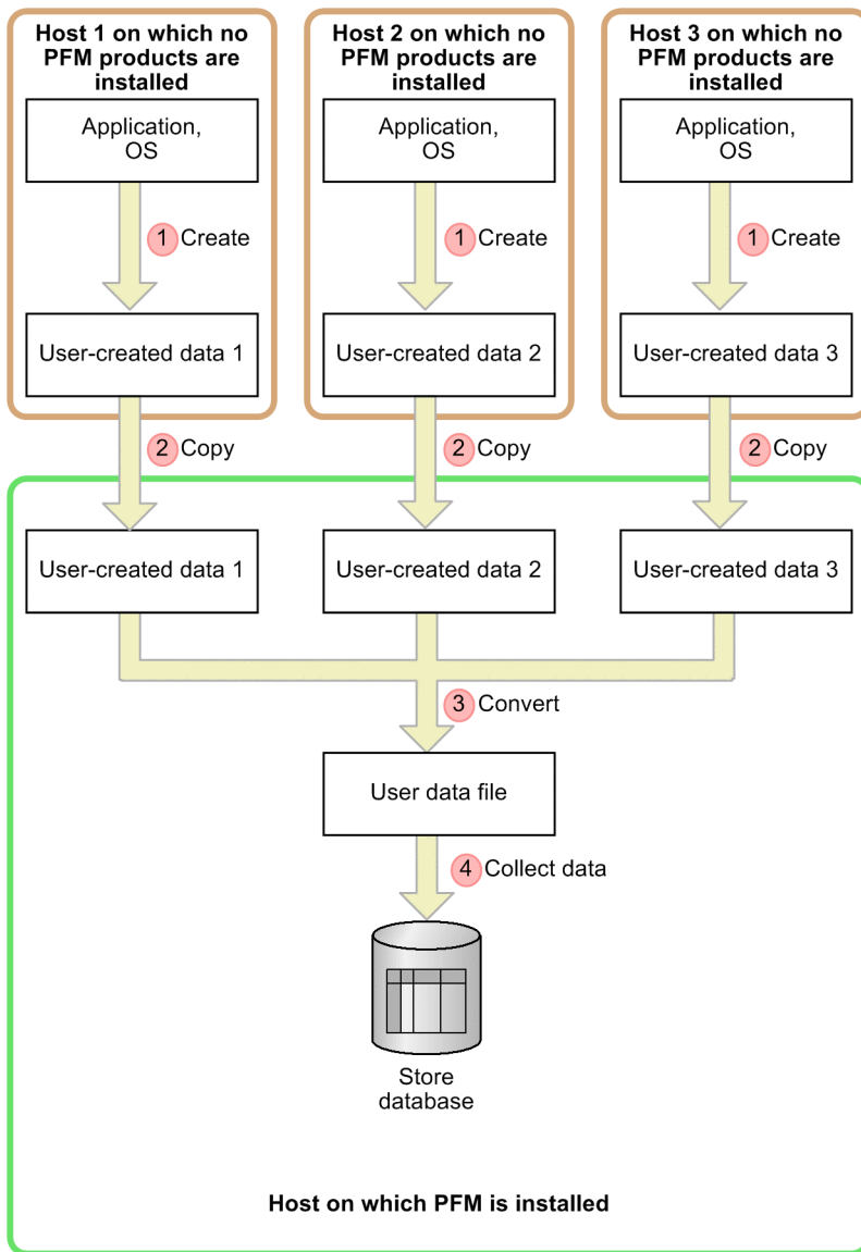
Figure 3–5: Flow of data collection for hosts on which PFM products are not installed
