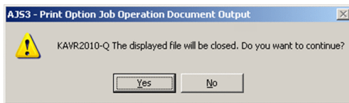
Figure 7–26: Close window
