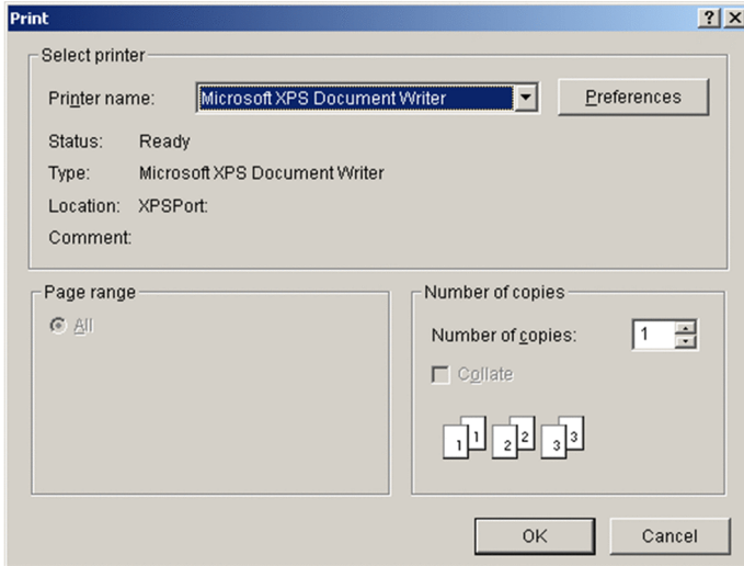
Figure 7–25: Print window
