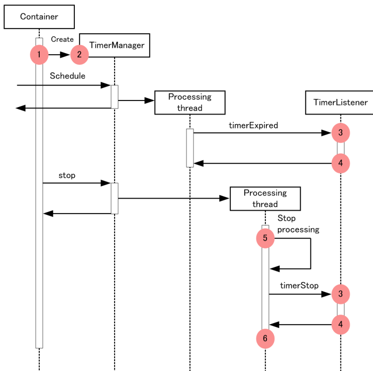
Figure 8-50: Trace collection points of TimerManager
