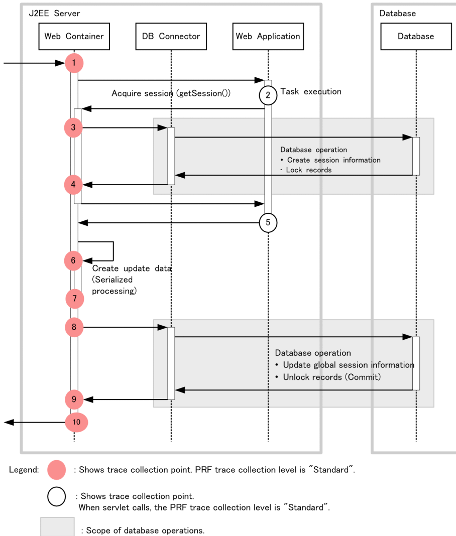
Figure 8-15: Trace collection points of the request processing for creating an HTTP session (database session failover functionality)
