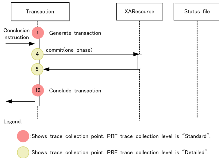
Figure 8-64: Trace collection points in a typical one-phase commit model
