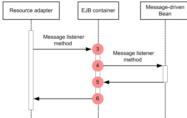
Figure 8-26: Trace collection points of a Message-driven Bean (EJB2.1 and later) (in the case of optionA#)
