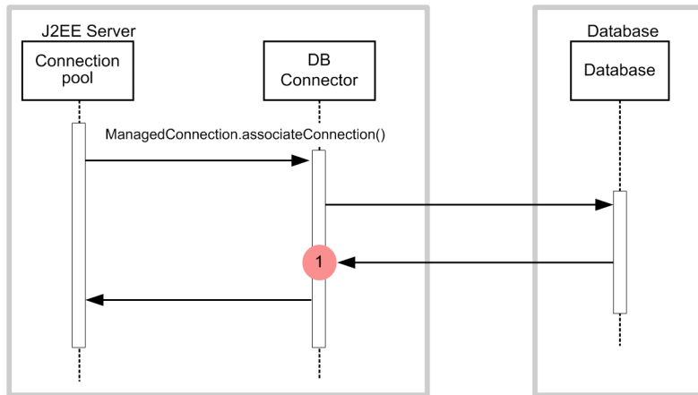
Figure 8-54: Details of trace collection points in a DB Connector and JCA container (connection association-related)
