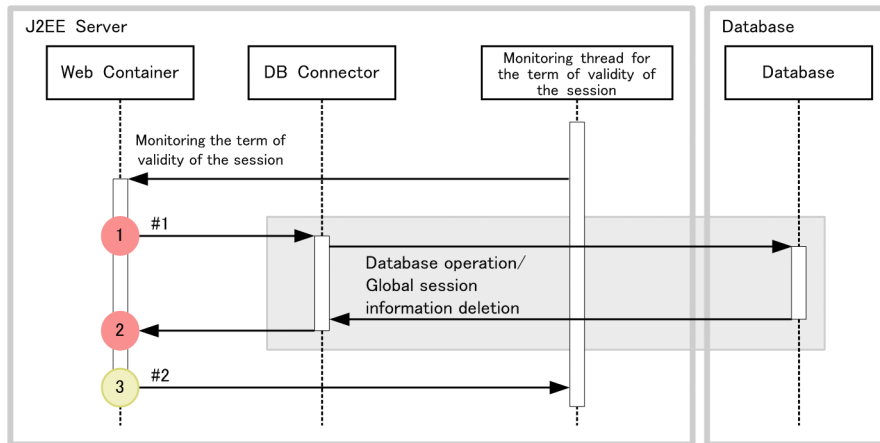
Figure 8-18: Trace collection points of the request processing for disabling an HTTP session through valid period monitoring (database session failover functionality)
