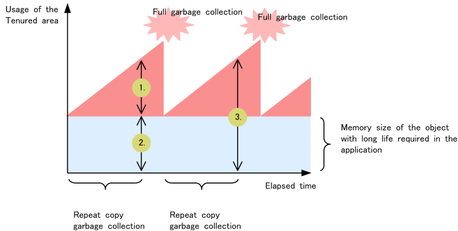
Figure 9-10: Contents that can be identified using the unused objects statistical functionality in the Tenured area and the instance statistical functionality
