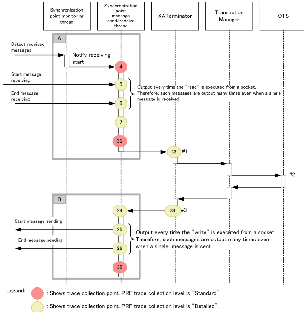
Figure 8-89: Overview of the trace collection points in the synchronous point processing
