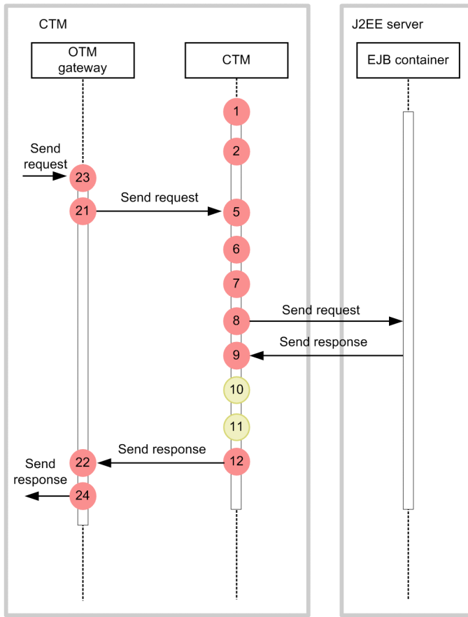
Figure 8-7: Trace collection points of a CTM (when using the OTM gateway)
