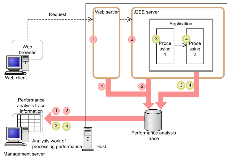
Figure 7-1: Overview of the trace based performance analysis
