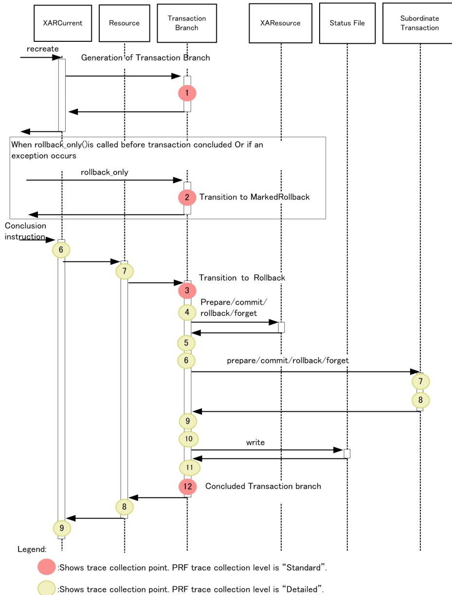
Figure 8-66: PRF acquisition information during transaction linkage with OpenTP1
