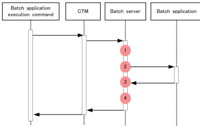
Figure 8-70: Trace collection points in the batch application execution functionality
