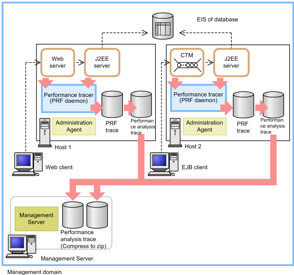
Figure 7-2: Overview of trace information collection of trace based performance analysis
