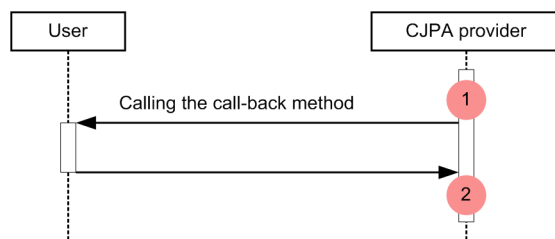
Figure 8-82: Trace collection points of the callback method to the user
