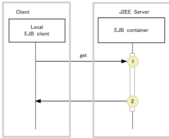
Figure 8-36: Trace collection points when get is invoked from the local client
