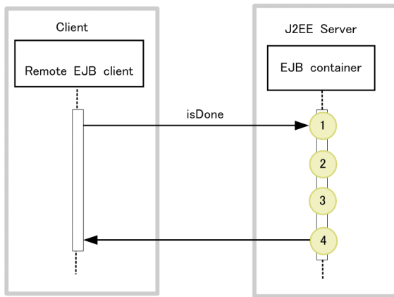
Figure 8-39: Trace collection points when isDone is invoked from the remote client
