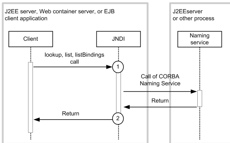
Figure 8-45: Trace collection points of a JNDI
