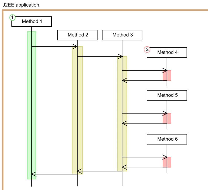
Figure 7-16: Method invocation relationship in an application
