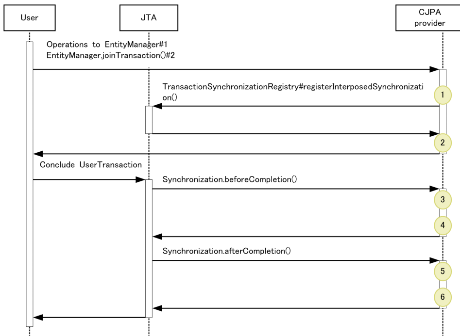
Figure 8-84: Trace collection points during transaction linkage with the transaction manager
