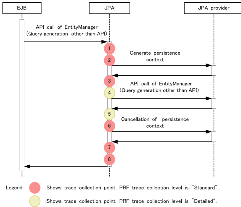
Figure 8-73: Trace collection points when the entity manager related to the persistent context of the transaction scope is used outside a transaction
