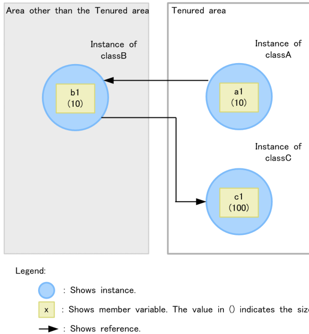
Figure 9-13: Example of reference relationship (Objects for which the statistics are not to be collected)
