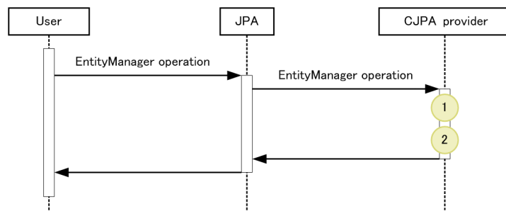
Figure 8-78: Trace collection points for javax.persistence.EntityManager
