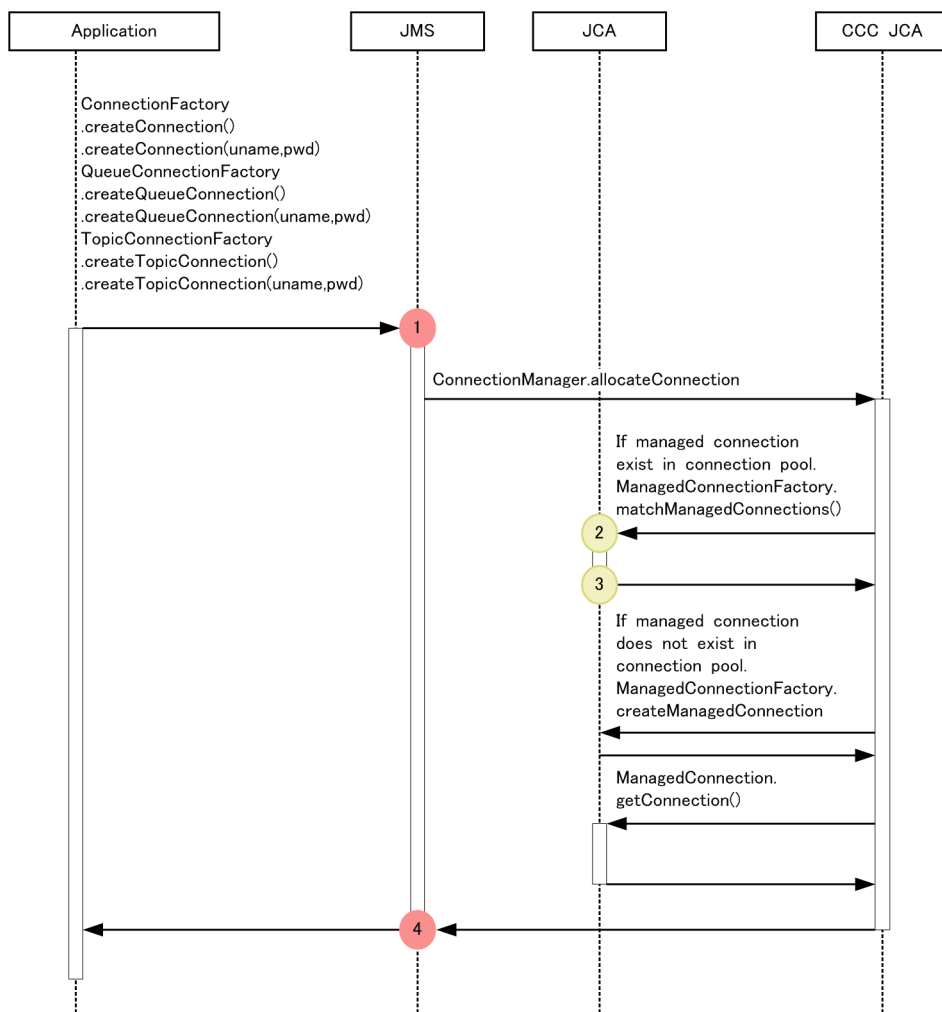
Figure 8-93: Trace collection points in JMS ConnectionFactory interface
