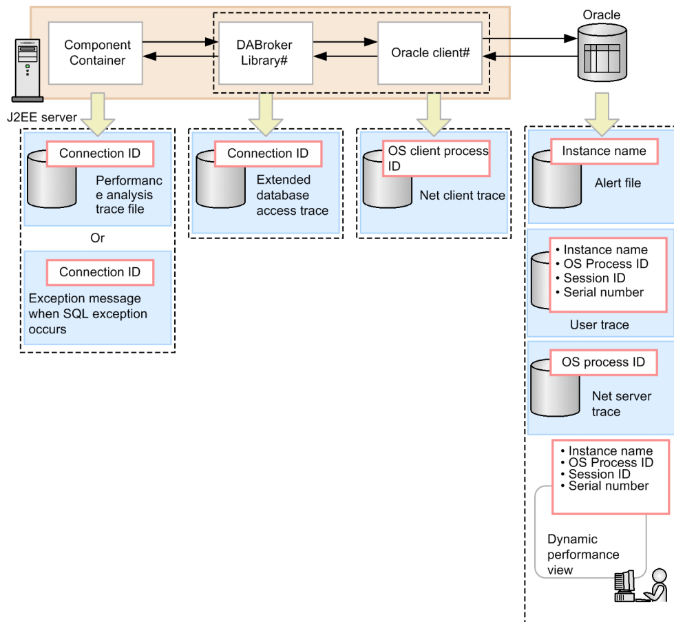
Figure B-2: Output overview of Connection ID (In Oracle)
