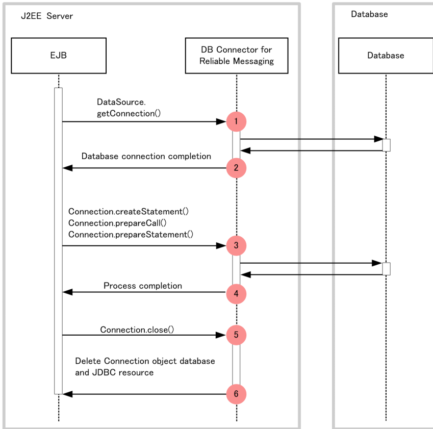
Figure 8-56: Details of trace collection points in a DB Connector and JCA container (during linkage with the DB Connector for Cosminexus RM)
