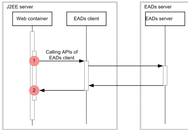
Figure 8-22: Trace collection points when an EADs client is invoked (EADs session failover functionality)
