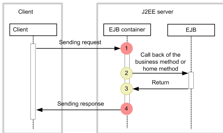
Figure 8-24: Trace collection points of a Session Bean or Entity Bean
