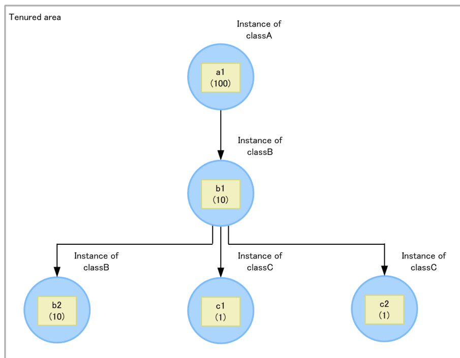
Figure 9-15: Example of the reference relationship based on the unused objects within the Tenured area
