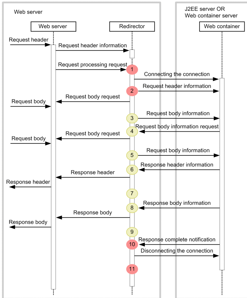
Figure 8-9: Trace collection points of a redirector
