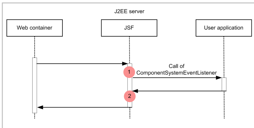
Figure 8-114: Trace collection points when ComponentSystemEventListener is invoked
