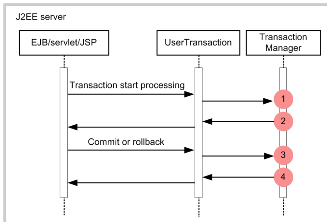
Figure 8-48: Trace collection points when UserTransaction is used
