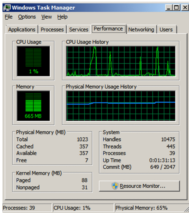
Figure 6-8: CPU usage
