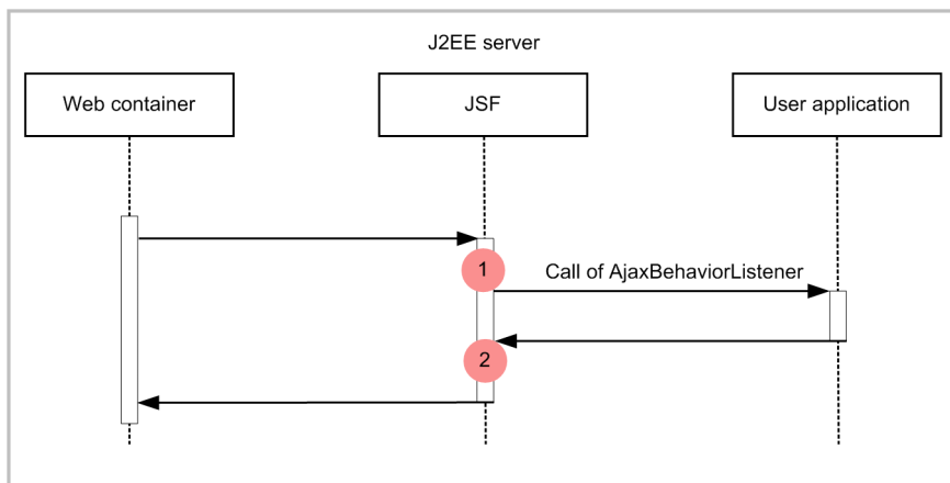
Figure 8-112: Trace collection points when AjaxBehaviorListener is invoked
