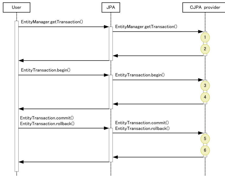
Figure 8-81: Trace collection points for the operation of EntityTransaction
