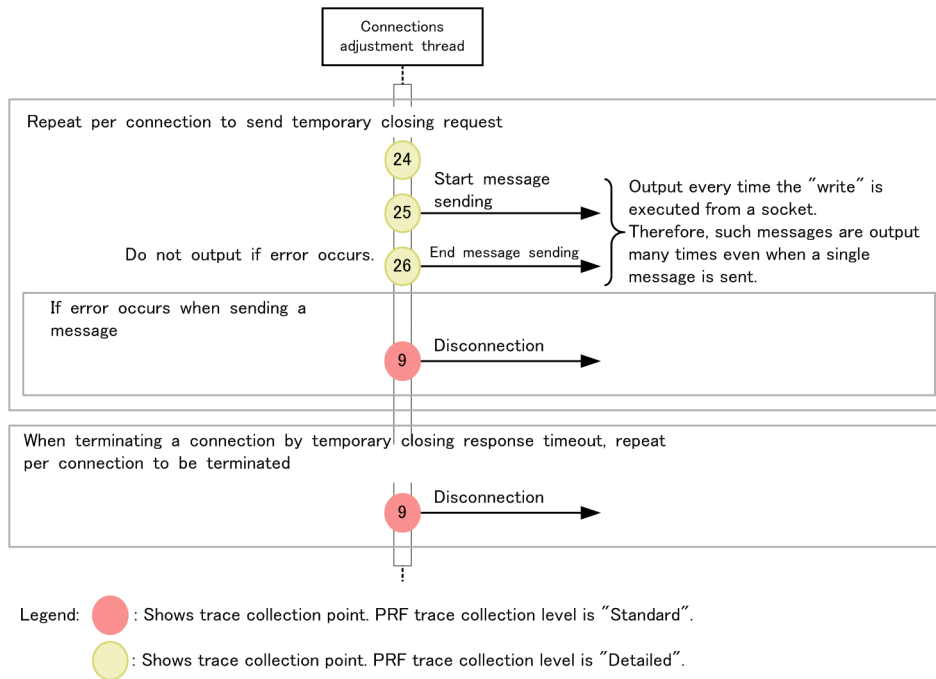
Figure 8-92: Trace collection points for the connection count adjustment thread
