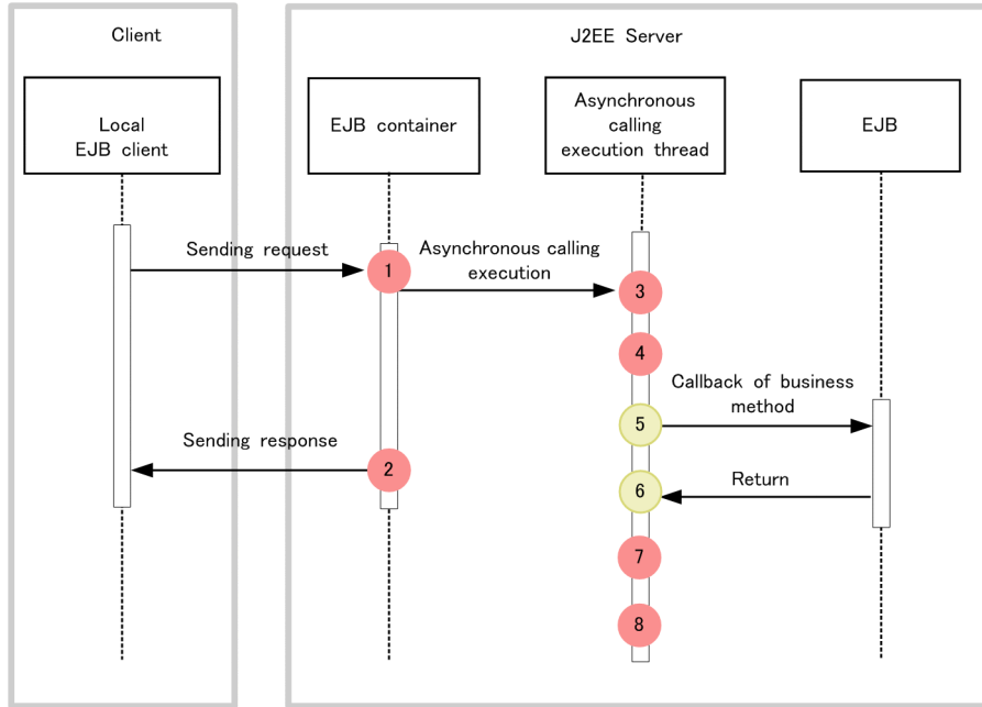
Figure 8-34: Trace collection points when the Session Bean is invoked asynchronously from the local client
