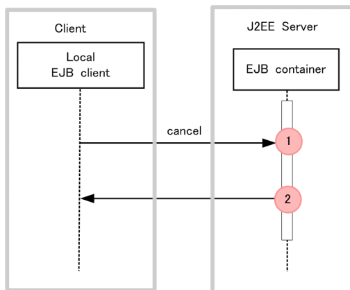
Figure 8-42: Trace collection points when cancel is invoked from the local client
