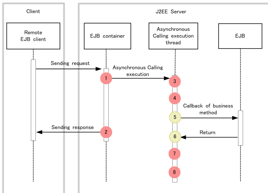
Figure 8-35: Trace collection points when the Session Bean is invoked asynchronously from the remote client
