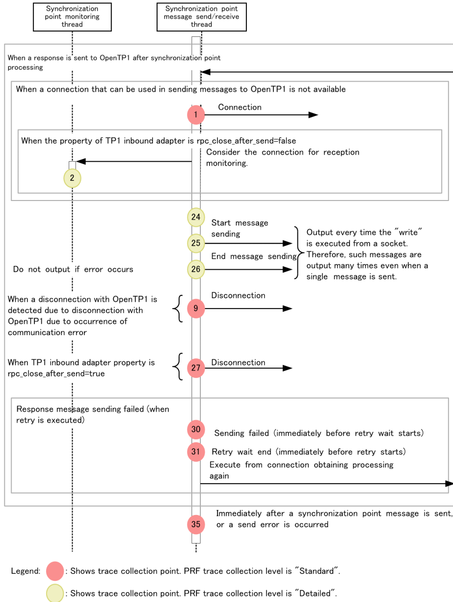
Figure 8-91: Trace collection point of the B part in the synchronous point processing
