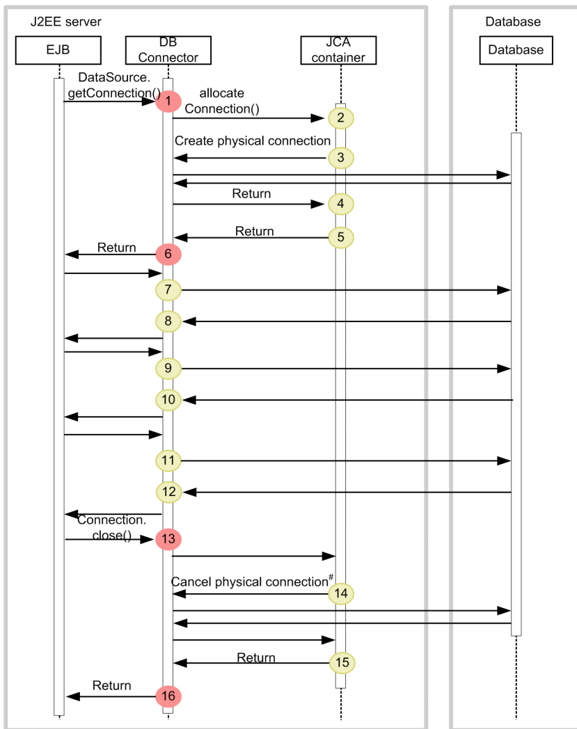
Figure 8-52: Trace collection points in a DB Connector and JCA container (connection-related)
