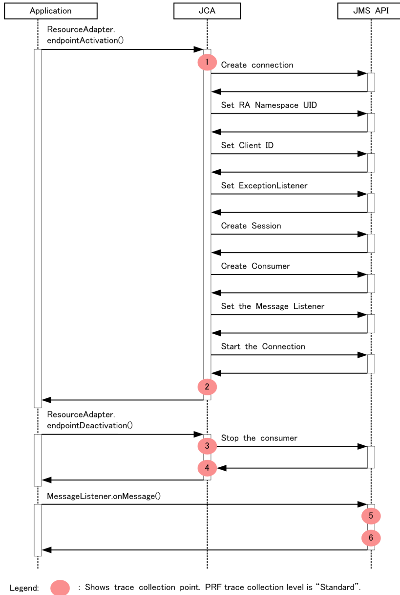
Figure 8-100: Trace collection points when Message-driven Bean is deployed from the CJMSP resource adapter
