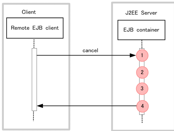
Figure 8-43: Trace collection points when cancel is invoked from the remote client
