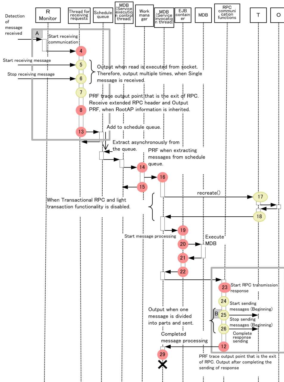
Figure 8-86: Overall trace collection points in the TP1 inbound integrated function
