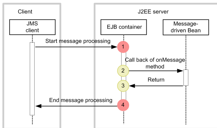
Figure 8-25: Trace collection points of a Message-driven Bean (EJB2.0)
