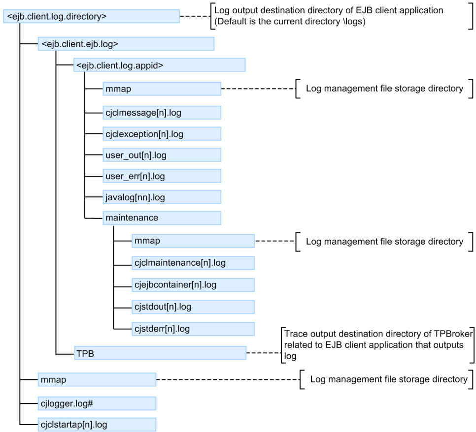
Figure 4 - 1: Output destination of the EJB client application system log in the subdirectory shared mode (When specified in the option definition file for Java applications)
