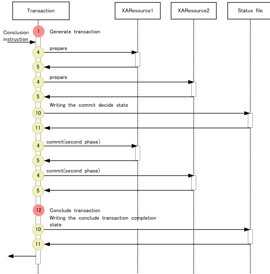
Figure 8-65: Trace collection points in a typical two-phase commit model
