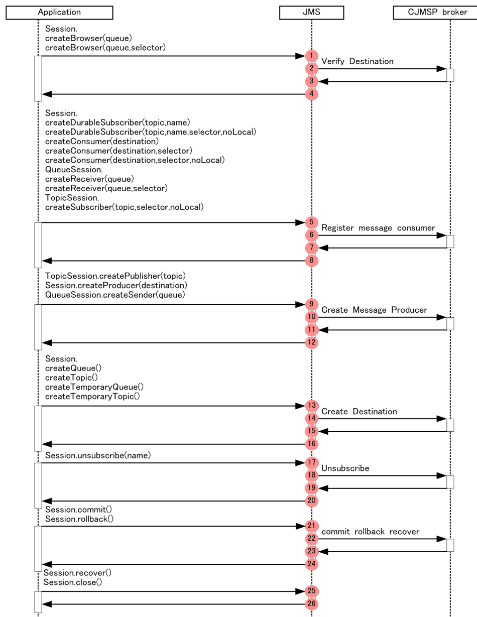
Figure 8-95: Trace collection points in the JMS session interface
