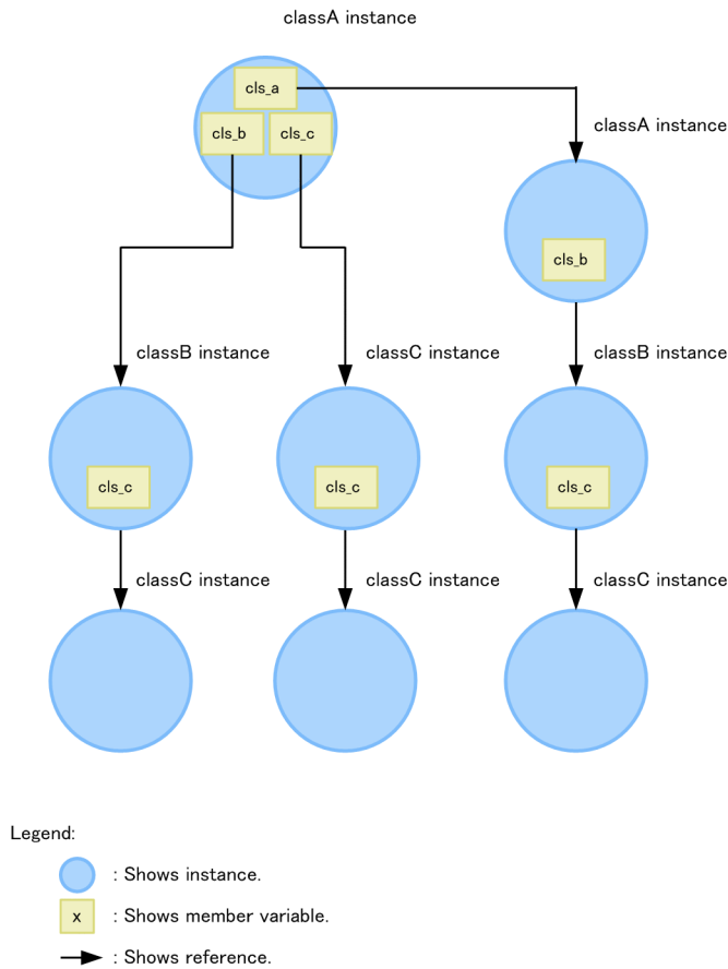
Figure 9-6: Instance structure (reference-related information output functionality)
