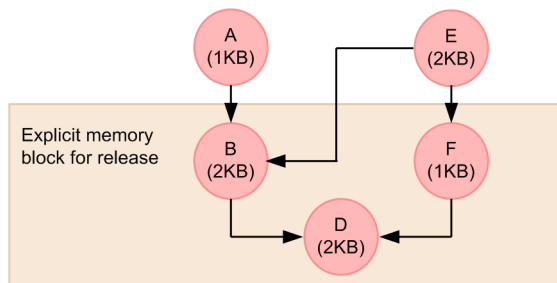
Figure 5-9: Example where there are multiple reference routes to object moving to Java heap
