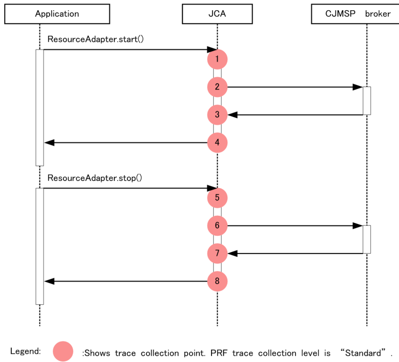
Figure 8-97: Trace collection points of CJMSP Broker when connecting to the CJMSP resource adapter
