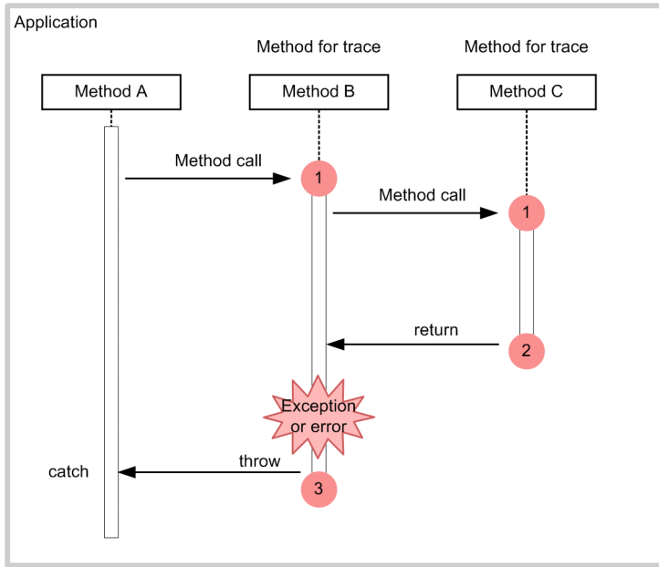
Figure 8-119: Trace collection points of the user-extended trace based performance analysis
