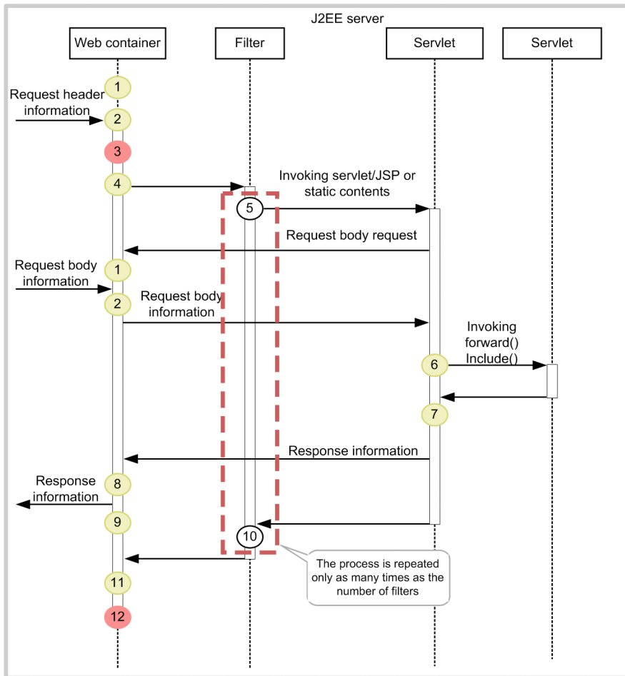
Figure 8-11: Trace collection points of an in-process HTTP server
