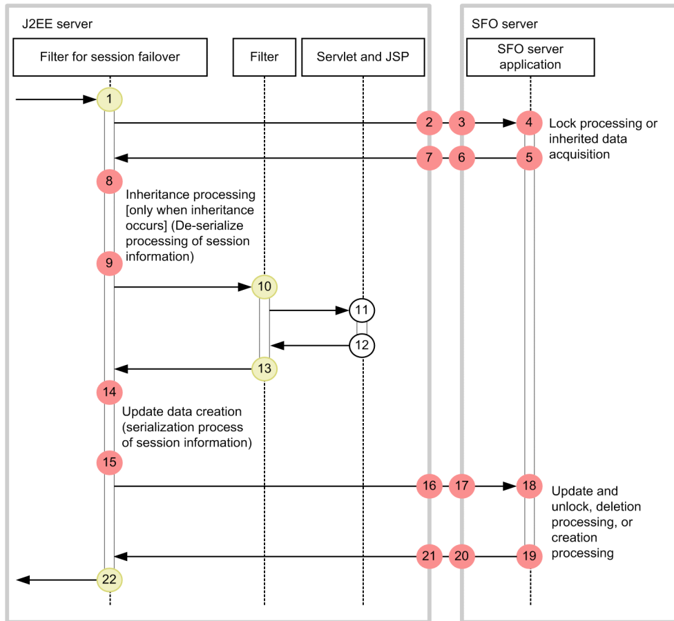
Figure 8-23: Trace collection points in a Web container (memory session failover functionality)
