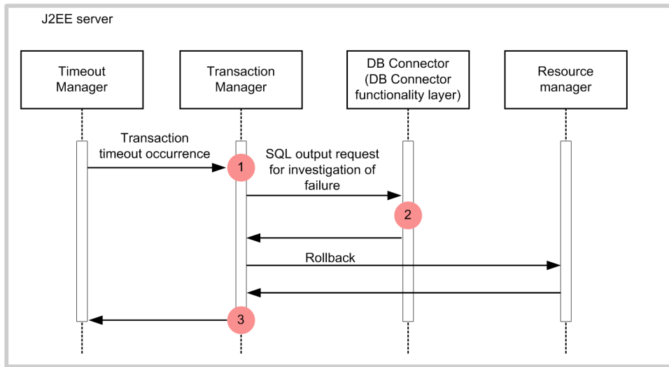
Figure 8-49: Trace collection points in the case of a transaction timeout
