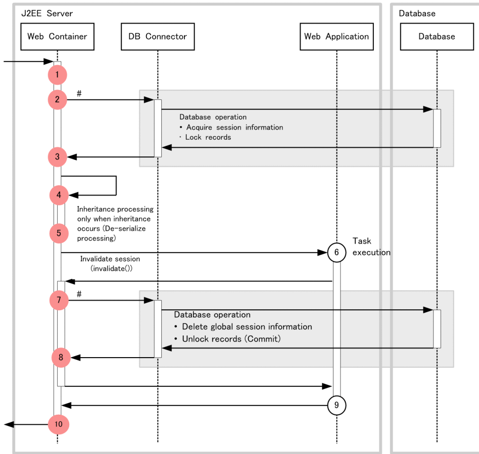
Figure 8-17: Trace collection points of the request processing for disabling an HTTP session (database session failover functionality)
