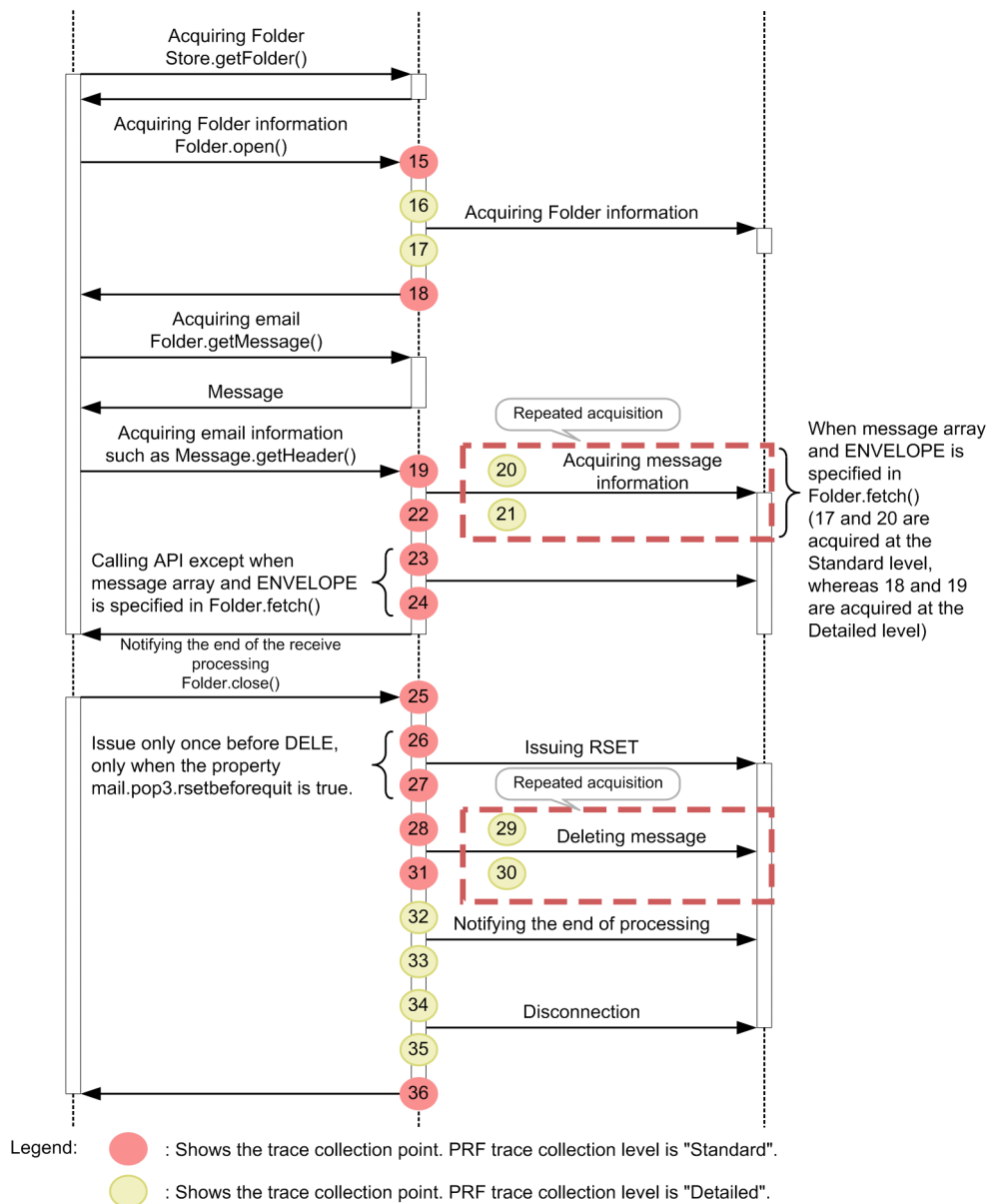
Figure 8-105: Trace collection point on confirming the JavaMail connection
