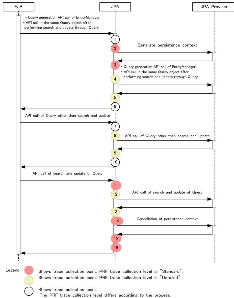
Figure 8-74: Trace collection points when a Query generated outside a transaction is used outside the transaction
