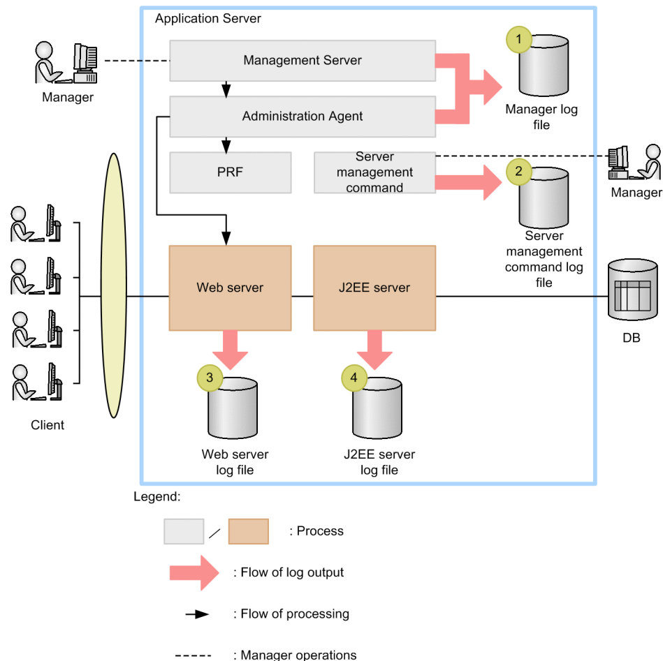
Figure 6-1: Processes that output logs
