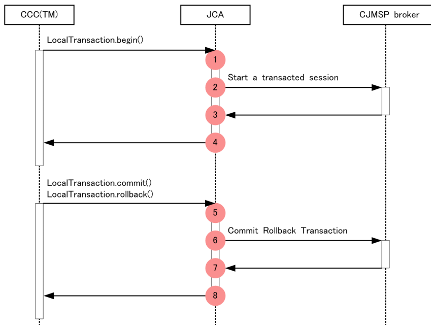
Figure 8-98: Trace collection points of the transaction management in the CJMSP resource adapter (for LocalTransaction )
