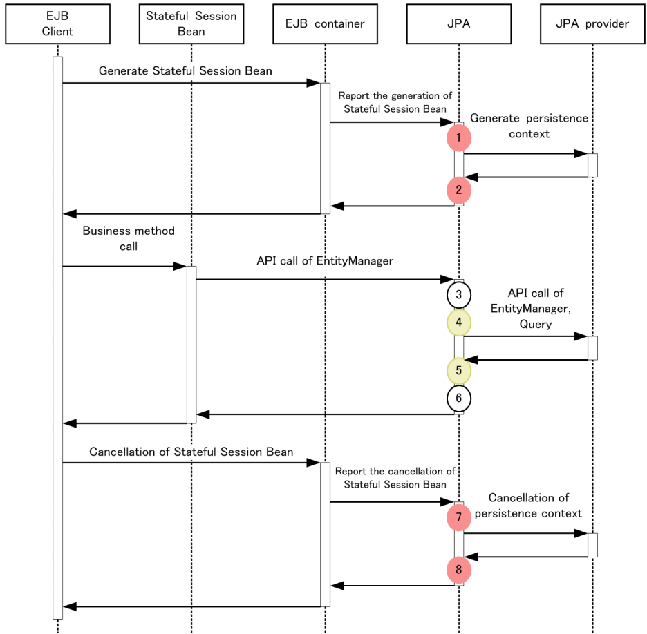
Figure 8-75: Trace collection points when an extended persistent context is used
