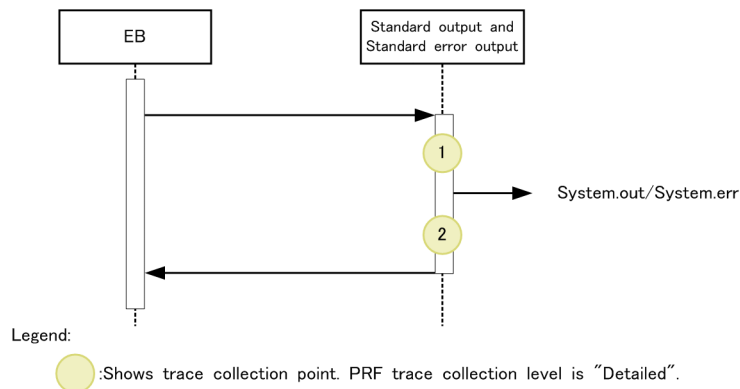
Figure 8-67: Trace collection points of standard output or standard error output
