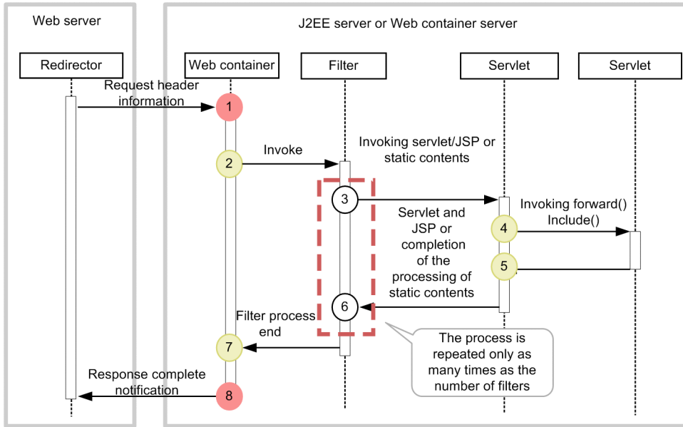
Figure 8-10: Trace collection points of a Web container (trace of request processing)
