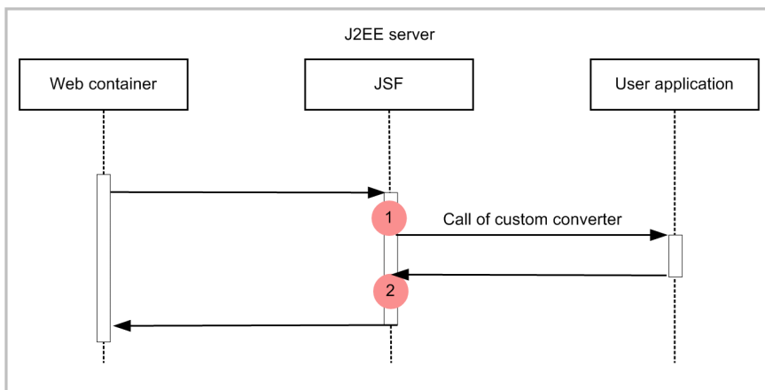
Figure 8-108: Trace collection points when a custom converter is invoked
