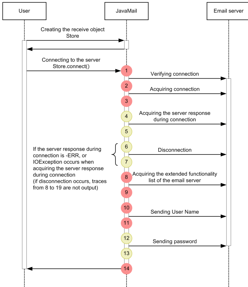
Figure 8-104: Trace collection points on JavaMail receipt
