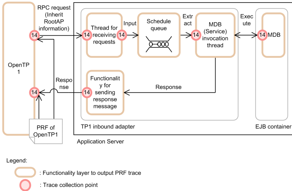
Figure 8-4: Functionality layers and trace collection points (In the TP1 inbound integrated function)
