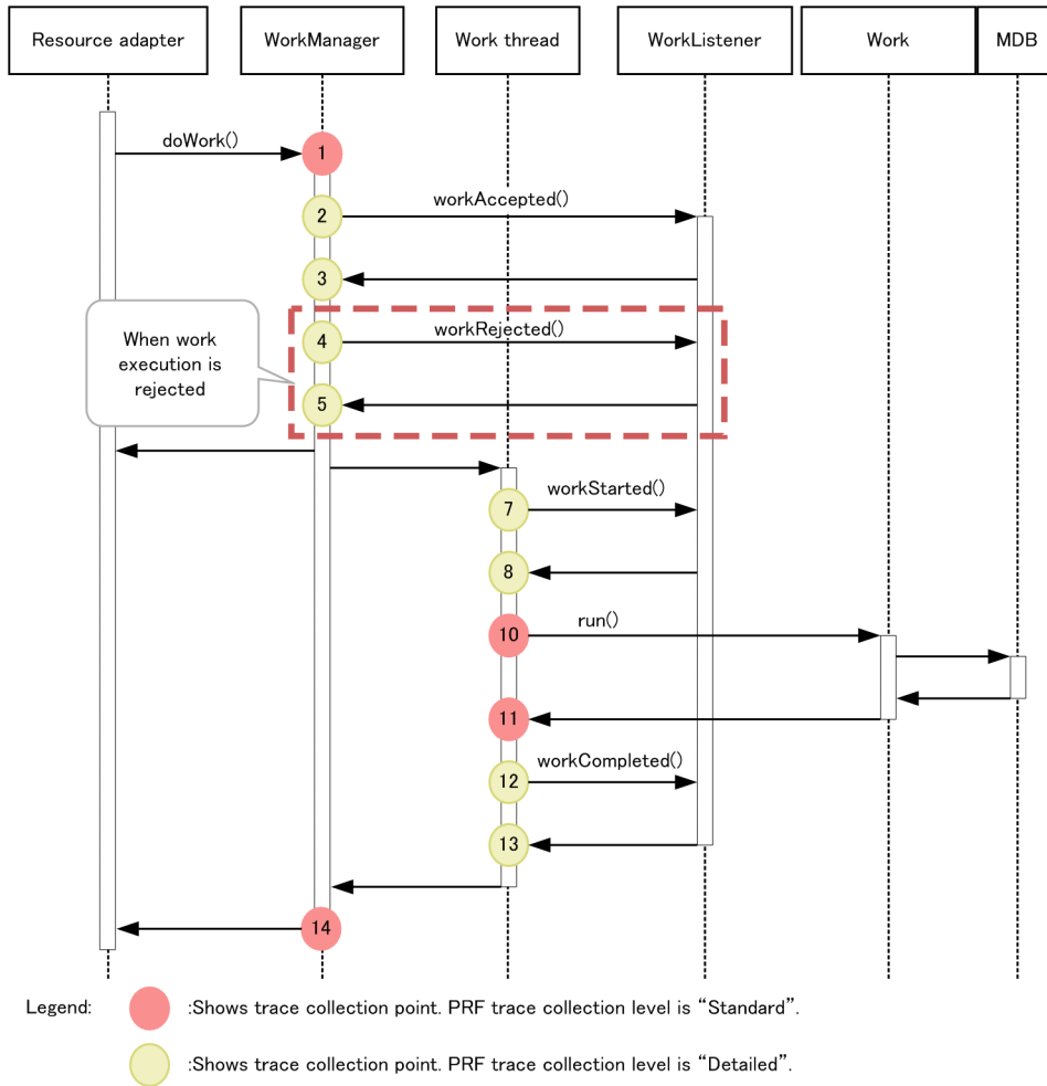
Figure 8-59: Details of trace collection points in a DB Connector and JCA container (when doWork() is invoked)
