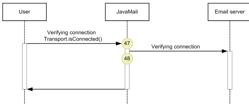
Figure 8-103: Trace collection point on confirming the JavaMail connection
