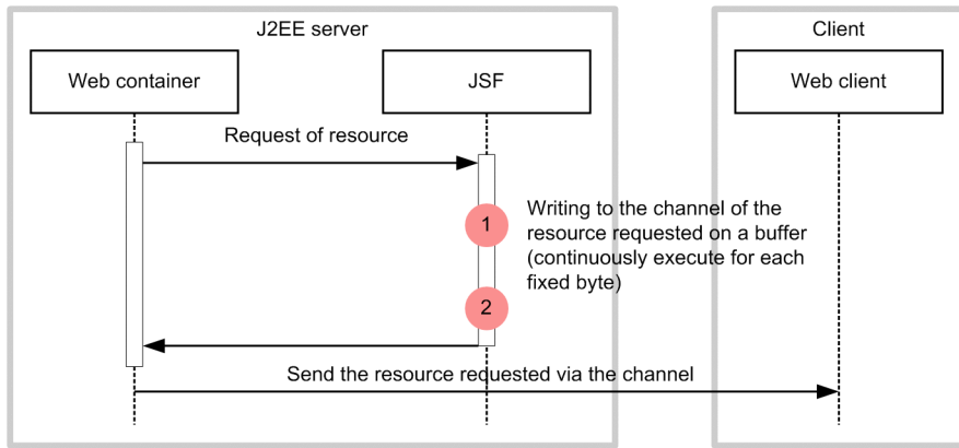
Figure 8-115: Trace collection points in resource handling
