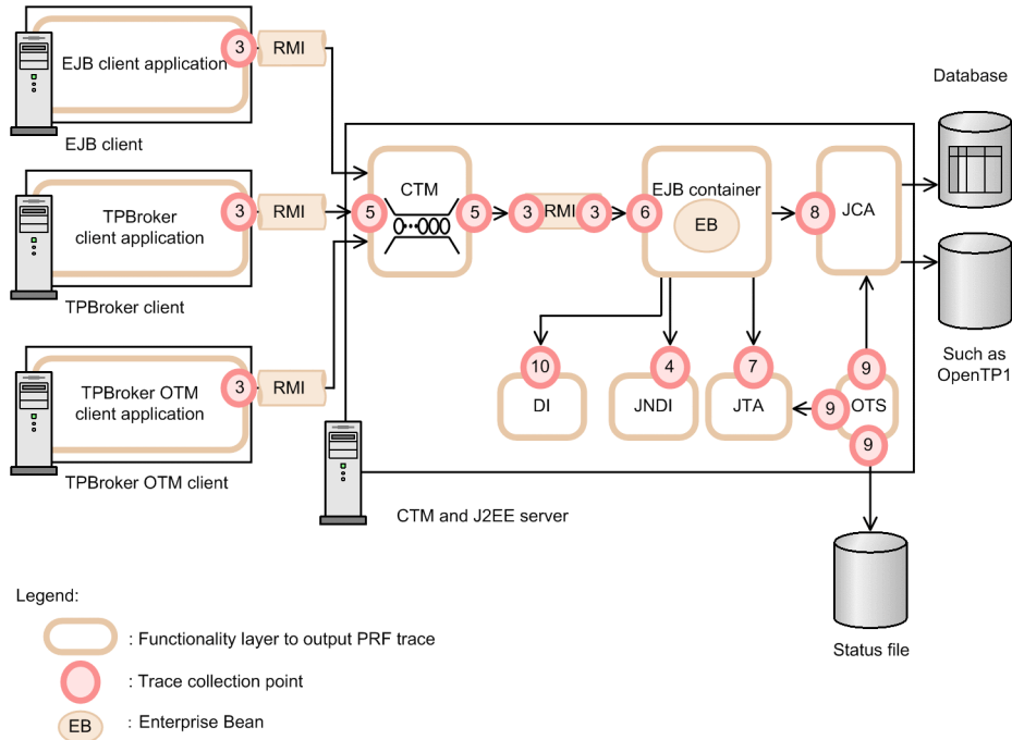
Figure 8-4: Functionality layers and trace collection points (In the TP1 inbound integrated function)
