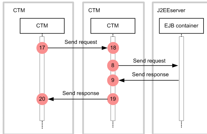
Figure 8-6: Trace collection points of a CTM (For linkage with another CTM)
