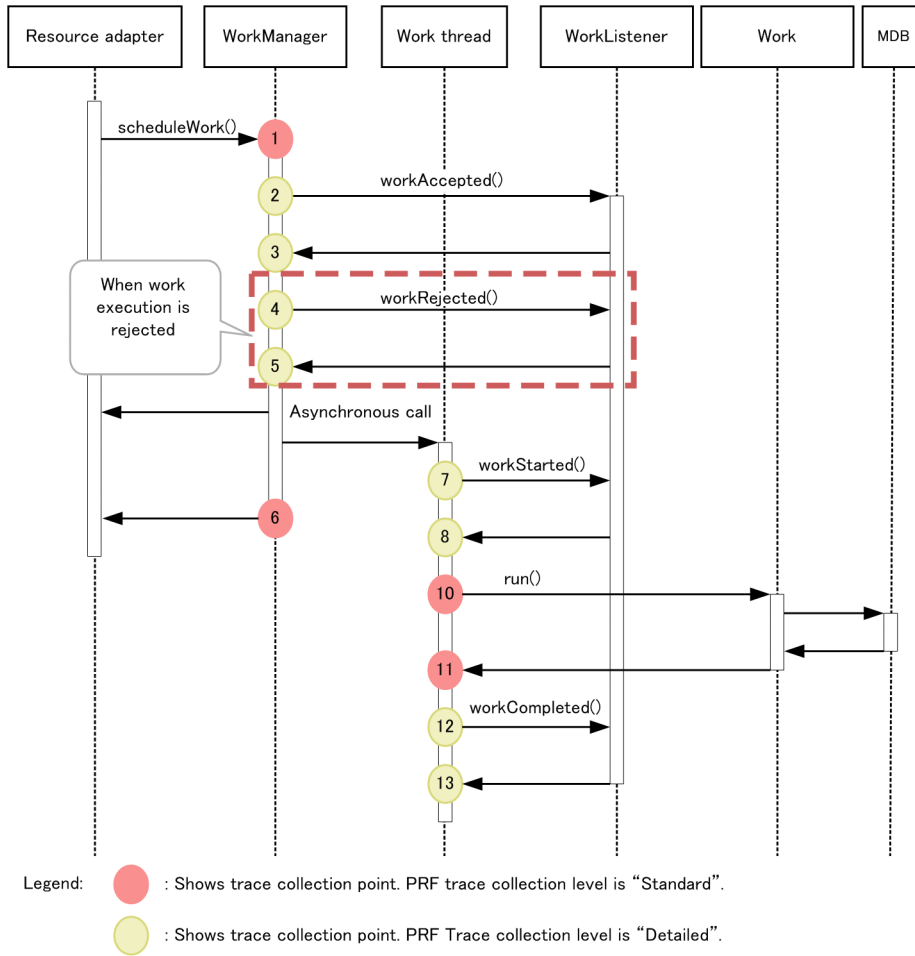
Figure 8-57: Details of trace collection points in a DB Connector and JCA container (when scheduleWork() is invoked)
