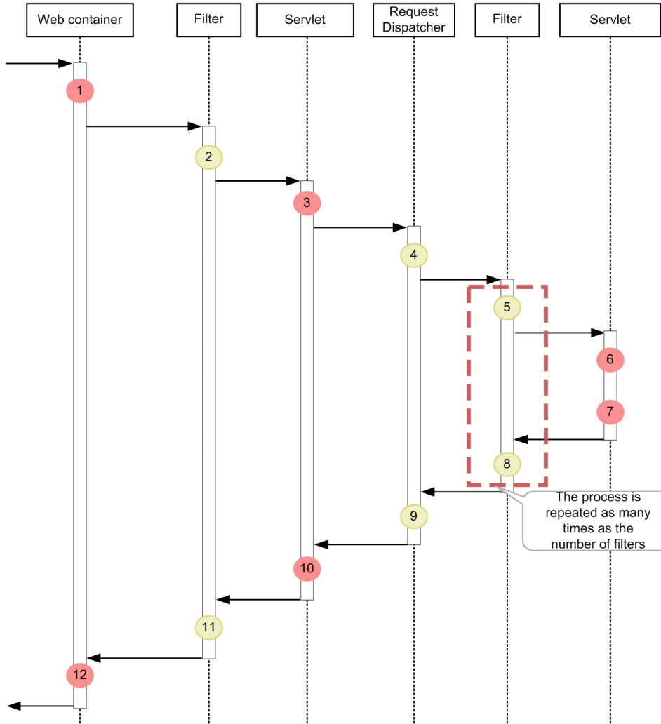
Figure 8-13: Trace collection points in a Web container during normal termination (filter trace)
