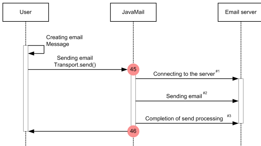
Figure 8-102: Trace collection points on JavaMail transmission (when the send(Message msg, Address[] addresses) method and send(Message msg) method of the javax.mail.Transport class are used)
