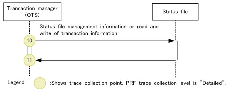
Figure 8-62: Trace collection points related to reading or writing into the status file during the in-process OTS initialization
