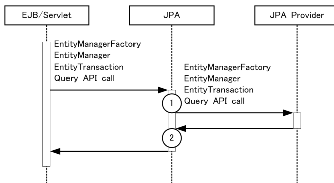
Figure 8-71: Trace collection points when the persistent context of application management is used
