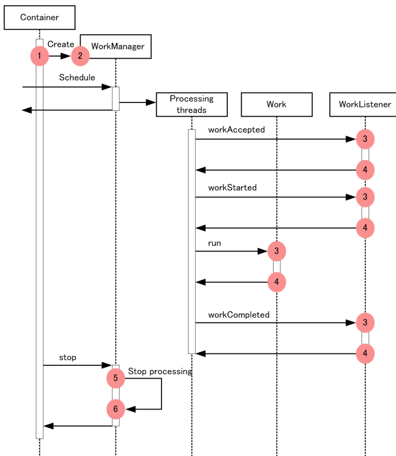
Figure 8-51: Trace collection points of WorkManager
