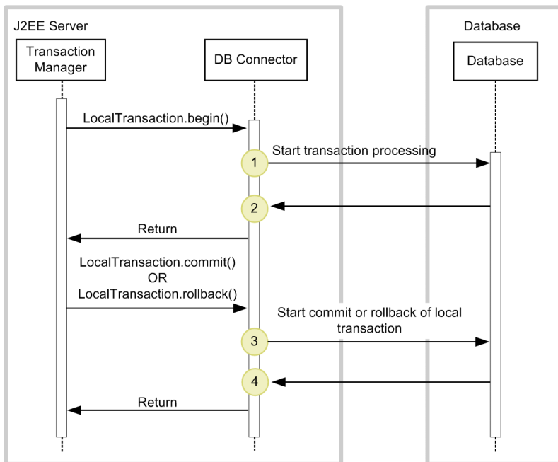
Figure 8-53: Details of trace collection points in a DB Connector and JCA container (local transaction-related)
