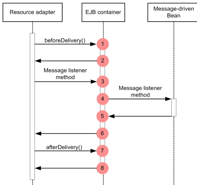
Figure 8-27: Trace collection points of a Message-driven Bean (EJB2.1 and later) (in the case of optionB#)
