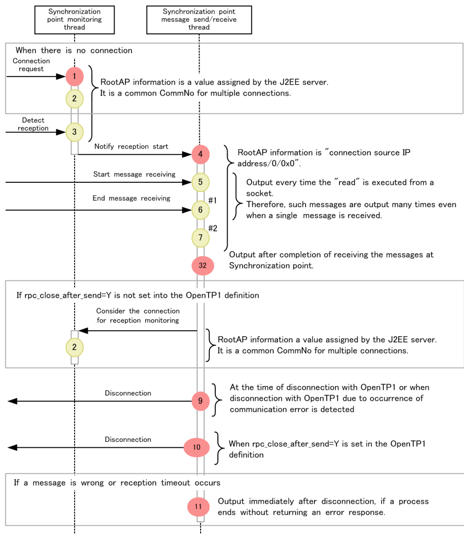
Figure 8-90: Trace collection point of the A part in the synchronous point processing
