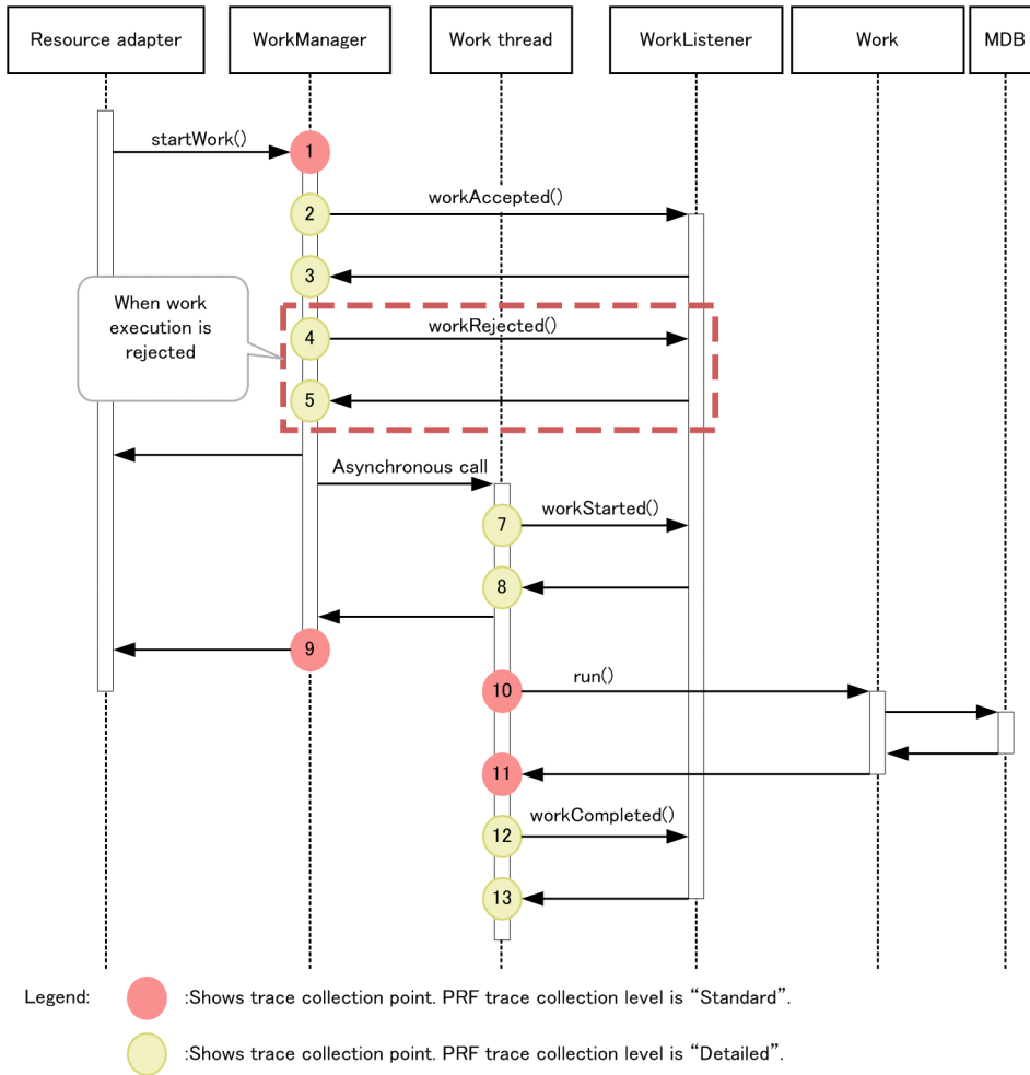
Figure 8-58: Details of trace collection points in a DB Connector and JCA container (when startWork() is invoked)
