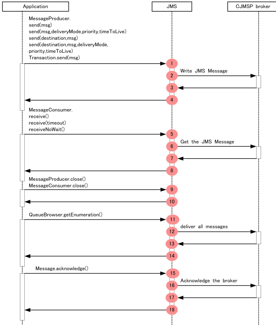
Figure 8-96: Trace collection points of the JMS messages, producer, consumer, and queue browser
