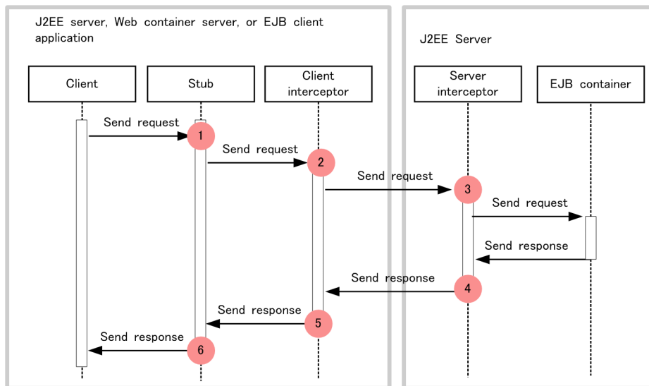
Figure 8-60: Trace collection points of an RMI
