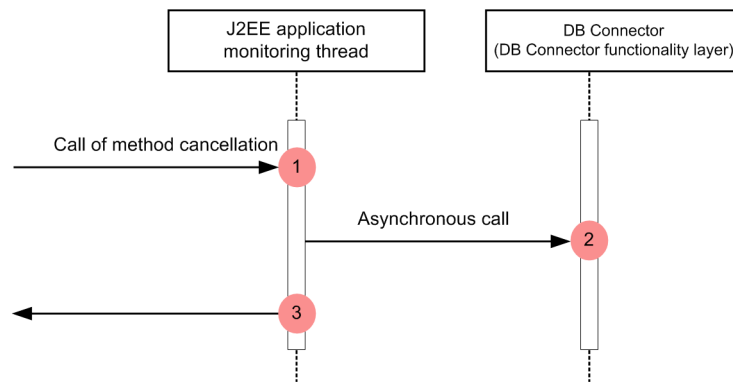
Figure 8-44: Trace collection points when method cancellation occurs
