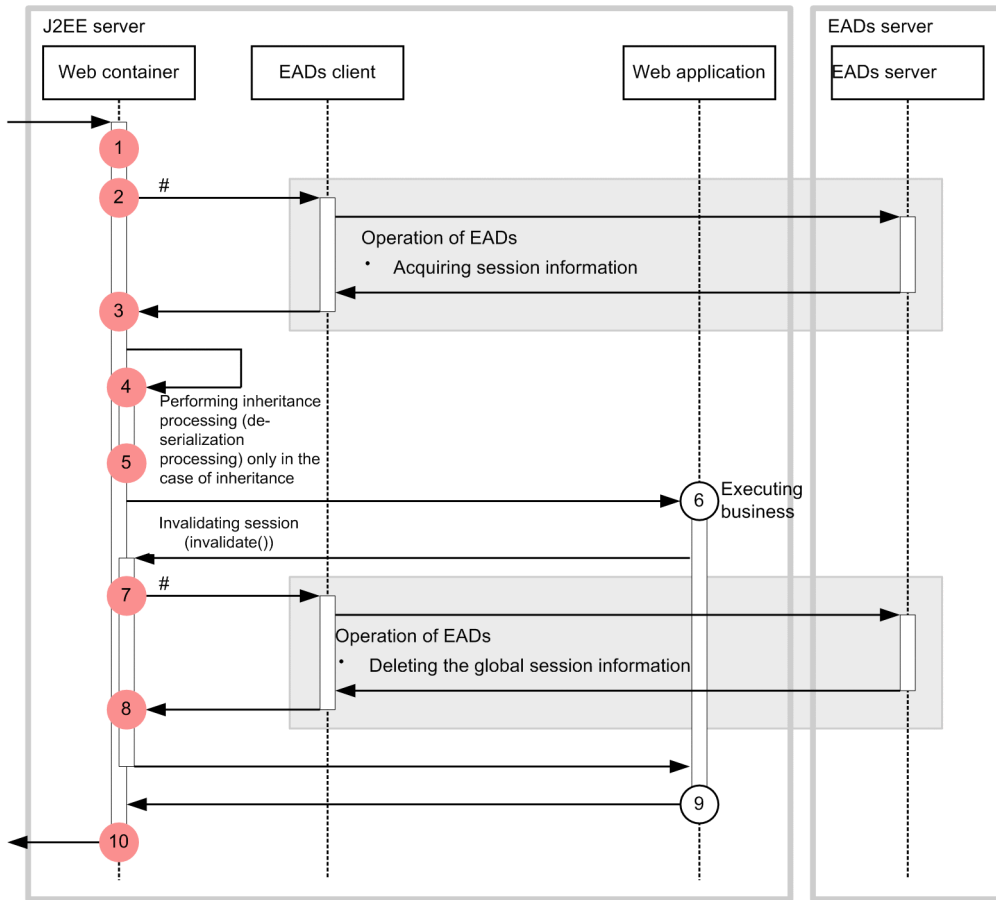
Figure 8-21: Trace collection points during request processing for disabling an HTTP session (EADs session failover functionality)
