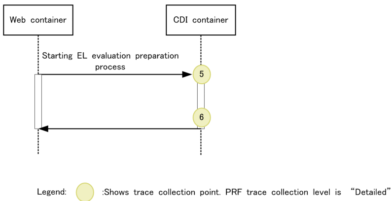
Figure 8-117: Trace collection points when a combination of JSF and CDI is used (for EL evaluation)
