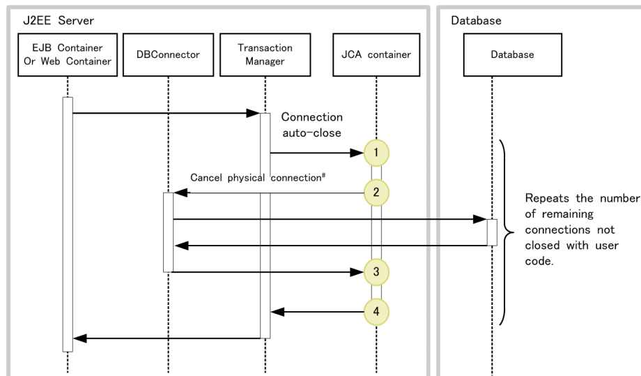
Figure 8-55: Details of trace collection points in a DB Connector and JCA container (when the connection closes automatically)
