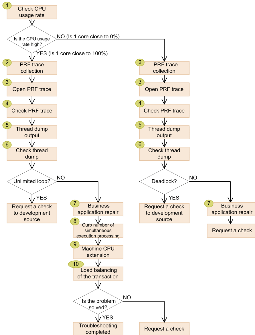
Figure 6-7: Flow of actions when a response is delayed
