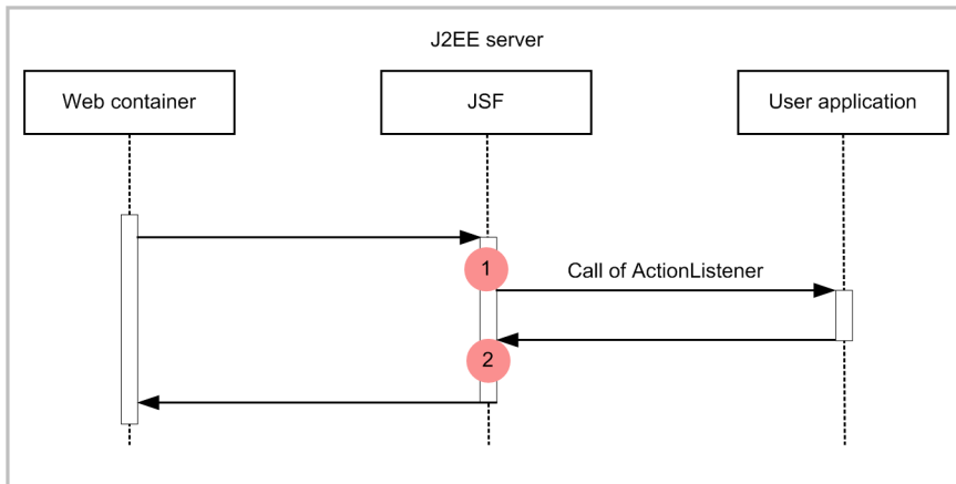
Figure 8-111: Trace collection points when ActionListener is invoked
