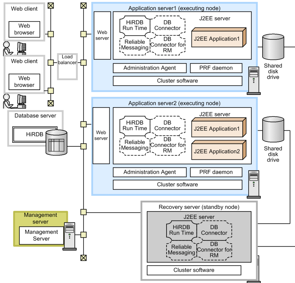
Figure 3-59: Example of system configuration of N-to-1 recovery system (when configuration of J2EE applications differ and all resource adapters are identical for N executing node machines)
