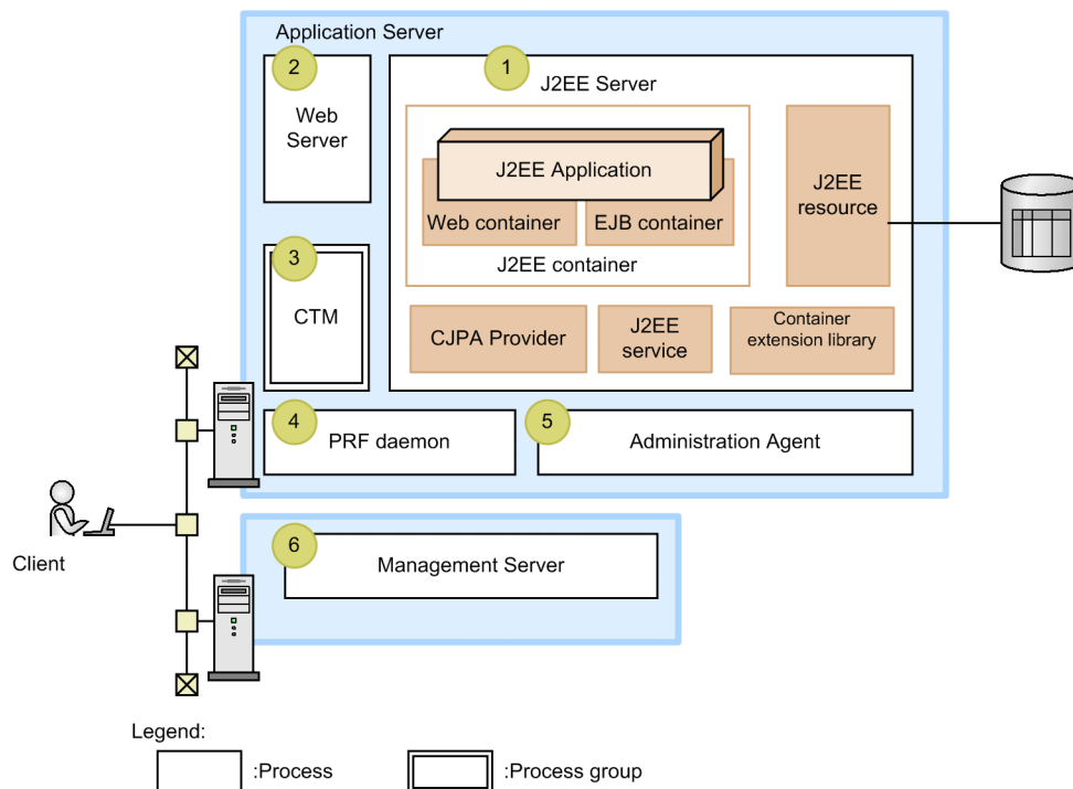
Figure 2-1: Processes that configure Application Server for executing J2EE applications
