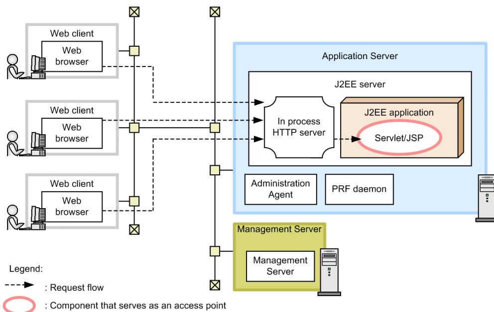
Figure 3-29: Example of Web client configuration built on one Application Server machine (for using in-process HTTP server)
