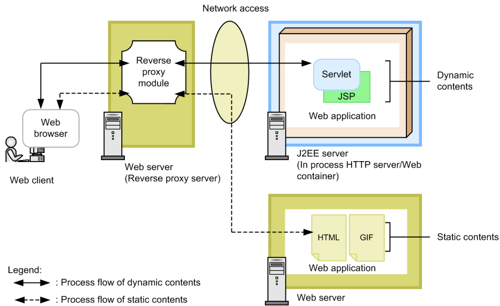
Figure 8-19: Image showing the distribution of dynamic and static contents by the reverse proxy server
