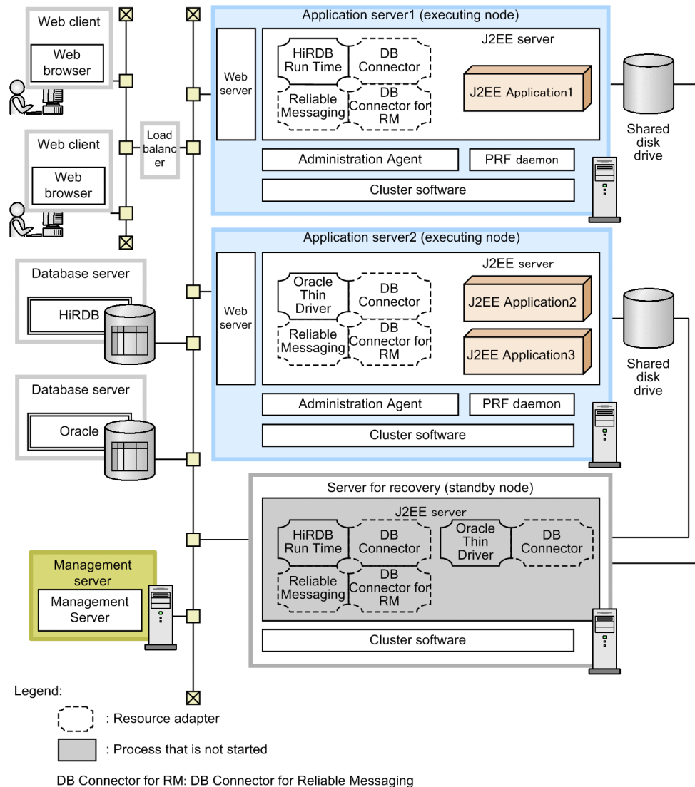
Figure 3-60: Example of system configuration of N-to-1 recovery system (when configuration of J2EE applications and resource adapters differ for N executing node machines)
