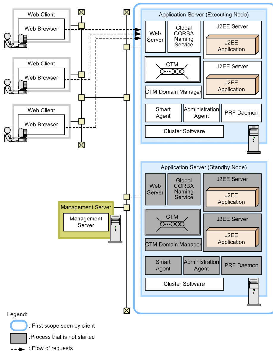
Figure 3-54: Example of system configuration where executing node and standby node are in 1-to-1 ratio and cluster software is used (when transaction service is not used)
