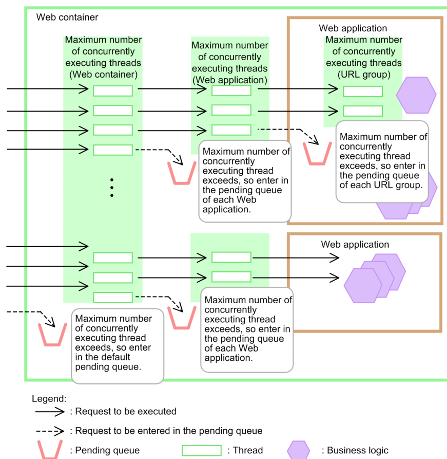
Figure 8-4: Relationship between concurrently executed threads of each Web container, Web application, and URL group
