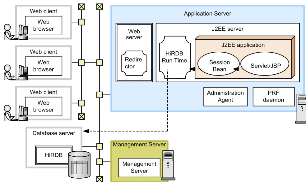
Figure 3-34: Example configuration when using a local transaction
