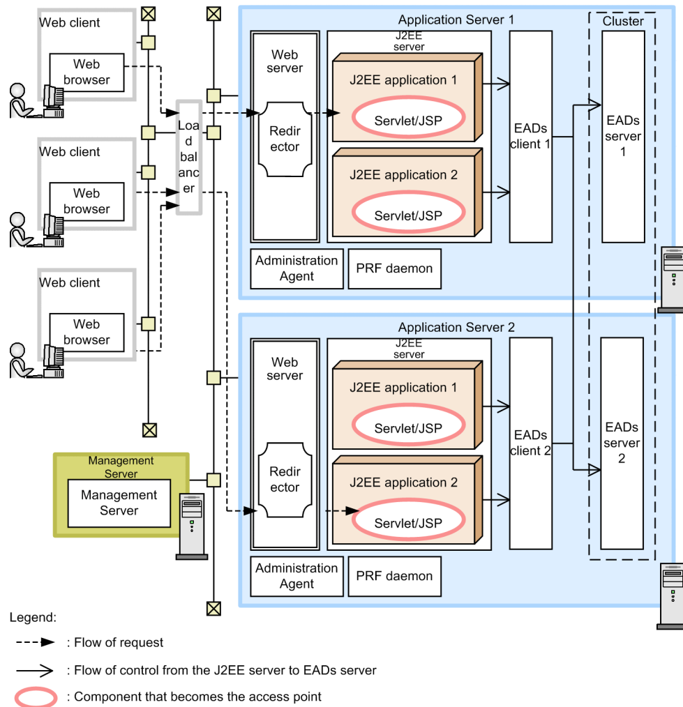
Figure 3-50: Example configuration for using an EADs server allocated to the same computer as the J2EE server and inheriting the session information
