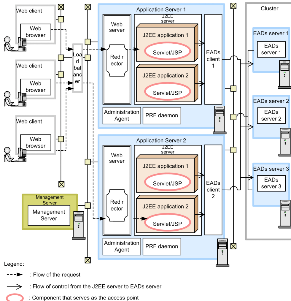
Figure 3-49: Example of a configuration using an EADs server allocated to a computer different from the J2EE server and inheriting the session information
