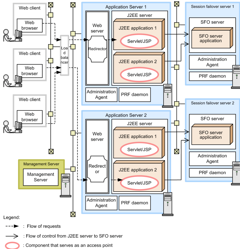
Figure 3-51: Example configuration when multiple SFO servers exist in a system
