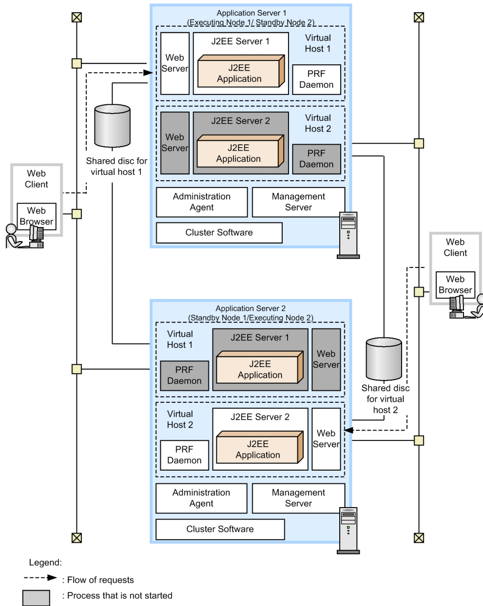
Figure 3-57: Example of the configuration of mutual node switching system (for using transaction service)
