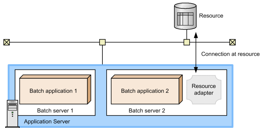
Figure 4-1: Example of a system configuration for executing batch applications
