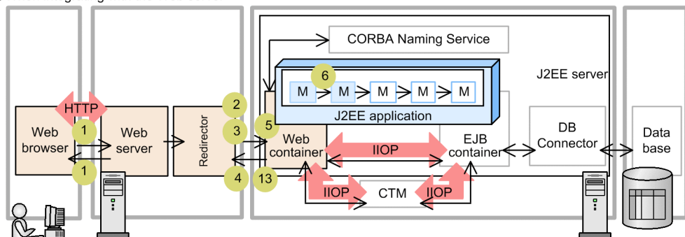
Figure 8-11: The timeout points (points 1 to 6 and 13) to be considered in the case of a Web front-end system
