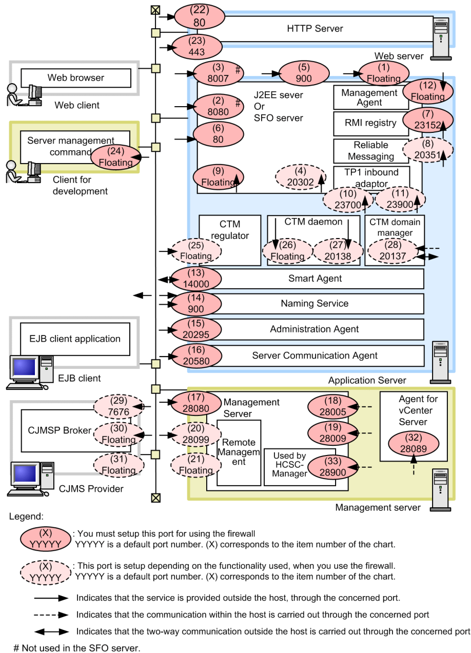
Figure 3-69: TCP/UDP port numbers used by Application Server
