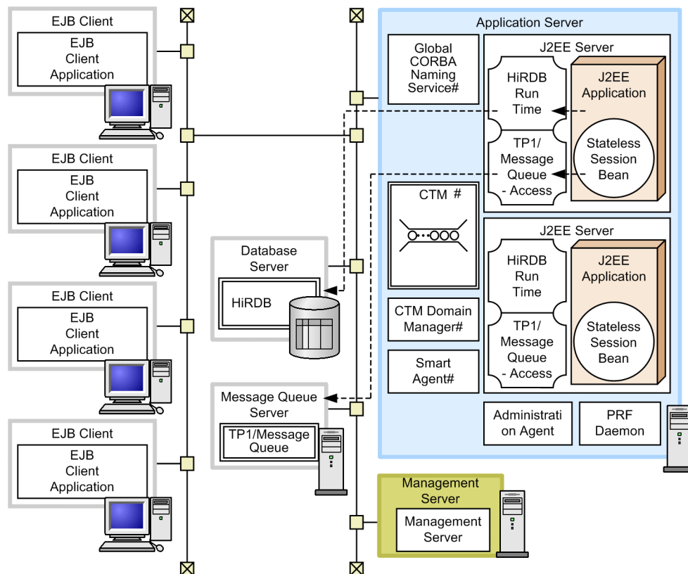
Figure 3-35: Example configuration when using a global transaction
