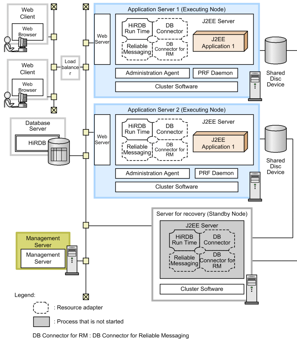
Figure 3-58: Example of system configuration of N-to-1 recovery system (when configuration of J2EE applications and resource adapters is same for N executing node machines)
