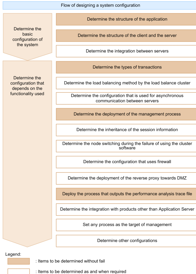
Figure 3-2: Flow for designing the system configuration (for a J2EE application execution platform)
