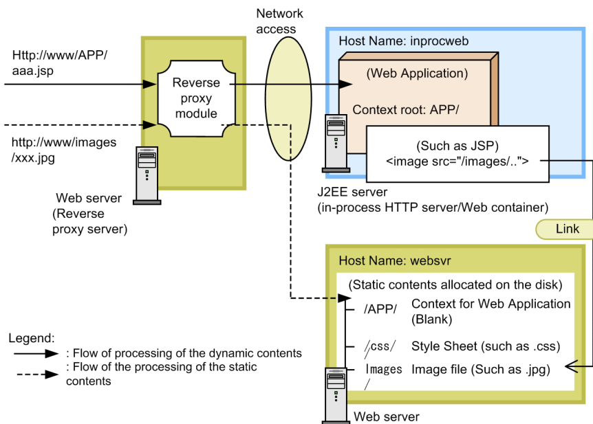
Figure 8-20: Deploying the static contents on the Web server (to use an in-process HTTP server)
