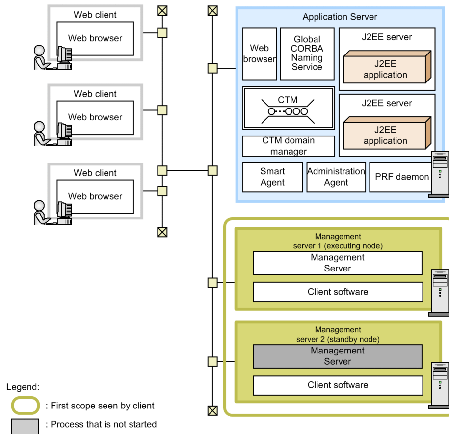
Figure 3-56: Example of the system configuration in which the executing node and the standby node of the management server are set to 1-to-1 ratio using cluster software
