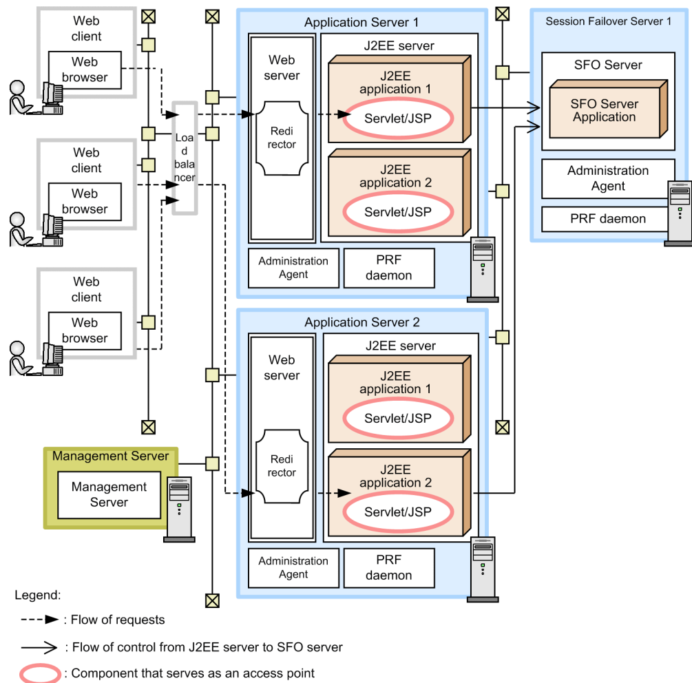
Figure 3-52: Example configuration when only a single SFO server exists in a system (when a session failover server is deployed)
