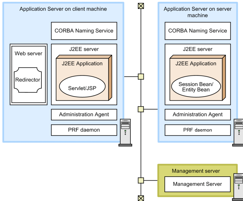
Figure 3-68: Example configuration with CORBA Naming Service invoked as out-process
