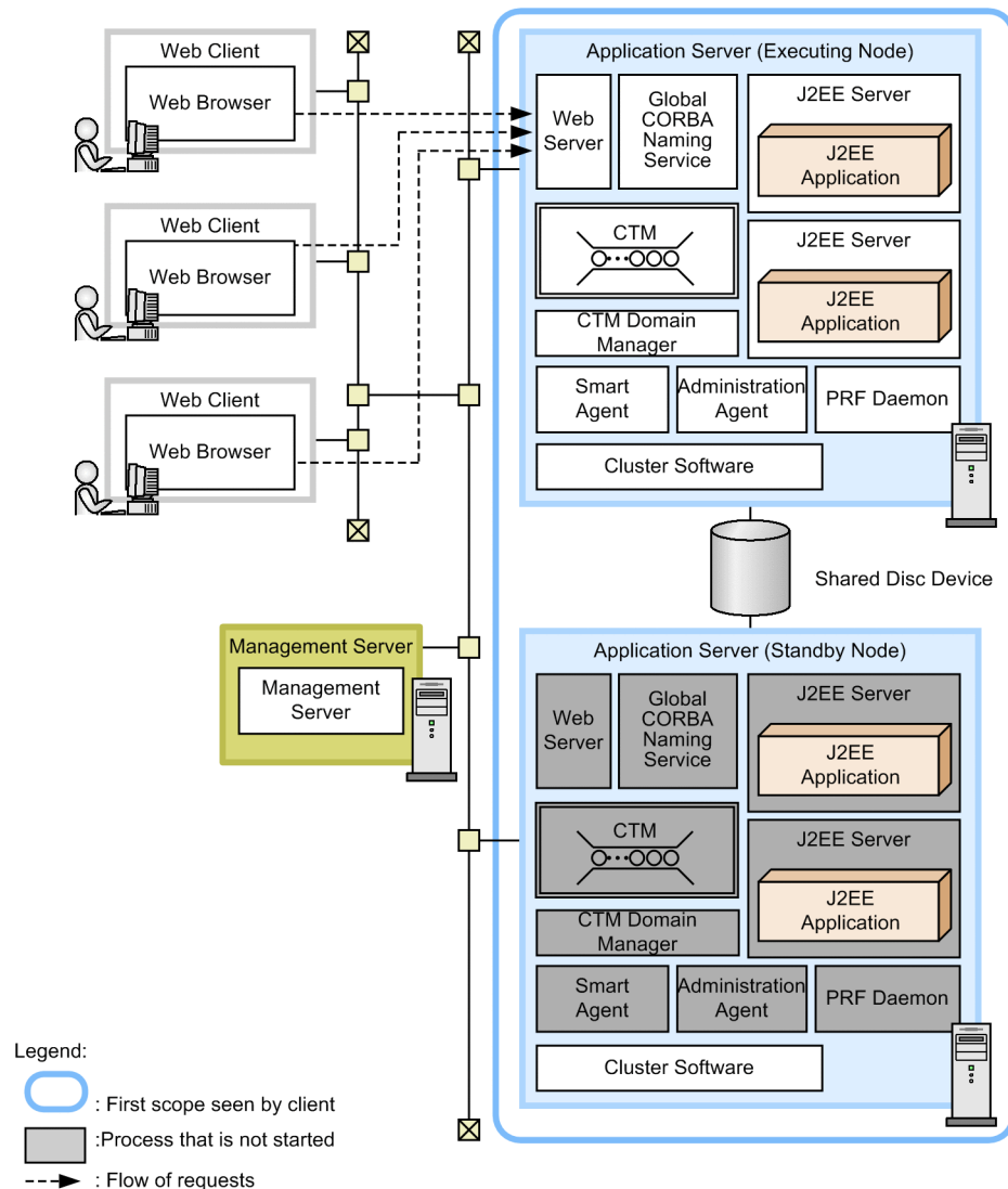
Figure 3-55: Example of system configuration where executing node and standby node of Application Server are in 1-to-1 ratio and cluster software is used (when transaction service is used)
