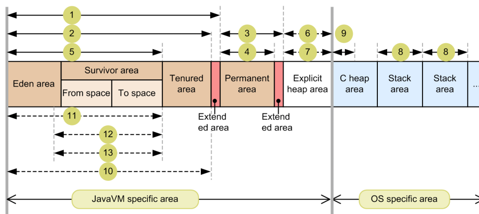
Figure 7-7: Configuration of memory space used by JavaVM
