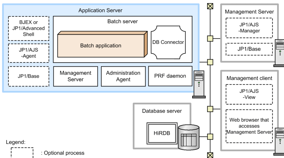
Figure 4-3: Example of the system configuration for deploying a batch server
