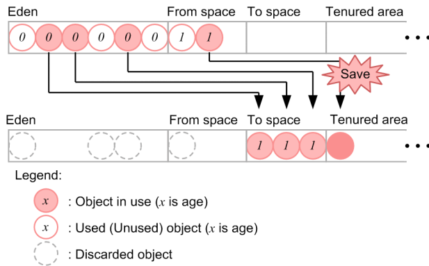
Figure 7-5: Saving objects
