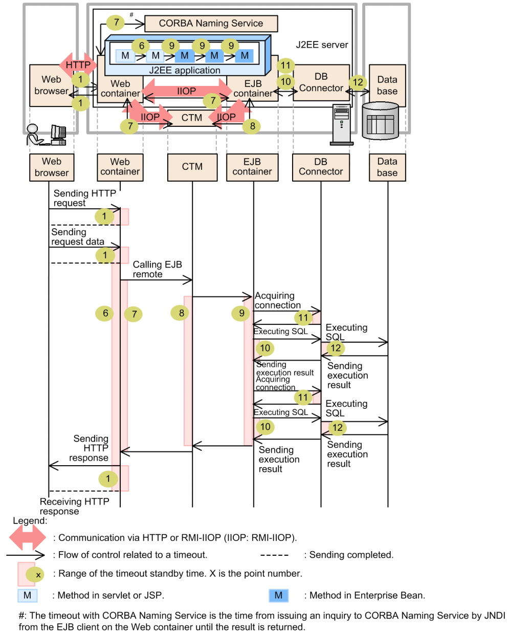
Figure 8-10: Points where timeouts can be set up (for in-process HTTP servers)
