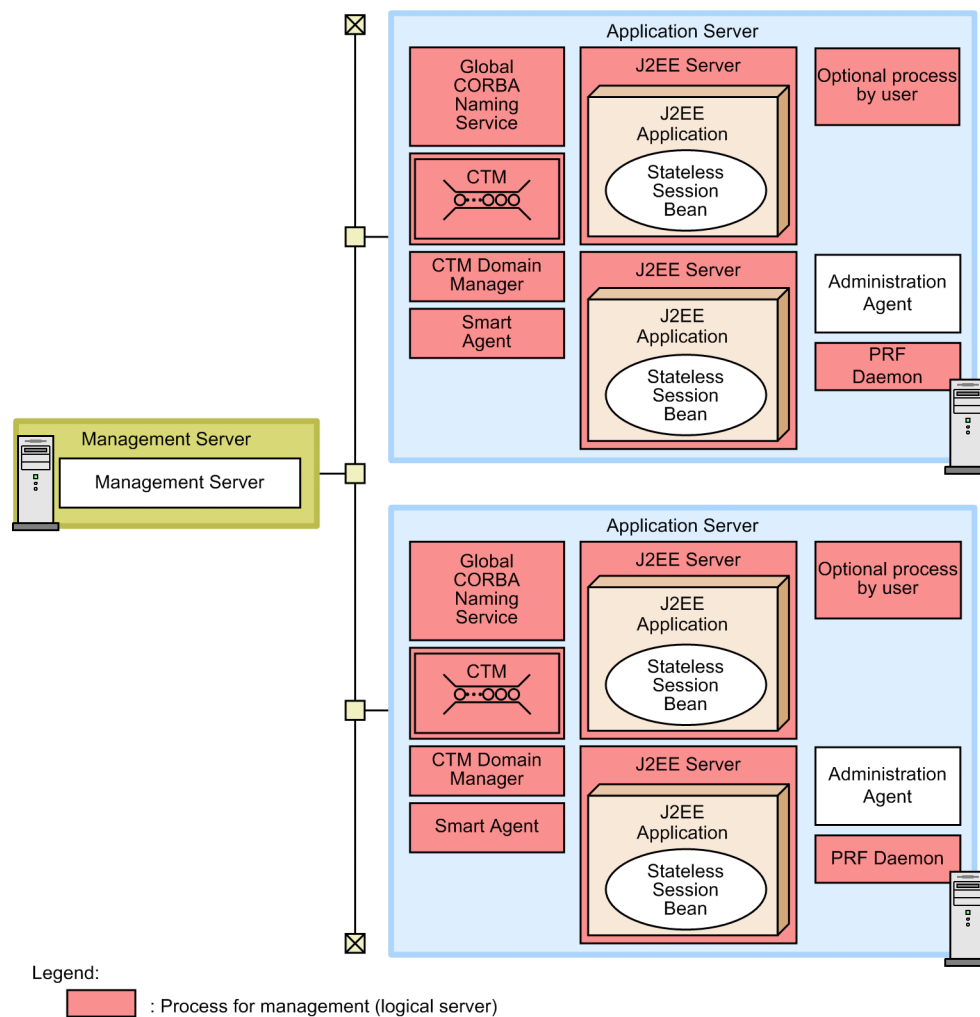
Figure 3-65: Example of a configuration with a user server deployed
