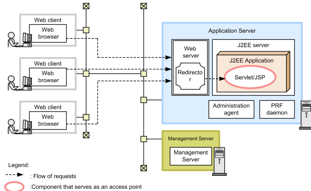
Figure 3-28: Example of a web client configuration built with one Application Server machine (in the case of Web server integration)
