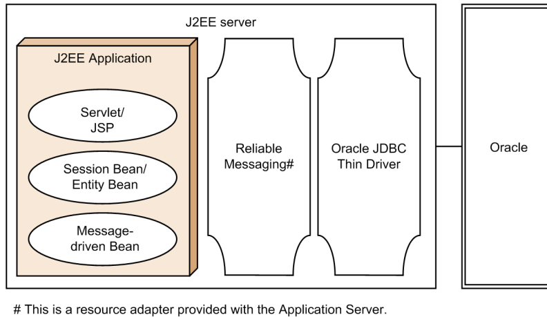
Figure 3-23: Configuration for accessing Oracle with Cosminexus RM
