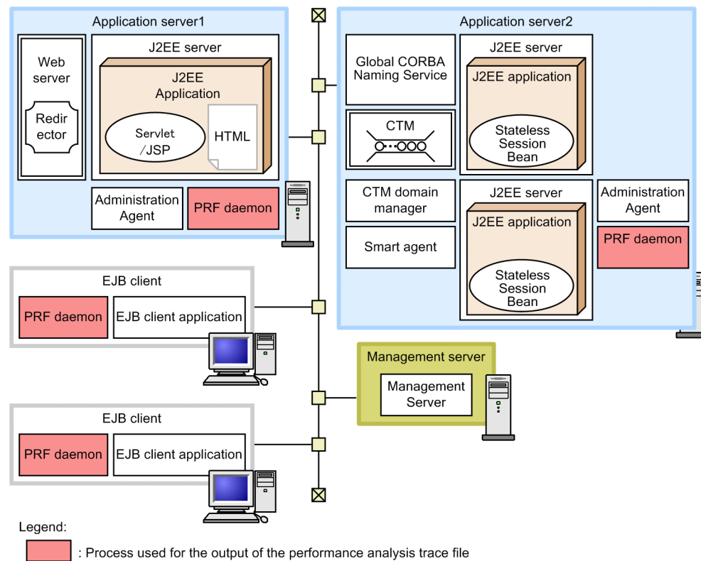
Figure 3-62: Example of deploying the PRF daemon
