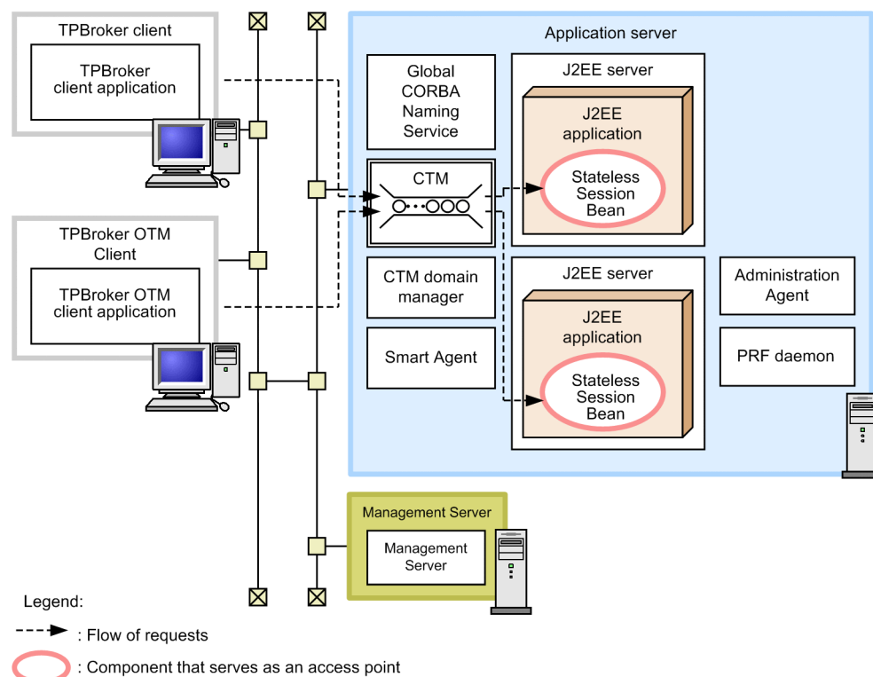
Figure 3-64: Example of configuration that invokes J2EE application through CTM from TPBroker client or TPBroker OTM client
