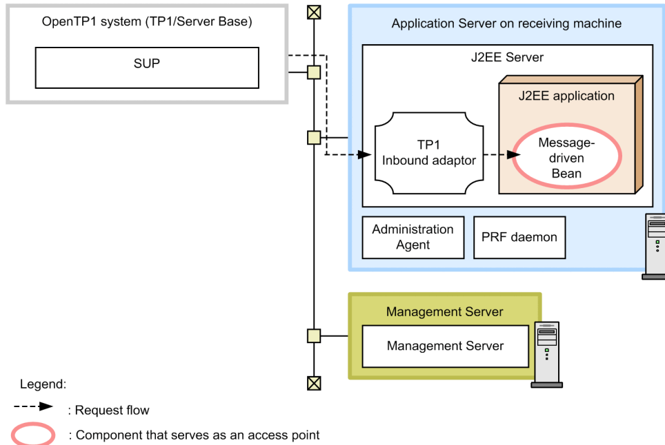
Figure 3-63: Example of message driven system configuration (when using the TP1 inbound integrated function)
