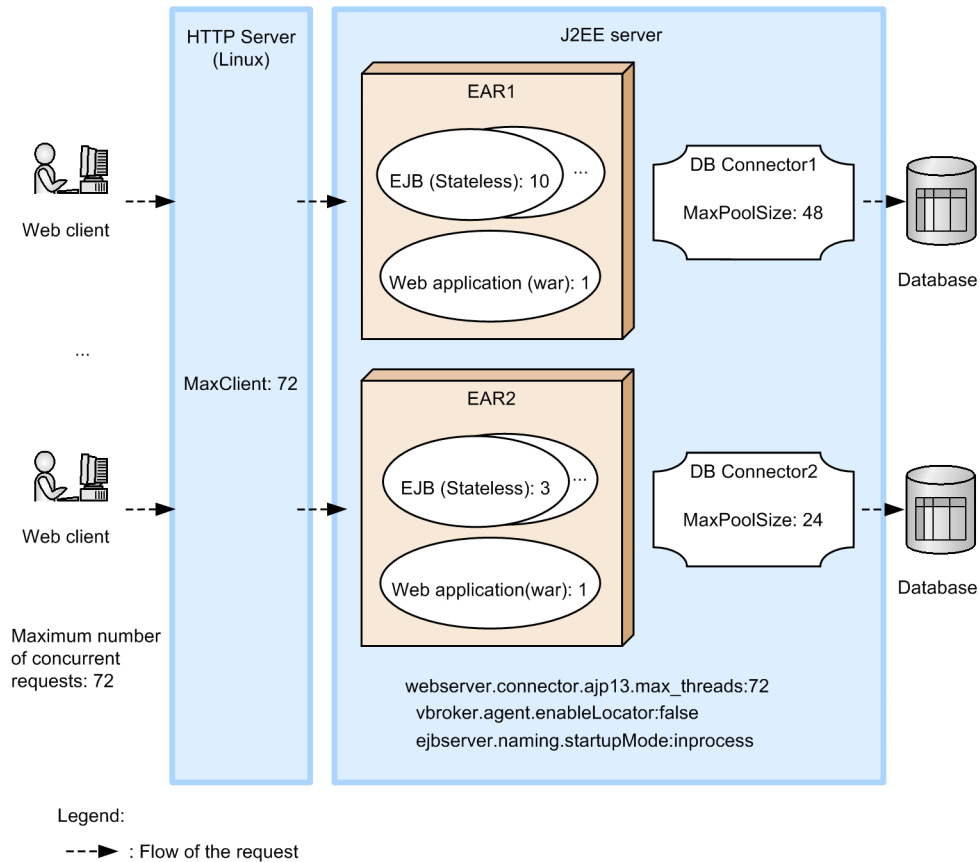
Figure 5-1: Example estimation of the number of threads when Cosminexus HTTP Server is used
