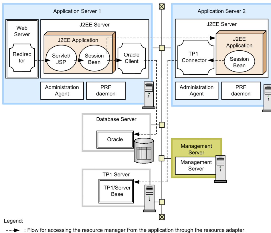
Figure 3-36: Example configuration when using transaction context propagation
