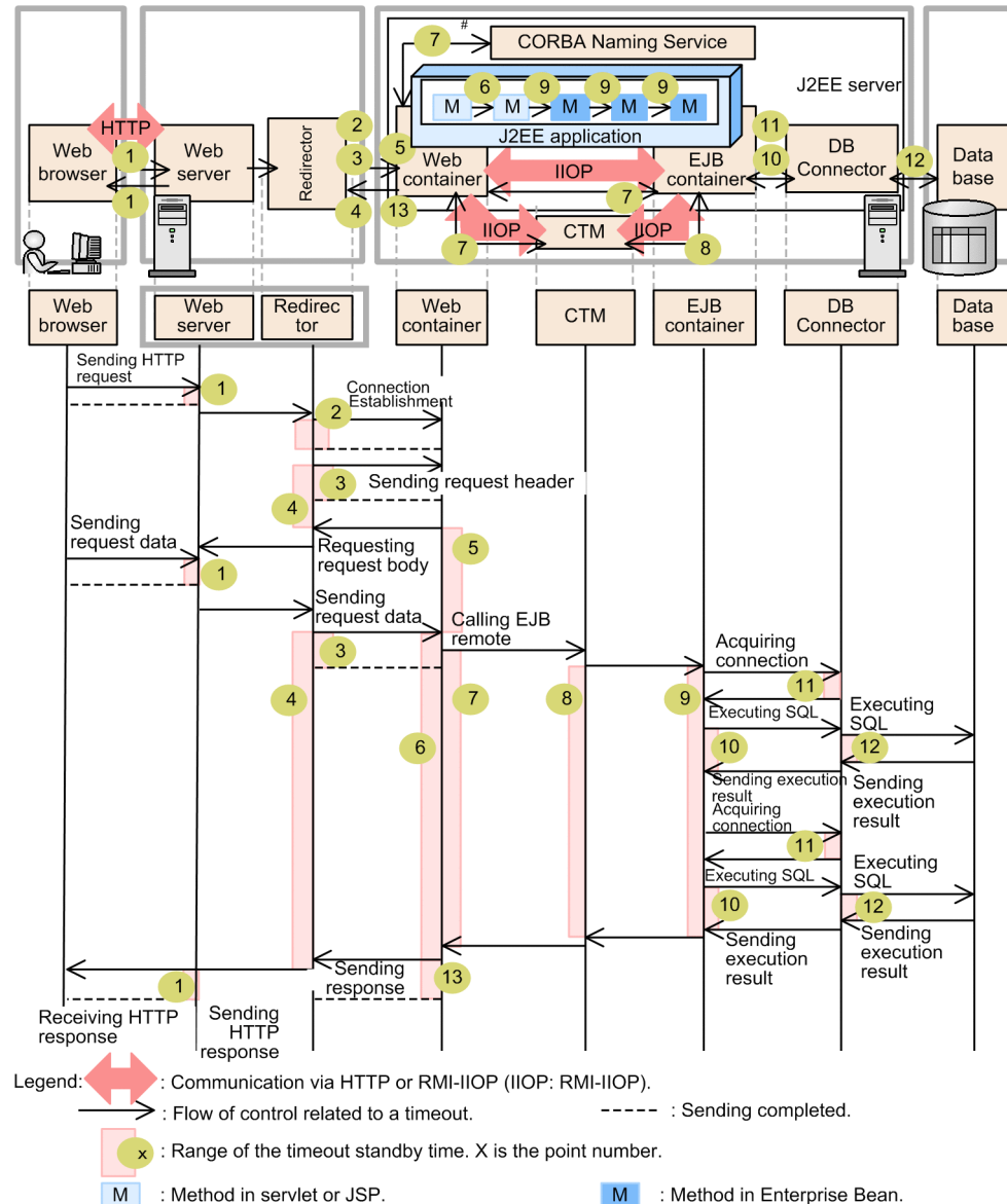
Figure 8-9: Points where a timeout can be set (for Web server integration)
