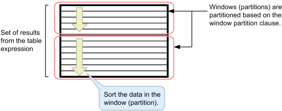
Figure 7-5: Functional overview of the window order clause
