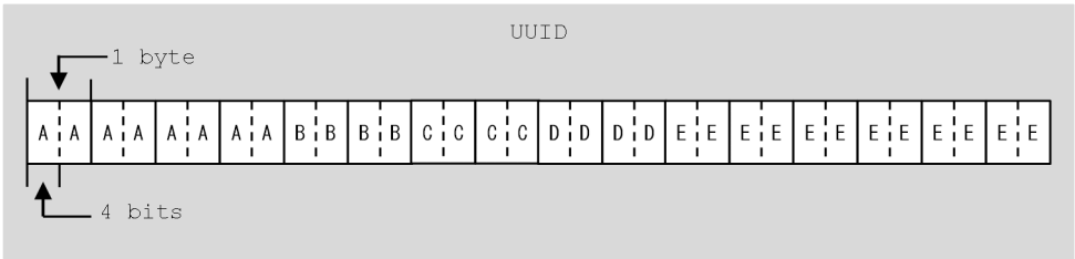
Figure 6-12: Data format of UUID type
