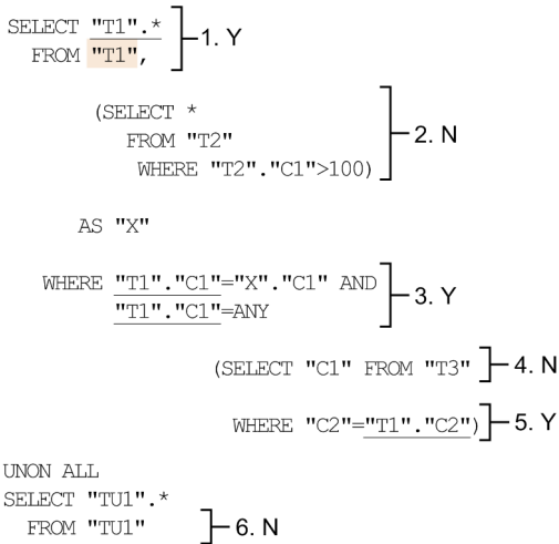
Figure 6-13: Example of the effective scope of scope variable T1 specified in a FROM clause (1 of 2)
