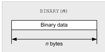
Figure 6-10: Data format of BINARY type
