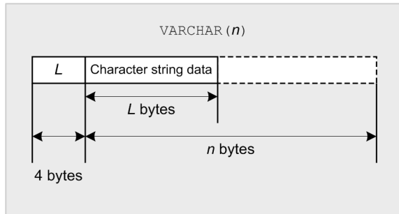
Figure 6-6: Data format of VARCHAR type
